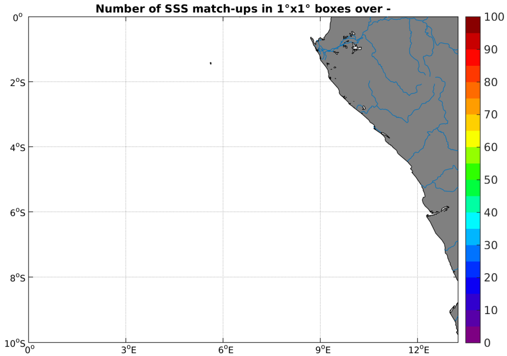
Figure 4: Number of SSS match-ups between TSG-GOSUD-Sailing-ship SSS and the SMOS-L4-CATDS-CECOS-IFREMER-V2-WEEKLY-0.5DEG SSS product for the Congo river plume Pi-MEP region over 1°x1° boxes and for the full satellite product period.
