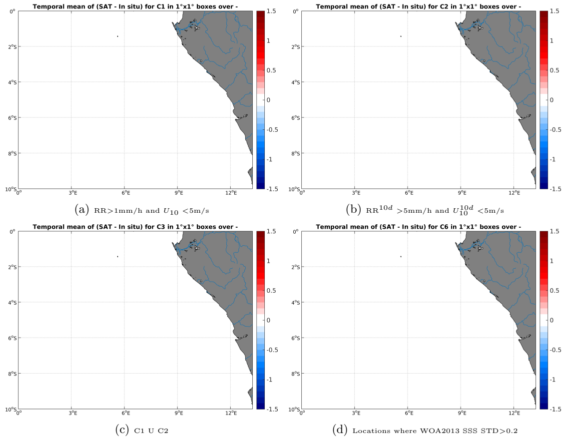
Figure 12: Temporal mean gridded over spatial boxes of size 1^\circ \times 1^\circ of \Delta SSS (SMOS-L4-CATDS-CECOS-IFREMER-V2-WEEKLY-0.5DEG - TSG-GOSUD-Sailing-ship) for 4 different subdatasets corresponding to:RR > 1 mm/h and U_{10} < 5 m/s (a), RR 10d > 5 mm/h and U_{10}^{10d} < 5 m/s (b), C1 U C2 (c),Locations where WOA2013 SSS STD > 0.2 (d).
