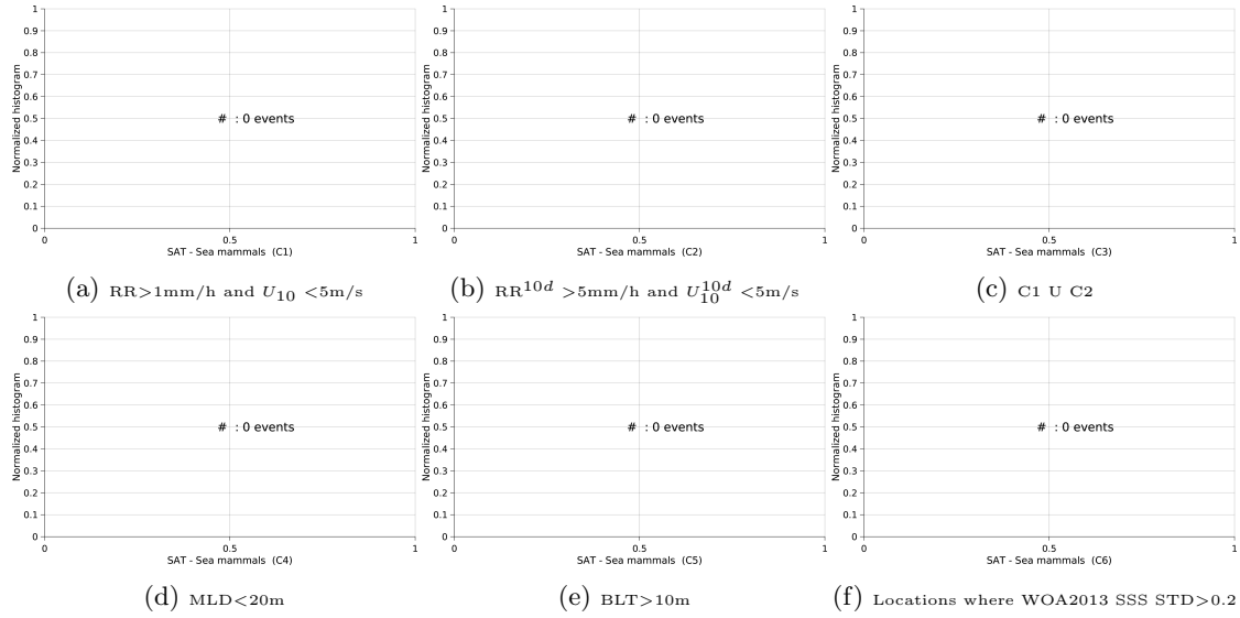
Figure 13: Normalized histogram of \Delta\text{SSS} (SMOS-L4-CATDS-CECOS-IFREMER-V2-WEEKLY-0.5DEG - Sea mammals) for 6 different subdatasets corresponding to: RR > 1\text{mm/h} and U_{10} < 5\text{m/s} (a), RR^{10d} > 5\text{mm/h} and U_{10}^{10d} < 5\text{m/s} (b), C1 U C2 (c), MLD < 20\text{m} (d), BLT > 10\text{m} (e), Locations where WOA2013 SSS STD > 0.2 (f).
