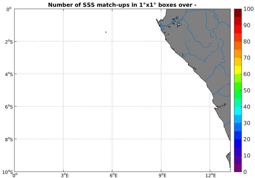
Figure 3: Number of SSS match-ups between Surface drifters SSS and the SMOS-L4-CATDS-CECOS-IFREMER-V2-WEEKLY-0.5DEG SSS product for the Congo river plume Pi-MEP region over 1^\circ \times 1^\circ boxes and for the full satellite product period.
