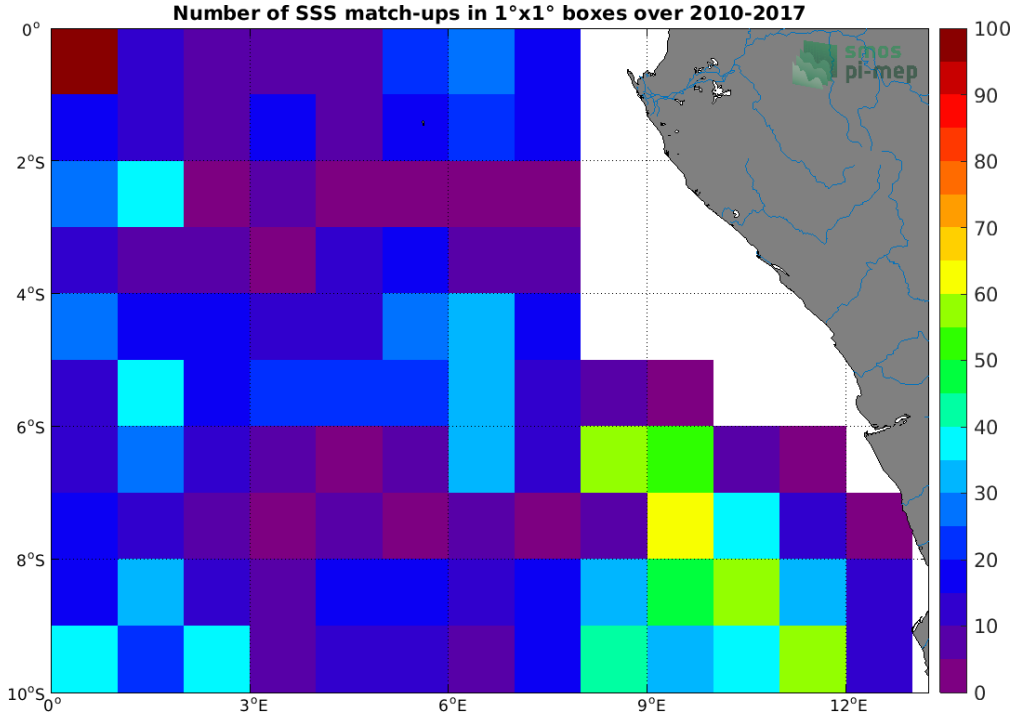
Figure 4: Number of SSS match-ups between Argo SSS and the SMOS L4 v2 Weekly (CATDS-CECOS-IFREMER) SSS product for the Congo river plume Pi-MEP region over 1°x1° boxes and for the full satellite product period.
