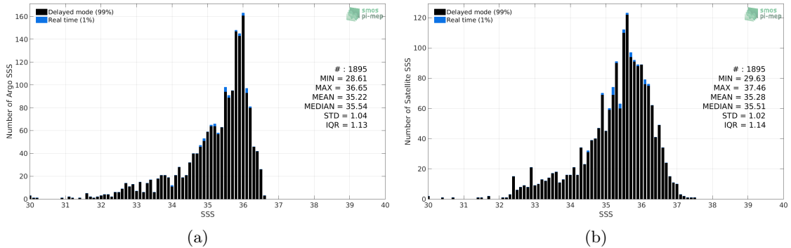
Figure 2: Histograms of SSS from Argos (a) and SMOS-L4-CATDS-CECOS-IFREMER-V2-WEEKLY-0.5DEG (b) considering all match-up pairs per bins of 0.1 over the Congo river plume Pi-MEP region and for the full satellite product period.
