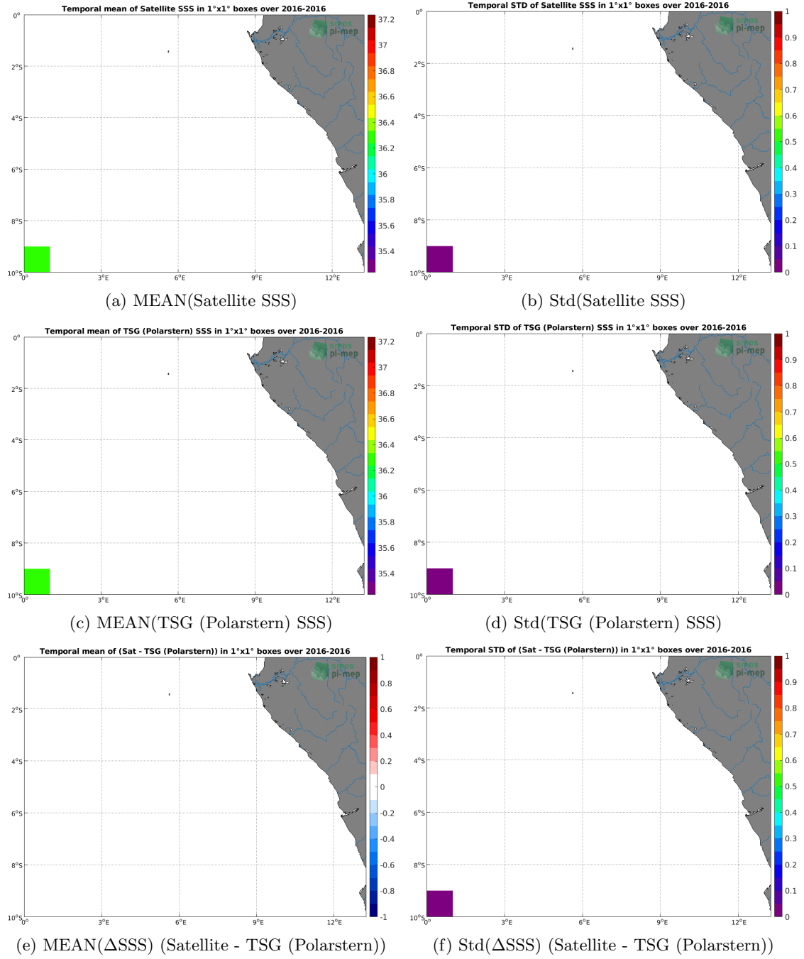
Figure 6: Temporal mean (left) and Std (right) of SSS from SMOS SSS L3 v3 Monthly (ICDC) (top), TSG (Polarstern) (middle), and of \Delta SSS (Satellite - TSG (Polarstern)). Only match-up pairs are used to generate these maps.
