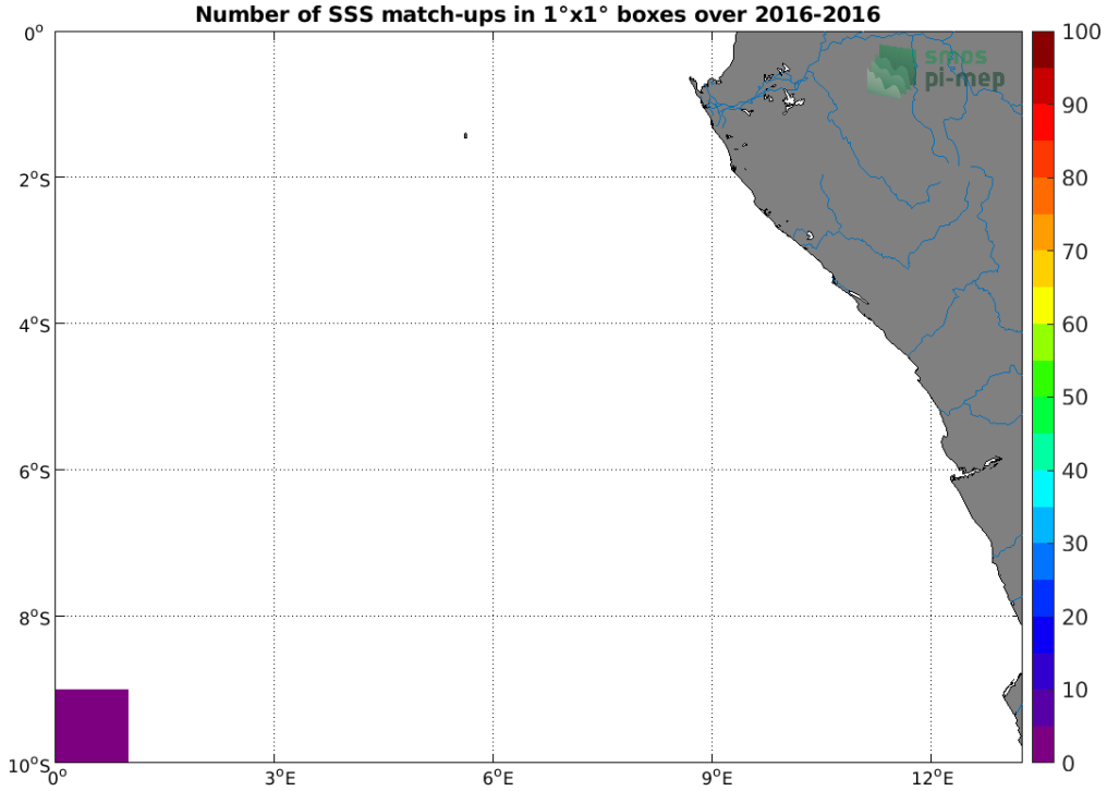
Figure 4: Number of SSS match-ups between TSG (Polarstern) SSS and the SMOS SSS L3 v3 Monthly (ICDC) SSS product for the Congo river plume Pi-MEP region over 1^\circ \times 1^\circ boxes and for the full satellite product period.
