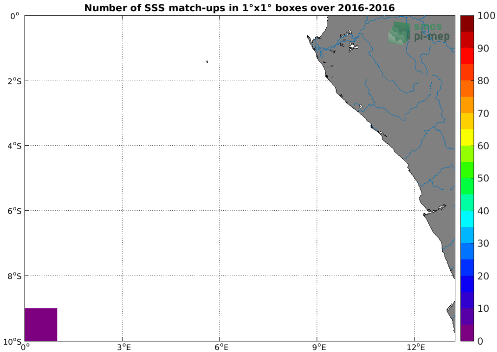
Figure 4: Number of SSS match-ups between TSG (Polarstern) SSS and the SMOS SSS L3 v3 Monthly (ICDC) SSS product for the Congo river plume Pi-MEP region over 1°x1° boxes and for the full satellite product period.
