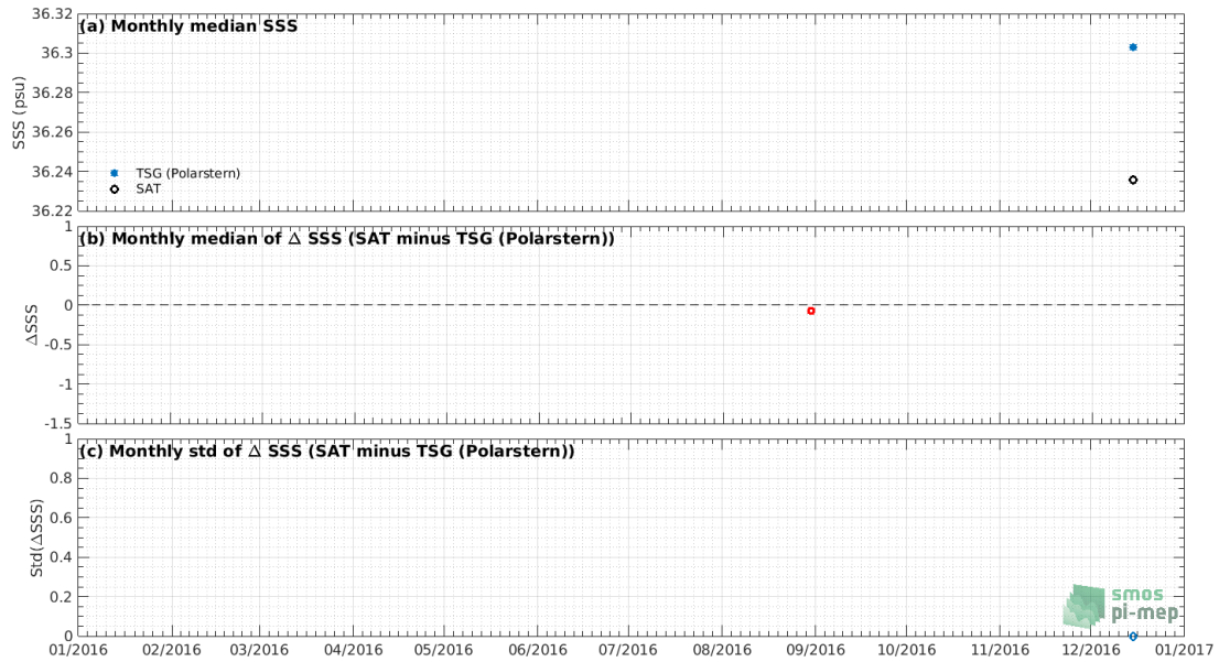
Figure 7: Time series of the monthly median SSS (top), median of \Delta SSS (Satellite - TSG (Polarstern)) and Std of \Delta SSS (Satellite - TSG (Polarstern)) over the Congo river plume Pi-MEP region considering all match-ups collected by the Pi-MEP.
