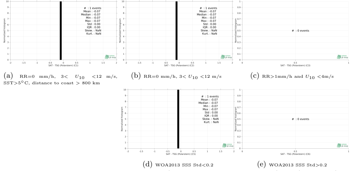
Figure 13: Normalized histogram of \Delta\text{SSS} (SMOS SSS L3 v3 Monthly (ICDC) - TSG (Polarstern)) for 5 different subdatasets corresponding to: RR=0 mm/h, 3 < U_{10} < 12 m/s, SST > 5^\circ\text{C} , distance to coast > 800 km (a), RR=0 mm/h, 3 < U_{10} < 12 m/s (b), RR > 1\text{mm/h} and U_{10} < 4\text{m/s} (c), WOA2013 SSS Std < 0.2 (d), WOA2013 SSS Std > 0.2 (e).
