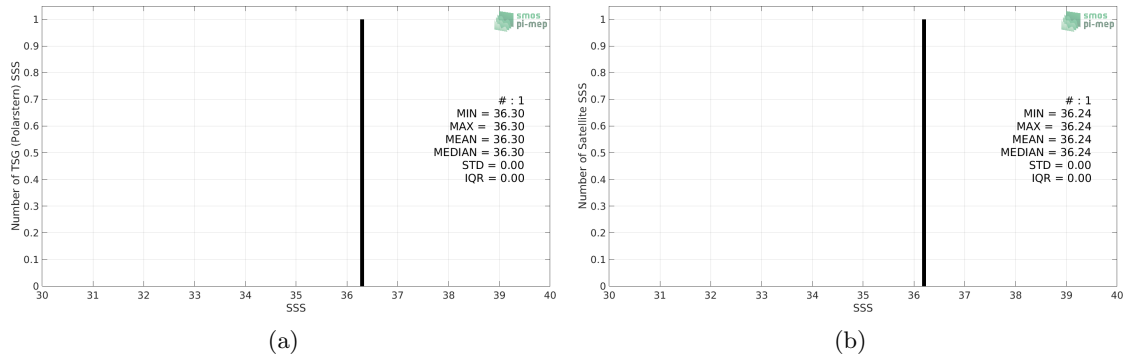
Figure 2: Histograms of SSS from TSG (Polarstern) (a) and SMOS SSS L3 v3 Monthly (ICDC) (b) considering all match-up pairs per bins of 0.1 over the Congo river plume Pi-MEP region and for the full satellite product period.
