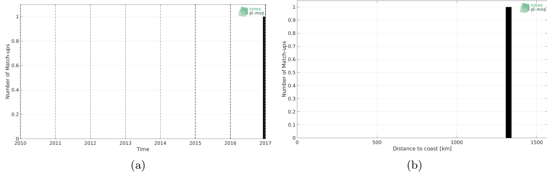
Figure 1: Number of match-ups between TSG (Polarstern) and SMOS SSS L3 v3 Monthly (ICDC) SSS as a function of time (a) and as function of the distance to coast (b) over the Congo river plume Pi-MEP region and for the full satellite product period.
