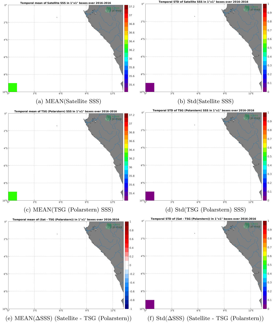
Figure 6: Temporal mean (left) and Std (right) of SSS from SMOS SSS L3 v3 Monthly (ICDC) (top), TSG (Polarstern) (middle), and of \Delta SSS (Satellite - TSG (Polarstern)). Only match-up pairs are used to generate these maps.
