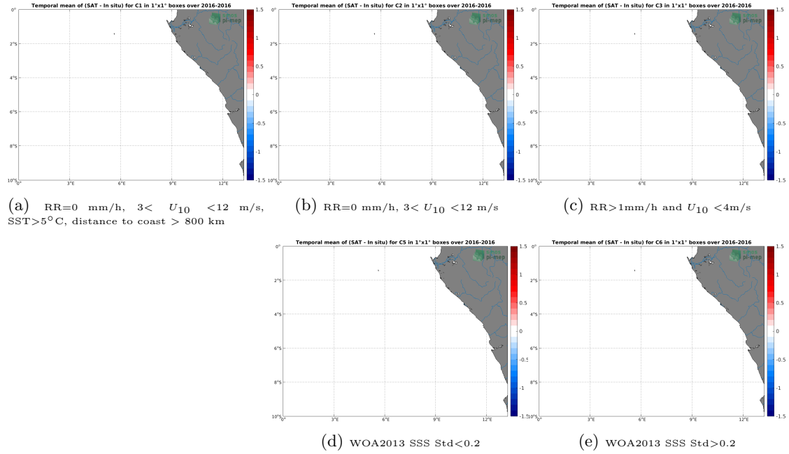
Figure 12: Temporal mean gridded over spatial boxes of size 1^{\circ}\times 1^{\circ} of \Delta\text{SSS} (SMOS SSS L3 v3 Monthly (ICDC) - TSG (Polarstern)) for 5 different subdatasets corresponding to:RR=0 mm/h, 3 < U_{10} < 12 m/s, SST >5^{\circ}\text{C} , distance to coast > 800 km (a), RR=0 mm/h, 3 < U_{10} < 12 m/s (b), RR >1 mm/h and U_{10} < 4 m/s (c), WOA2013 SSS Std <0.2 (d), WOA2013 SSS Std >0.2 (e).
