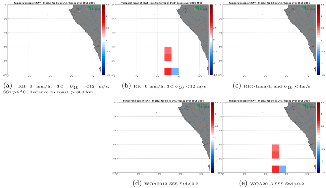
Figure 12: Temporal mean gridded over spatial boxes of size 1^\circ \times 1^\circ of \Delta SSS (SMOS SSS L3 v3 Monthly (ICDC) - TSG (LEGOS-DM)) for 5 different subdatasets corresponding to: RR=0 mm/h, 3 < U_{10} < 12 m/s, SST >5^\circ\text{C} , distance to coast > 800 km (a), RR=0 mm/h, 3 < U_{10} < 12 m/s (b), RR >1 mm/h and U_{10} < 4 m/s (c), WOA2013 SSS Std <0.2 (d), WOA2013 SSS Std >0.2 (e).
