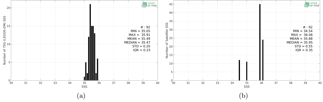
Figure 2: Histograms of SSS from TSG (LEGOS-DM) (a) and SMOS SSS L3 v3 Monthly (ICDC) (b) considering all match-up pairs per bins of 0.1 over the Congo river plume Pi-MEP region and for the full satellite product period.
