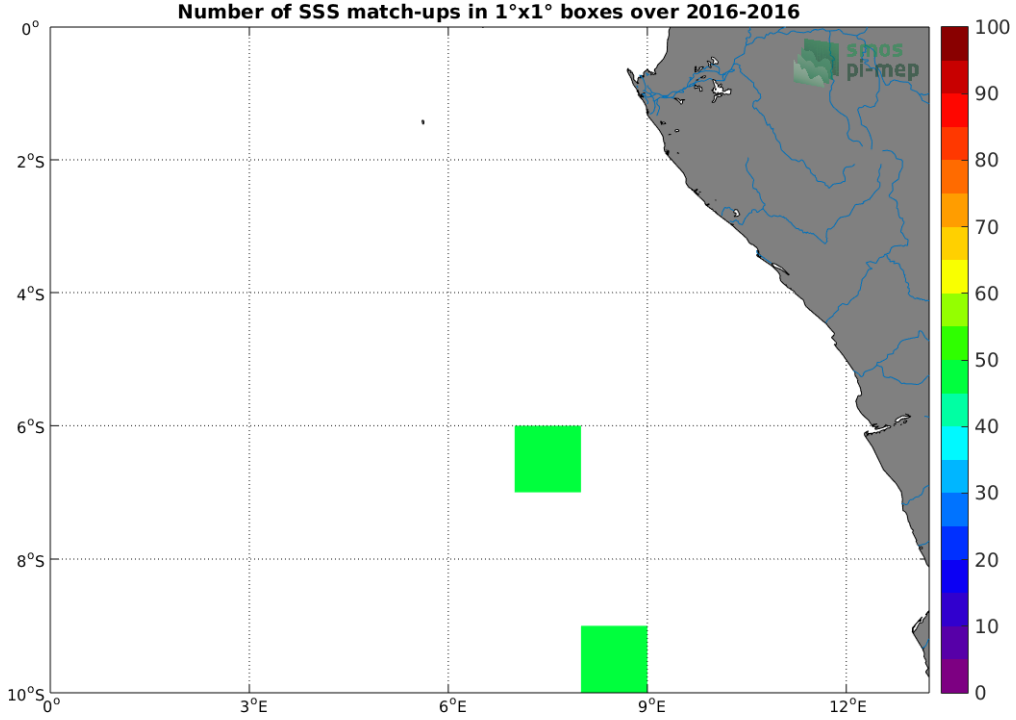
Figure 4: Number of SSS match-ups between TSG (LEGOS-DM) SSS and the SMOS SSS L3 v3 Monthly (ICDC) SSS product for the Congo river plume Pi-MEP region over 1^\circ \times 1^\circ boxes and for the full satellite product period.
