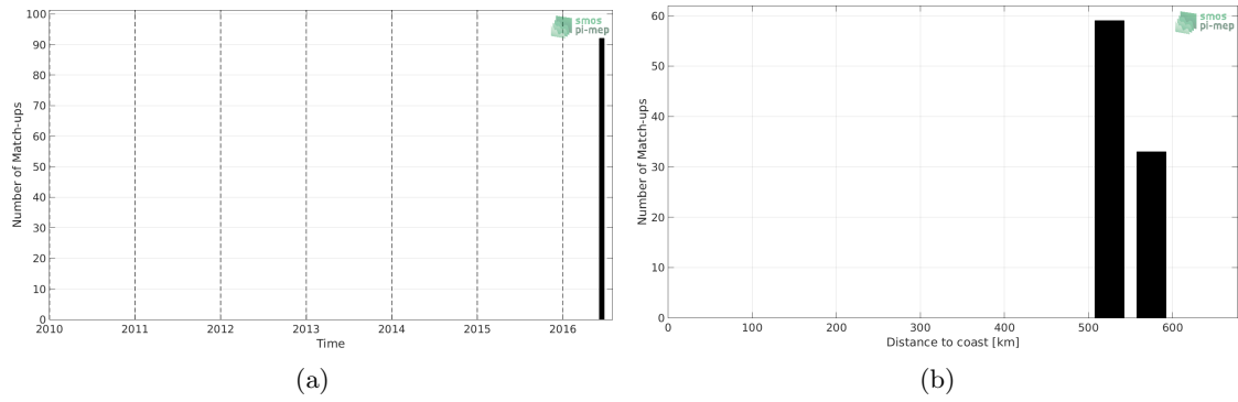
Figure 1: Number of match-ups between TSG (LEGOS-DM) and SMOS SSS L3 v3 Monthly (ICDC) SSS as a function of time (a) and as function of the distance to coast (b) over the Congo river plume Pi-MEP region and for the full satellite product period.
