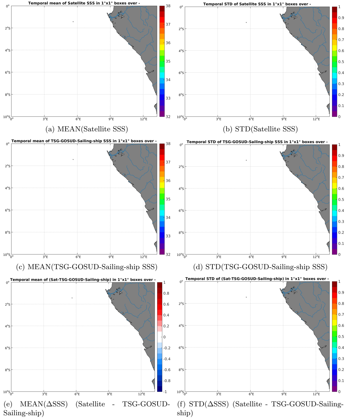
Figure 6: Temporal mean (left) and STD (right) of SSS from SMOS-L3-ICDC-V3-MONTHLY-0.5DEG (top), TSG-GOSUD-Sailing-ship (middle), and of \Delta SSS (Satellite - TSG-GOSUD-Sailing-ship). Only match-up pairs are used to generate these maps.
