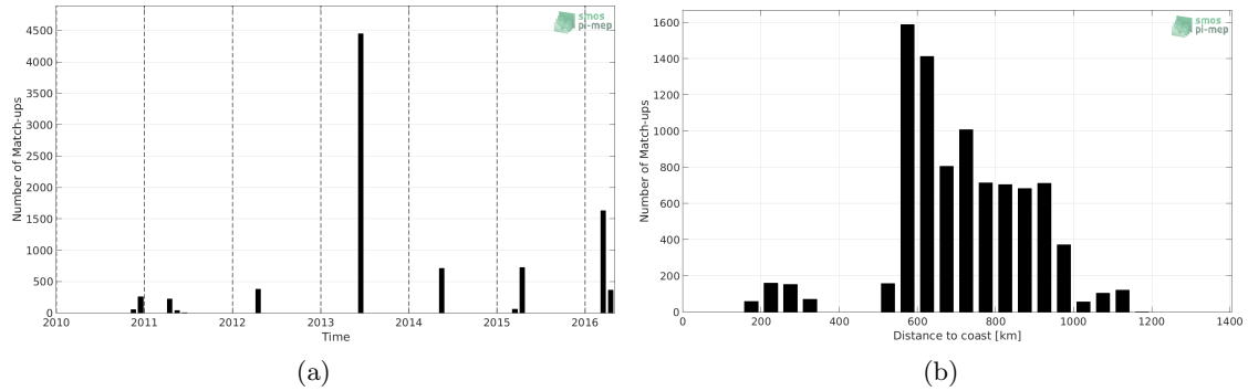
Figure 1: Number of match-ups between TSG (GOSUD-Research-vessel) and SMOS SSS L3 v3 Monthly (ICDC) SSS as a function of time (a) and as function of the distance to coast (b) over the Congo river plume Pi-MEP region and for the full satellite product period.
