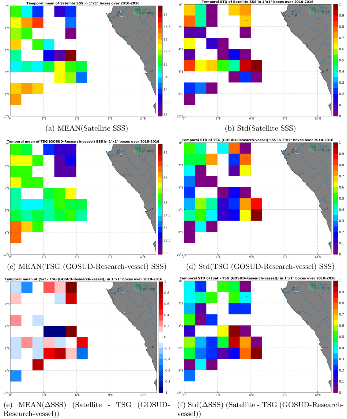
Figure 6: Temporal mean (left) and Std (right) of SSS from SMOS SSS L3 v3 Monthly (ICDC) (top), TSG (GOSUD-Research-vessel) (middle), and of \Delta SSS (Satellite - TSG (GOSUD-Research-vessel)). Only match-up pairs are used to generate these maps.
