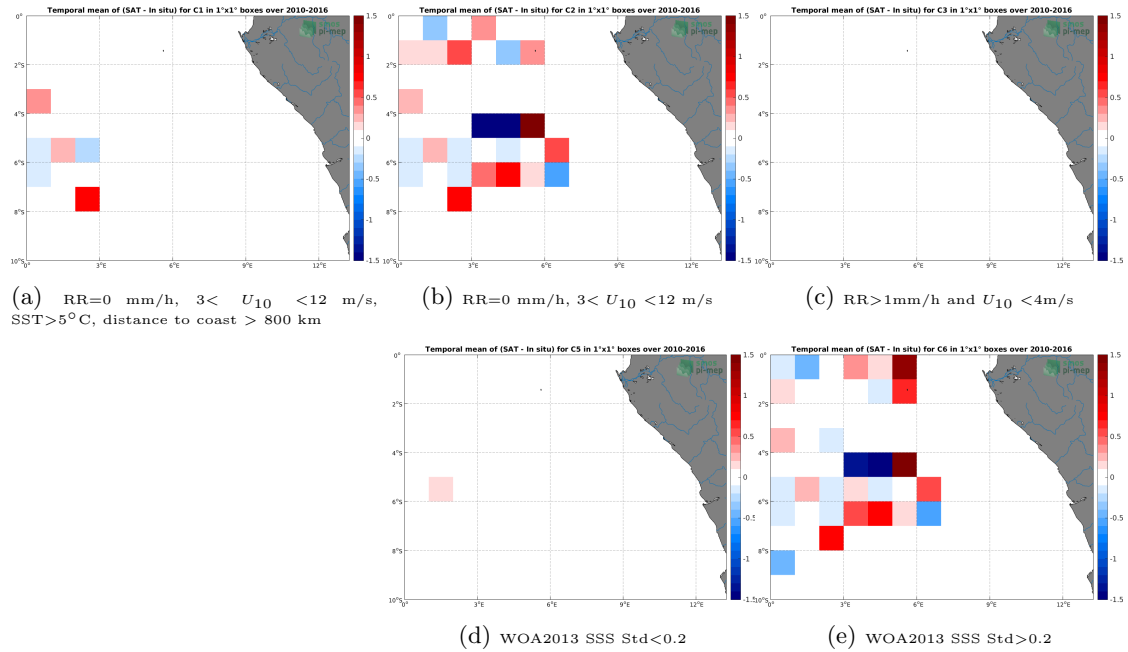
Figure 12: Temporal mean gridded over spatial boxes of size 1^\circ \times 1^\circ of \Delta SSS (SMOS SSS L3 v3 Monthly (ICDC) - TSG (GOSUD-Research-vessel)) for 5 different subdatasets corresponding to: RR=0 mm/h, 3 < U_{10} < 12 m/s, SST >5^\circ\text{C} , distance to coast > 800 km (a), RR=0 mm/h, 3 < U_{10} < 12 m/s (b), RR >1 mm/h and U_{10} < 4 m/s (c), WOA2013 SSS Std <0.2 (d), WOA2013 SSS Std >0.2 (e).
