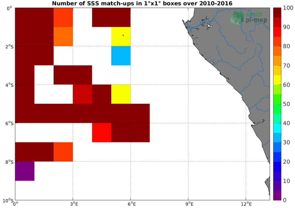
Figure 4: Number of SSS match-ups between TSG (GOSUD-Research-vessel) SSS and the SMOS SSS L3 v3 Monthly (ICDC) SSS product for the Congo river plume Pi-MEP region over 1^\circ \times 1^\circ boxes and for the full satellite product period.
