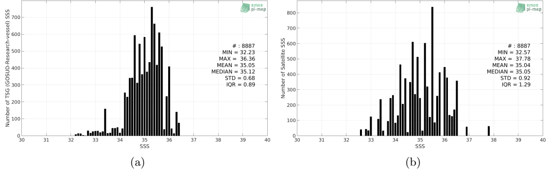
Figure 2: Histograms of SSS from TSG (GOSUD-Research-vessel) (a) and SMOS SSS L3 v3 Monthly (ICDC) (b) considering all match-up pairs per bins of 0.1 over the Congo river plume Pi-MEP region and for the full satellite product period.
