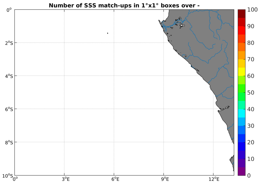
Figure 4: Number of SSS match-ups between Sea mammals SSS and the SMOS-L3-ICDC-V3-MONTHLY-0.5DEG SSS product for the Congo river plume Pi-MEP region over 1°x1° boxes and for the full satellite product period.
