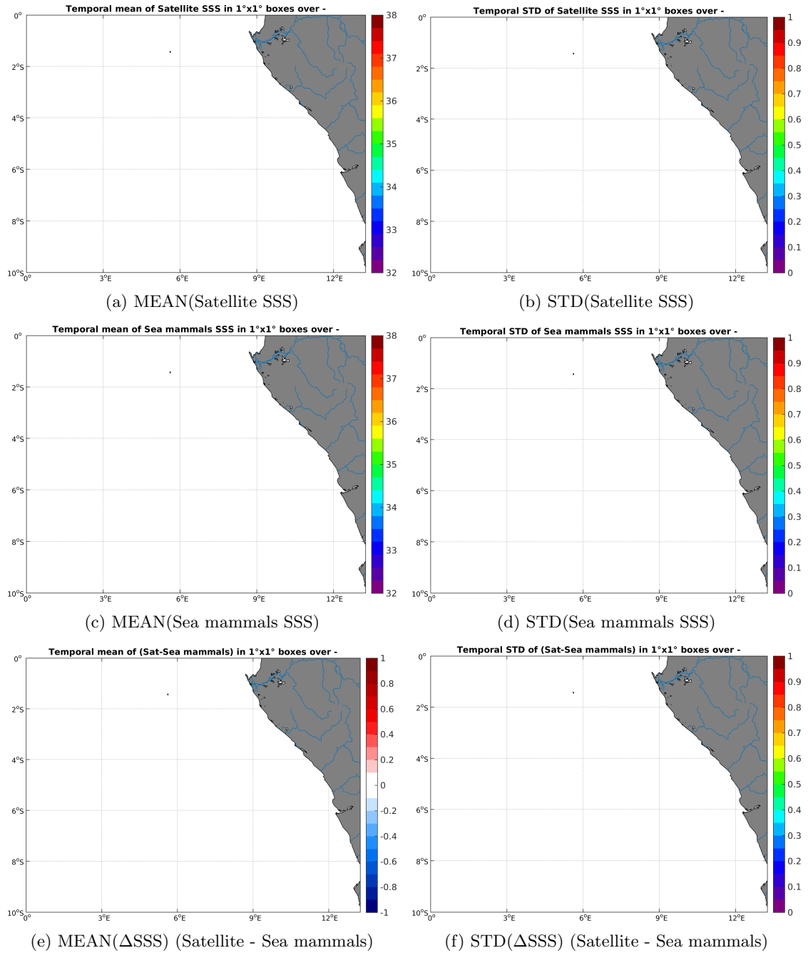
Figure 6: Temporal mean (left) and STD (right) of SSS from SMOS-L3-ICDC-V3-MONTHLY-0.5DEG (top), Sea mammals (middle), and of \Delta SSS (Satellite - Sea mammals). Only match-up pairs are used to generate these maps.
