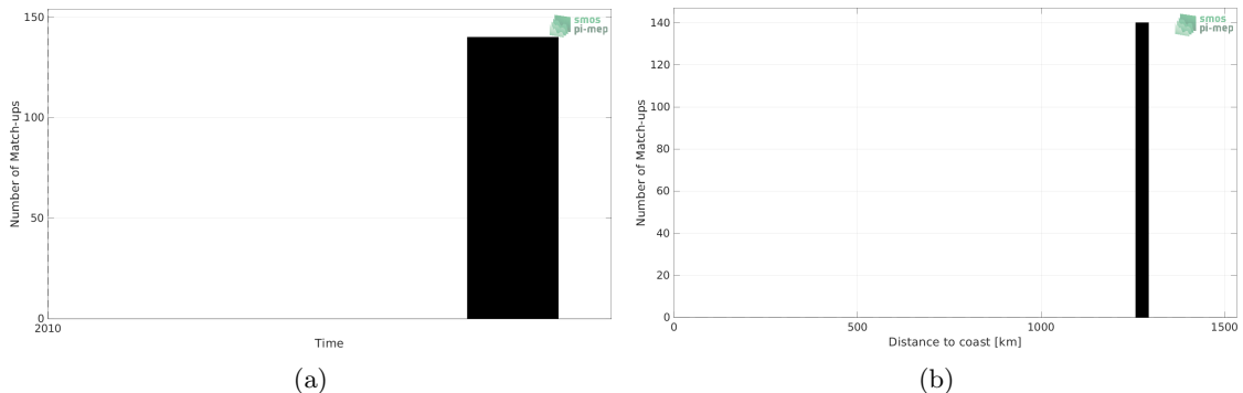
Figure 1: Number of match-ups between TSG (SAMOS) and SMOS SSS L2Q v331 - With FLAG (CMEMS-CATDS-CPDC) SSS as a function of time (a) and as function of the distance to coast (b) over the Congo river plume Pi-MEP region and for the full satellite product period.
