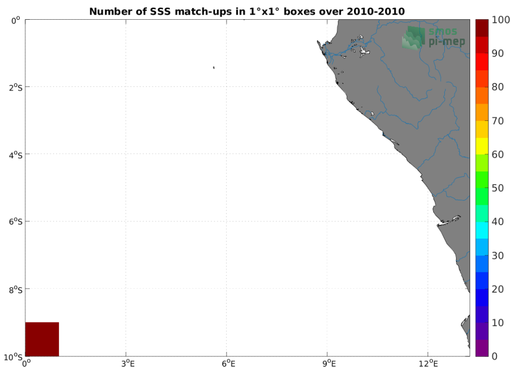
Figure 4: Number of SSS match-ups between TSG (SAMOS) SSS and the SMOS SSS L2Q v331 - With FLAG (CMEMS-CATDS-CPDC) SSS product for the Congo river plume Pi-MEP region over 1^\circ \times 1^\circ boxes and for the full satellite product period.
