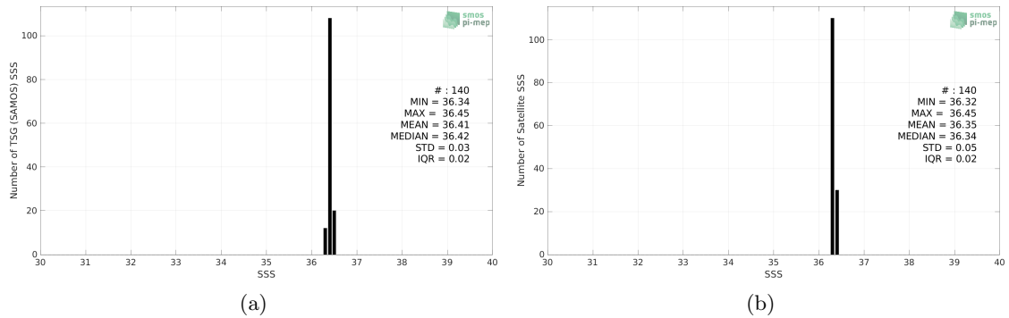
Figure 2: Histograms of SSS from TSG (SAMOS) (a) and SMOS SSS L2Q v331 - With FLAG (CMEMS-CATDS-CPDC) (b) considering all match-up pairs per bins of 0.1 over the Congo river plume Pi-MEP region and for the full satellite product period.
