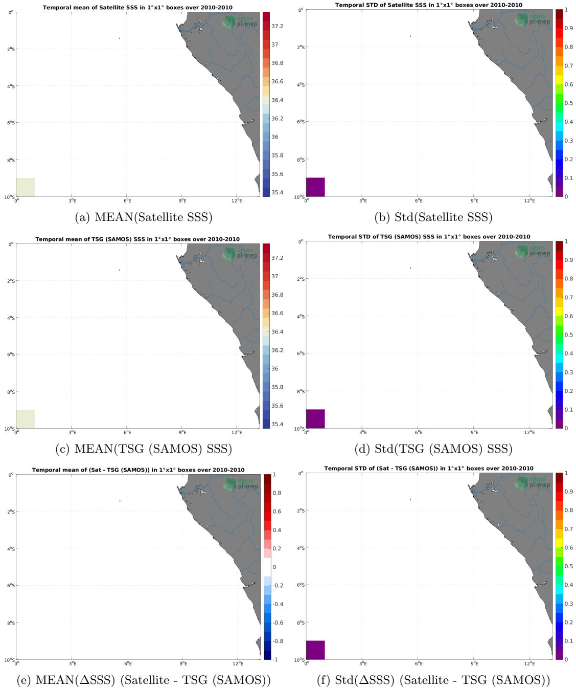
Figure 6: Temporal mean (left) and Std (right) of SSS from SMOS SSS L2Q v331 - With FLAG (CMEMS-CATDS-CPDC) (top), TSG (SAMOS) (middle), and of \Delta SSS (Satellite - TSG (SAMOS)). Only match-up pairs are used to generate these maps.
