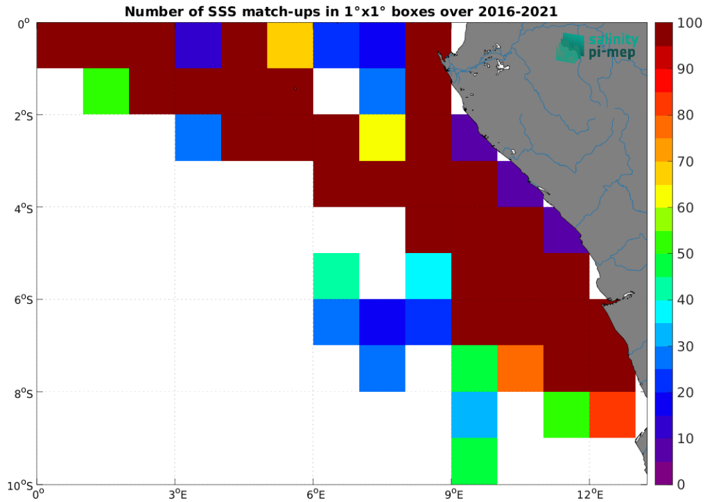
Figure 5: Number of SSS match-ups between TSG (LEGOS-DM) SSS and the SMOS SSS L2Q v331 - With FLAG (CMEMS-CATDS-CPDC) SSS product for the Congo river plume Pi-MEP region over 1^\circ \times 1^\circ boxes and for the full satellite product period.
