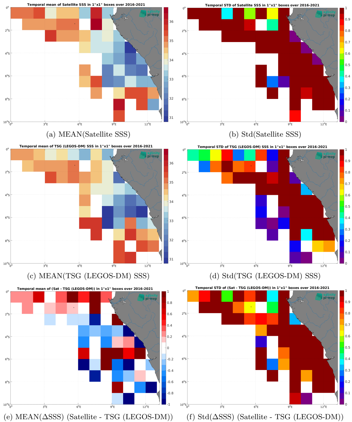
Figure 7: Temporal mean (left) and Std (right) of SSS from SMOS SSS L2Q v331 - With FLAG (CMEMS-CATDS-CPDC) (top), TSG (LEGOS-DM) (middle), and of \Delta SSS (Satellite - TSG (LEGOS-DM)). Only match-up pairs are used to generate these maps.
