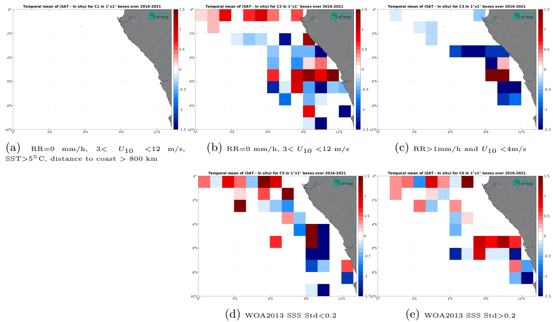
Figure 14: Temporal mean gridded over spatial boxes of size 1^\circ \times 1^\circ of \Delta SSS (SMOS SSS L2Q v331 - With FLAG (CMEMS-CATDS-CPDC) - TSG (LEGOS-DM)) for 5 different subdatasets corresponding to:RR=0 mm/h, 3 < U_{10} < 12 m/s, SST >5^\circ C, distance to coast > 800 km (a), RR=0 mm/h, 3 < U_{10} < 12 m/s (b), RR >1 mm/h and U_{10} < 4 m/s (c), WOA2013 SSS Std <0.2 (d), WOA2013 SSS Std >0.2 (e).
