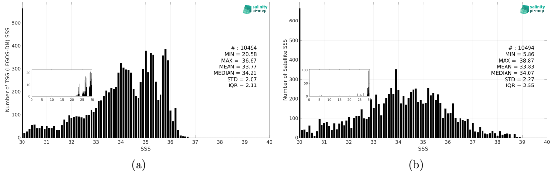
Figure 3: Histograms of SSS from TSG (LEGOS-DM) (a) and SMOS SSS L2Q v331 - With FLAG (CMEMS-CATDS-CPDC) (b) considering all match-up pairs per bins of 0.1 over the Congo river plume Pi-MEP region and for the full satellite product period.
