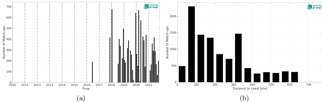
Figure 2: Number of match-ups between TSG (LEGOS-DM) and SMOS SSS L2Q v331 - With FLAG (CMEMS-CATDS-CPDC) SSS as a function of time (a) and as function of the distance to coast (b) over the Congo river plume Pi-MEP region and for the full satellite product period.
