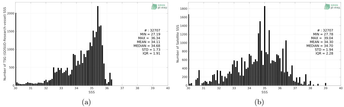
Figure 2: Histograms of SSS from TSG (GOSUD-Research-vessel) (a) and SMOS SSS L2Q v331 - With FLAG (CMEMS-CATDS-CPDC) (b) considering all match-up pairs per bins of 0.1 over the Congo river plume Pi-MEP region and for the full satellite product period.
