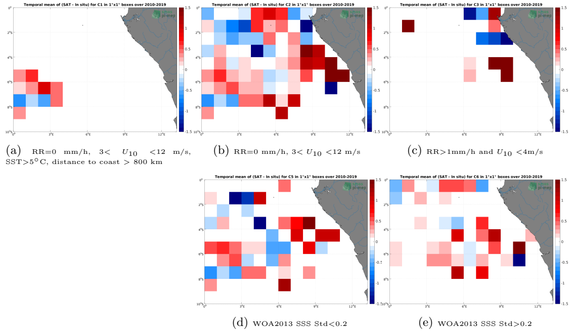
Figure 12: Temporal mean gridded over spatial boxes of size 1^\circ \times 1^\circ of \Delta SSS (SMOS SSS L2Q v331 - With FLAG (CMEMS-CATDS-CPDC) - TSG (GOSUD-Research-vessel)) for 5 different subdatasets corresponding to:RR=0 mm/h, 3 < U_{10} < 12 m/s, SST >5^\circ\text{C} , distance to coast > 800 km (a), RR=0 mm/h, 3 < U_{10} < 12 m/s (b), RR >1 mm/h and U_{10} < 4 m/s (c), WOA2013 SSS Std <0.2 (d), WOA2013 SSS Std >0.2 (e).
