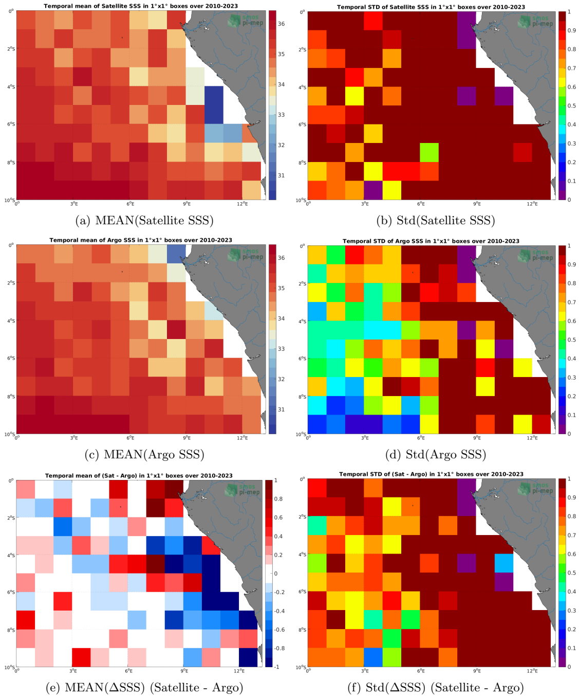
Figure 6: Temporal mean (left) and Std (right) of SSS from SMOS SSS L2Q v331 - With FLAG (CMEMS-CATDS-CPDC) (top), Argo (middle), and of \Delta SSS (Satellite - Argo). Only match-up pairs are used to generate these maps.
