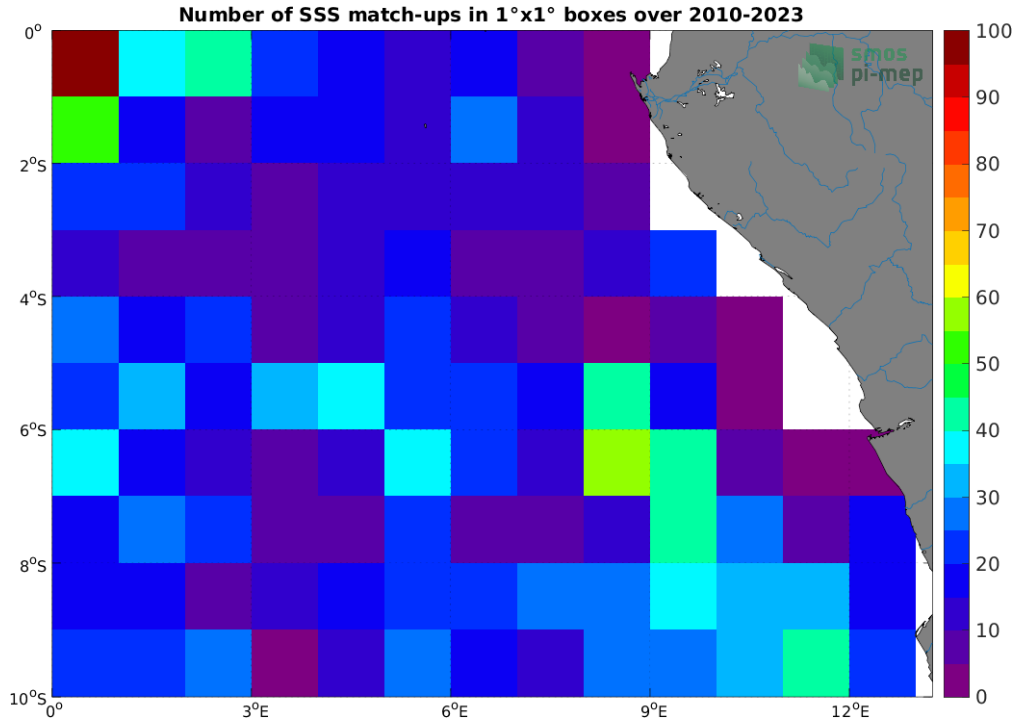
Figure 4: Number of SSS match-ups between Argo SSS and the SMOS SSS L2Q v331 - With FLAG (CMEMS-CATDS-CPDC) SSS product for the Congo river plume Pi-MEP region over 1^\circ \times 1^\circ boxes and for the full satellite product period.
