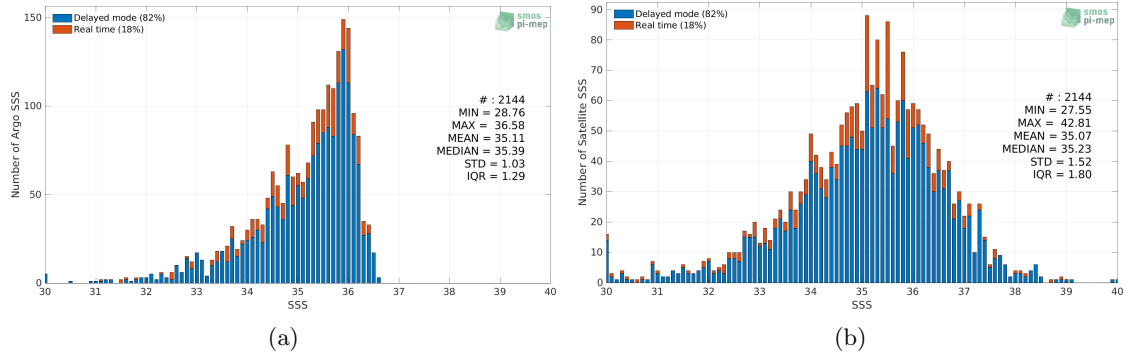
Figure 2: Histograms of SSS from Argo (a) and SMOS SSS L2Q v331 - With FLAG (CMEMS-CATDS-CPDC) (b) considering all match-up pairs per bins of 0.1 over the Congo river plume Pi-MEP region and for the full satellite product period.
