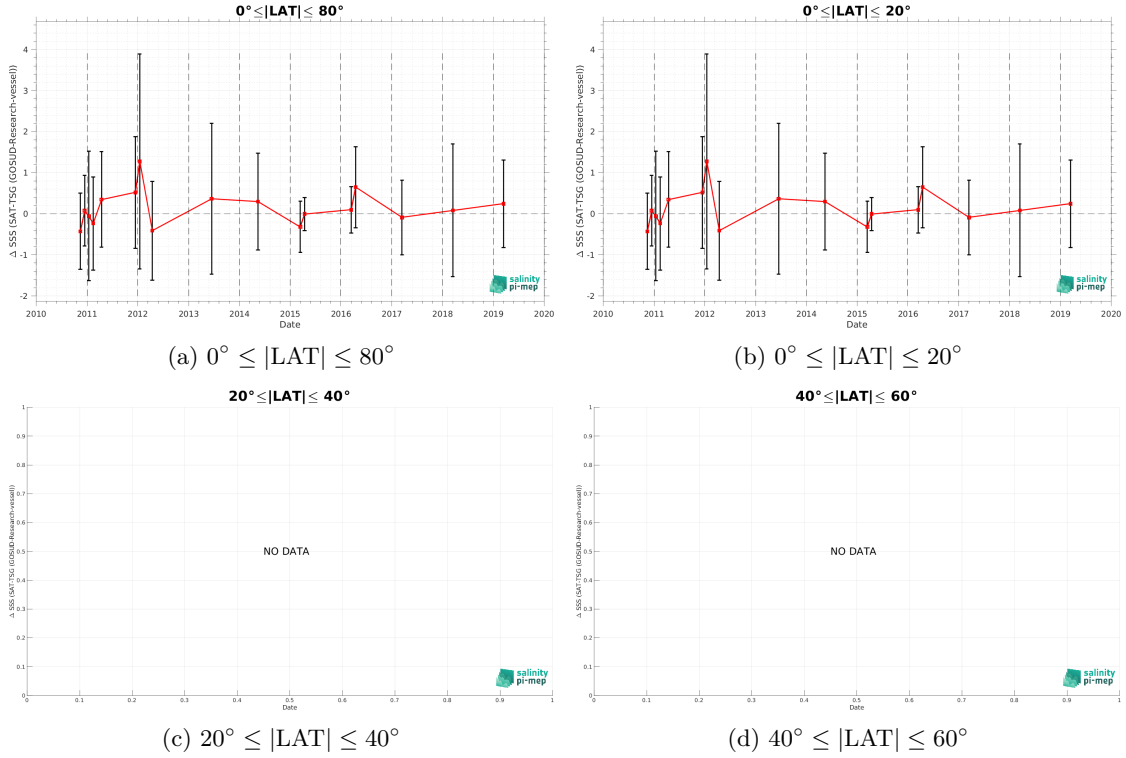
Figure 10: Monthly median (red curves) of \Delta SSS (Satellite - in situ ) between SMOS SSS L2Q v331 - No FLAG (CMEMS-CATDS-CPDC) and TSG (GOSUD-Research-vessel) SSS as function of time for all the collected Pi-MEP match-up pairs estimated over the Congo river plume Pi-MEP region and for the full satellite product period are shown for different latitude bands: (a) 80^\circ\text{S}-80^\circ\text{N} , (b) 20^\circ\text{S}-20^\circ\text{N} , (c) 40^\circ\text{S}-20^\circ\text{S} and 20^\circ\text{N}-40^\circ\text{N} and (d) 60^\circ\text{S}-40^\circ\text{S} and 40^\circ\text{N}-60^\circ\text{N} .
