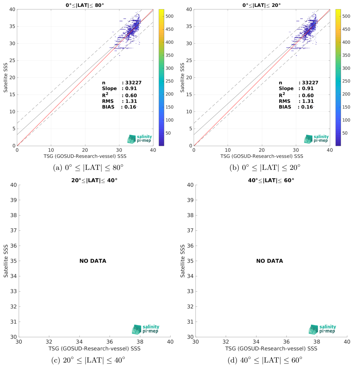
Figure 9: Contour maps of the concentration of SMOS SSS L2Q v331 - No FLAG (CMEMS-CATDS-CPDC) SSS ( y -axis) versus TSG (GOSUD-Research-vessel) SSS ( x -axis) at match-up pairs for different latitude bands. For each plot, the red line shows x=y . The black thin and dashed lines indicate a linear fit through the data cloud and the \pm 95\% confidence levels, respectively. The number match-up pairs n , the slope and R^2 coefficient of the linear fit, the root mean square (RMS) and the mean bias between satellite and in situ data are indicated for each latitude band in each plots.
