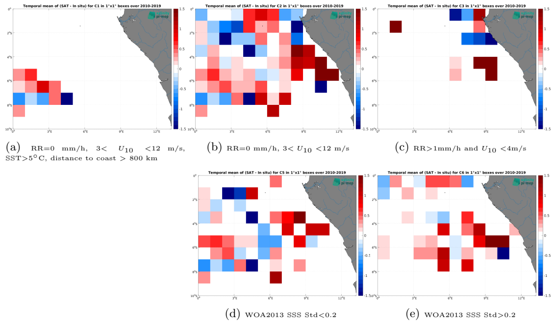
Figure 12: Temporal mean gridded over spatial boxes of size 1^{\circ}\times 1^{\circ} of \Delta SSS (SMOS SSS L2Q v331 - No FLAG (CMEMS-CATDS-CPDC) - TSG (GOSUD-Research-vessel)) for 5 different subdatasets corresponding to:RR=0 mm/h, 3 < U_{10} < 12 m/s, SST >5^{\circ}\text{C} , distance to coast > 800 km (a), RR=0 mm/h, 3 < U_{10} < 12 m/s (b), RR >1 mm/h and U_{10} < 4 m/s (c), WOA2013 SSS Std <0.2 (d), WOA2013 SSS Std >0.2 (e).
