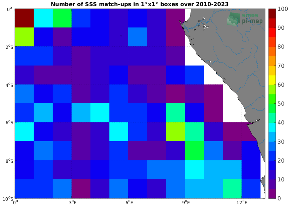
Figure 4: Number of SSS match-ups between Argo SSS and the SMOS SSS L2Q v331 - No FLAG (CMEMS-CATDS-CPDC) SSS product for the Congo river plume Pi-MEP region over 1^\circ \times 1^\circ boxes and for the full satellite product period.
