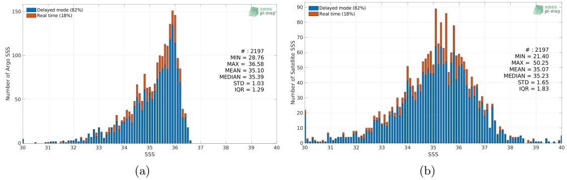
Figure 2: Histograms of SSS from Argo (a) and SMOS SSS L2Q v331 - No FLAG (CMEMS-CATDS-CPDC) (b) considering all match-up pairs per bins of 0.1 over the Congo river plume Pi-MEP region and for the full satellite product period.
