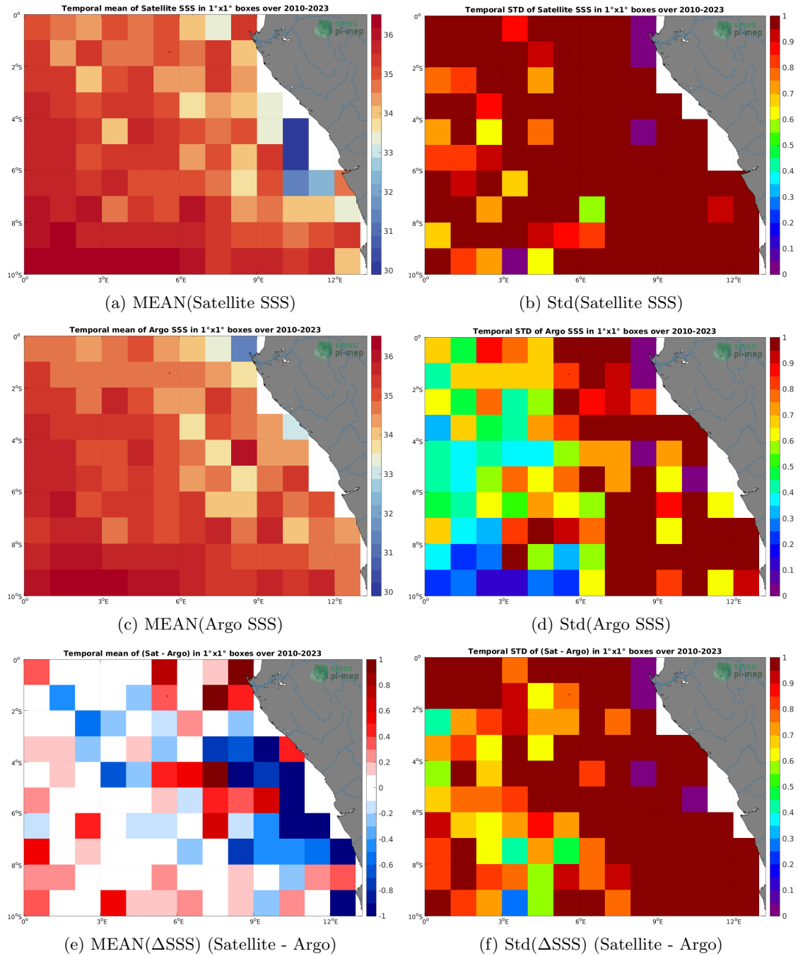
Figure 6: Temporal mean (left) and Std (right) of SSS from SMOS SSS L2Q v331 - No FLAG (CMEMS-CATDS-CPDC) (top), Argo (middle), and of \Delta SSS (Satellite - Argo). Only match-up pairs are used to generate these maps.
