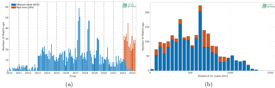
Figure 1: Number of match-ups between Argo and SMOS SSS L2Q v331 - No FLAG (CMEMS-CATDS-CPDC) SSS as a function of time (a) and as function of the distance to coast (b) over the Congo river plume Pi-MEP region and for the full satellite product period.
