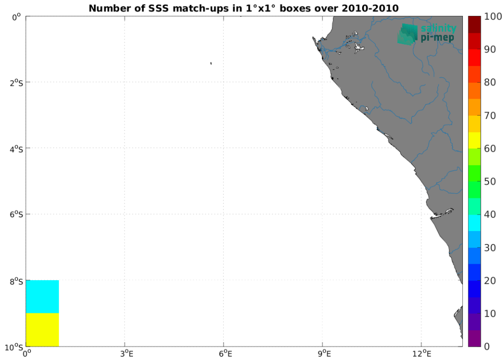
Figure 5: Number of SSS match-ups between TSG (SAMOS) SSS and the SMOS SSS L3 v9 - 9 Days (CATDS-CEC-LOCEAN) SSS product for the Congo river plume Pi-MEP region over 1^\circ \times 1^\circ boxes and for the full satellite product period.
