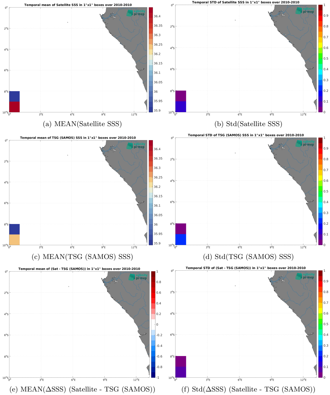
Figure 7: Temporal mean (left) and Std (right) of SSS from SMOS SSS L3 v9 - 9 Days (CATDS-CEC-LOCEAN) (top), TSG (SAMOS) (middle), and of \Delta SSS (Satellite - TSG (SAMOS)). Only match-up pairs are used to generate these maps.
