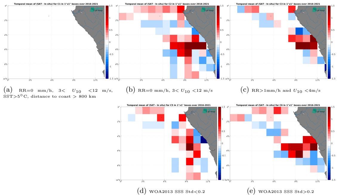
Figure 14: Temporal mean gridded over spatial boxes of size 1^\circ \times 1^\circ of \Delta SSS (SMOS SSS L3 v9 - 9 Days (CATDS-CEC-LOCEAN) - TSG (LEGOS-DM)) for 5 different subdatasets corresponding to:RR=0 mm/h, 3 < U_{10} < 12 m/s, SST > 5°C, distance to coast > 800 km (a), RR=0 mm/h, 3 < U_{10} < 12 m/s (b), RR > 1mm/h and U_{10} < 4 m/s (c), WOA2013 SSS Std < 0.2 (d), WOA2013 SSS Std > 0.2 (e).
