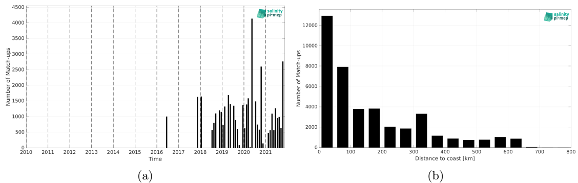
Figure 2: Number of match-ups between TSG (LEGOS-DM) and SMOS SSS L3 v9 - 9 Days (CATDS-CEC-LOCEAN) SSS as a function of time (a) and as function of the distance to coast (b) over the Congo river plume Pi-MEP region and for the full satellite product period.
