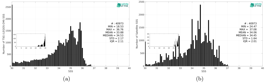
Figure 3: Histograms of SSS from TSG (LEGOS-DM) (a) and SMOS SSS L3 v9 - 9 Days (CATDS-CEC-LOCEAN) (b) considering all match-up pairs per bins of 0.1 over the Congo river plume Pi-MEP region and for the full satellite product period.
