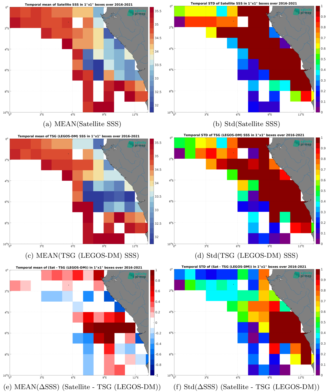
Figure 7: Temporal mean (left) and Std (right) of SSS from SMOS SSS L3 v9 - 9 Days (CATDS-CEC-LOCEAN) (top), TSG (LEGOS-DM) (middle), and of \Delta SSS (Satellite - TSG (LEGOS-DM)). Only match-up pairs are used to generate these maps.
