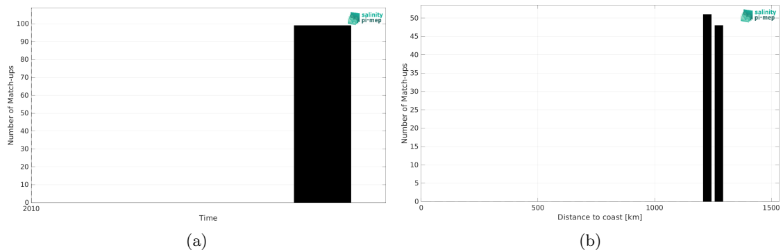
Figure 1: Number of match-ups between TSG (SAMOS) and SMOS SSS L3 v8 - 9 Days (CATDS-CEC-LOCEAN) SSS as a function of time (a) and as function of the distance to coast (b) over the Congo river plume Pi-MEP region and for the full satellite product period.
