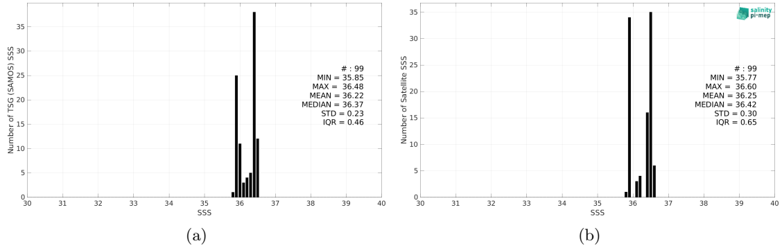
Figure 2: Histograms of SSS from TSG (SAMOS) (a) and SMOS SSS L3 v8 - 9 Days (CATDS-CEC-LOCEAN) (b) considering all match-up pairs per bins of 0.1 over the Congo river plume Pi-MEP region and for the full satellite product period.
