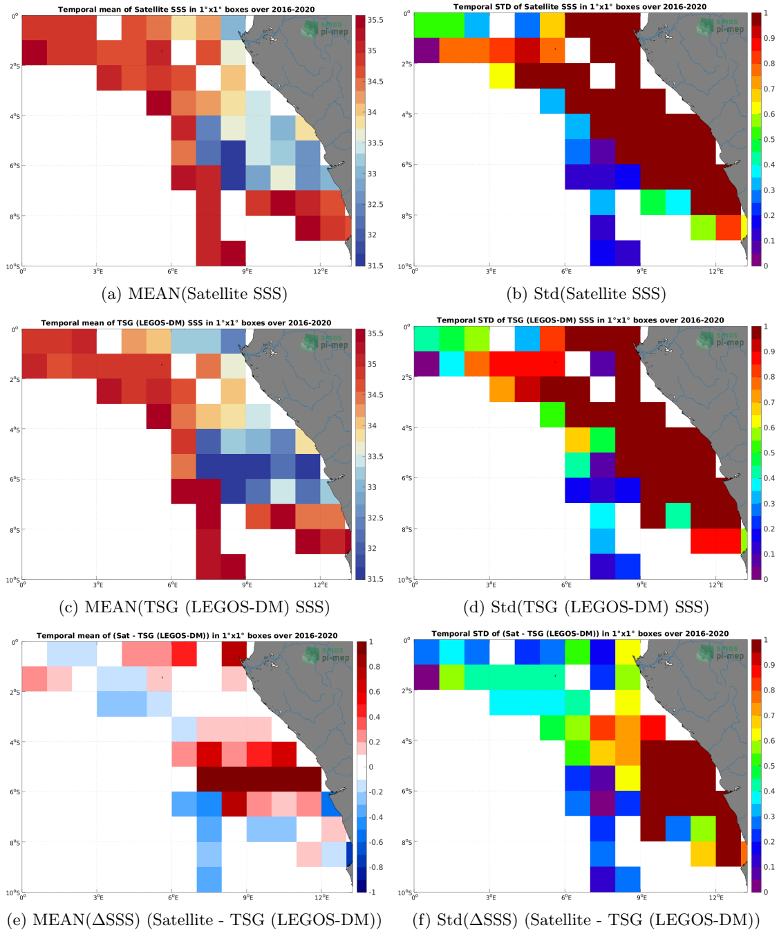
Figure 6: Temporal mean (left) and Std (right) of SSS from SMOS SSS L3 v8 - 9 Days (CATDS-CECOS-LOCEAN) (top), TSG (LEGOS-DM) (middle), and of \Delta SSS (Satellite - TSG (LEGOS-DM)). Only match-up pairs are used to generate these maps.
