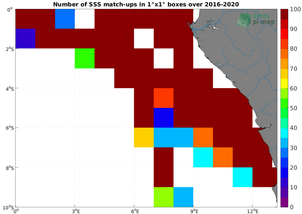
Figure 4: Number of SSS match-ups between TSG (LEGOS-DM) SSS and the SMOS SSS L3 v8 - 9 Days (CATDS-CECOS-LOCEAN) SSS product for the Congo river plume Pi-MEP region over 1^\circ \times 1^\circ boxes and for the full satellite product period.
