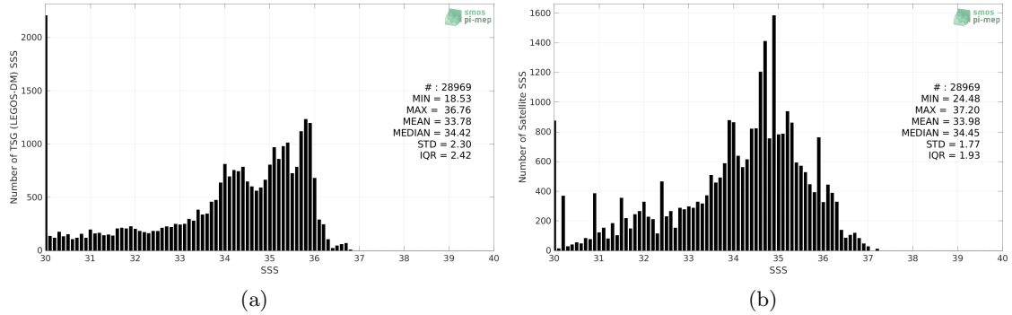
Figure 2: Histograms of SSS from TSG (LEGOS-DM) (a) and SMOS SSS L3 v8 - 9 Days (CATDS-CECOS-LOCEAN) (b) considering all match-up pairs per bins of 0.1 over the Congo river plume Pi-MEP region and for the full satellite product period.
