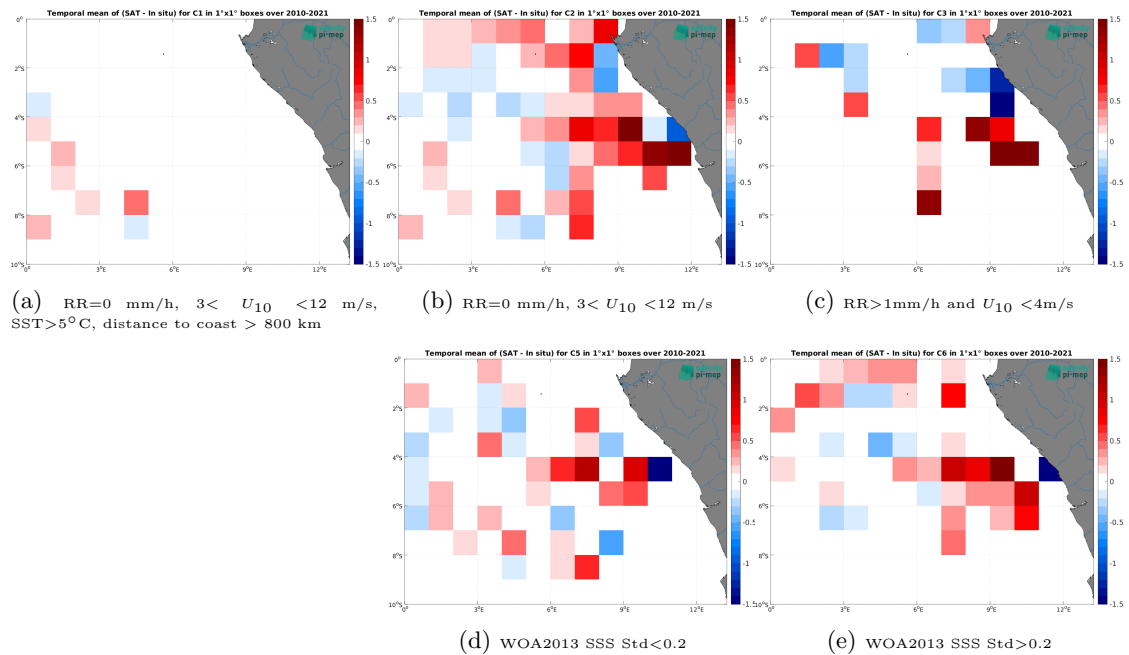
Figure 12: Temporal mean gridded over spatial boxes of size 1^\circ \times 1^\circ of \Delta SSS (SMOS SSS L3 v8 - 9 Days (CATDS-CEC-LOCEAN) - TSG (GOSUD-Research-vessel)) for 5 different subdatasets corresponding to:RR=0 mm/h, 3 < U_{10} < 12 m/s, SST > 5°C, distance to coast > 800 km (a), RR=0 mm/h, 3 < U_{10} < 12 m/s (b), RR > 1mm/h and U_{10} < 4 m/s (c), WOA2013 SSS Std < 0.2 (d), WOA2013 SSS Std > 0.2 (e).
