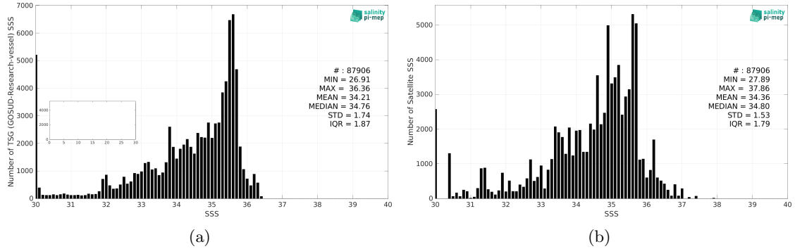
Figure 2: Histograms of SSS from TSG (GOSUD-Research-vessel) (a) and SMOS SSS L3 v8 - 9 Days (CATDS-CEC-LOCEAN) (b) considering all match-up pairs per bins of 0.1 over the Congo river plume Pi-MEP region and for the full satellite product period.
