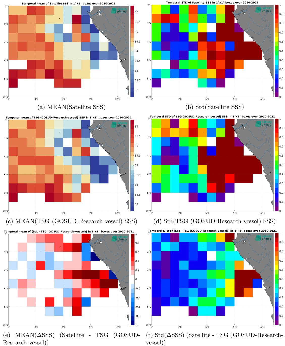
Figure 6: Temporal mean (left) and Std (right) of SSS from SMOS SSS L3 v8 - 9 Days (CATDS-CEC-LOCEAN) (top), TSG (GOSUD-Research-vessel) (middle), and of \Delta SSS (Satellite - TSG (GOSUD-Research-vessel)). Only match-up pairs are used to generate these maps.
