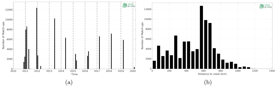
Figure 1: Number of match-ups between TSG (GOSUD-Research-vessel) and SMOS SSS L3 v8 - 9 Days (CATDS-CECOS-LOCEAN) SSS as a function of time (a) and as function of the distance to coast (b) over the Congo river plume Pi-MEP region and for the full satellite product period.
