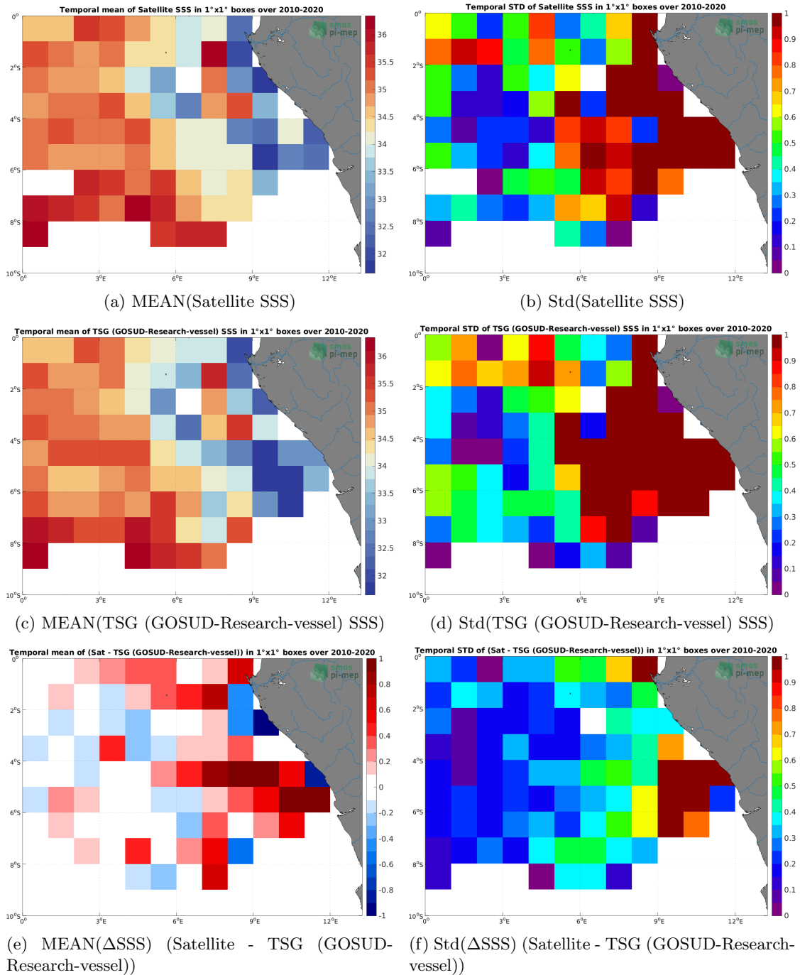
Figure 6: Temporal mean (left) and Std (right) of SSS from SMOS SSS L3 v8 - 9 Days (CATDS-CECOS-LOCEAN) (top), TSG (GOSUD-Research-vessel) (middle), and of \Delta SSS (Satellite - TSG (GOSUD-Research-vessel)). Only match-up pairs are used to generate these maps.
