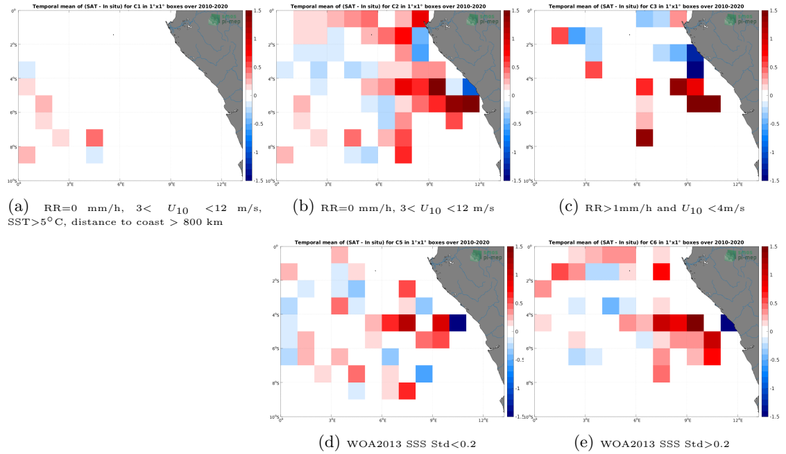
Figure 12: Temporal mean gridded over spatial boxes of size 1^\circ \times 1^\circ of \Delta SSS (SMOS SSS L3 v8 - 9 Days (CATDS-CECOS-LOCEAN) - TSG (GOSUD-Research-vessel)) for 5 different subdatasets corresponding to:RR=0 mm/h, 3 < U_{10} < 12 m/s, SST >5^\circ\text{C} , distance to coast > 800 km (a), RR=0 mm/h, 3 < U_{10} < 12 m/s (b), RR >1 mm/h and U_{10} < 4 m/s (c), WOA2013 SSS Std <0.2 (d), WOA2013 SSS Std >0.2 (e).
