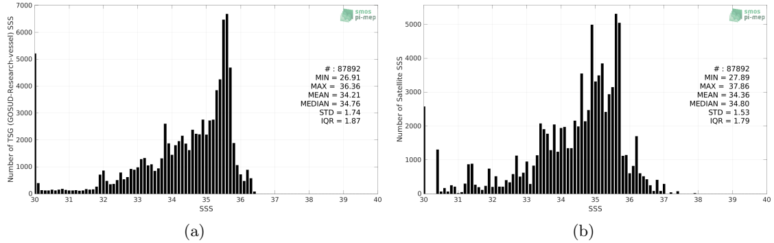
Figure 2: Histograms of SSS from TSG (GOSUD-Research-vessel) (a) and SMOS SSS L3 v8 - 9 Days (CATDS-CECOS-LOCEAN) (b) considering all match-up pairs per bins of 0.1 over the Congo river plume Pi-MEP region and for the full satellite product period.
