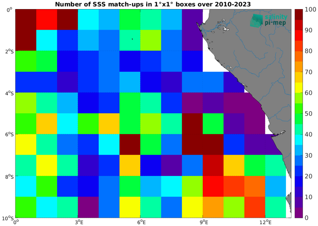
Figure 4: Number of SSS match-ups between Argo SSS and the SMOS SSS L3 v8 - 18 Days (CATDS-CEC-LOCEAN) SSS product for the Congo river plume Pi-MEP region over 1^\circ \times 1^\circ boxes and for the full satellite product period.
