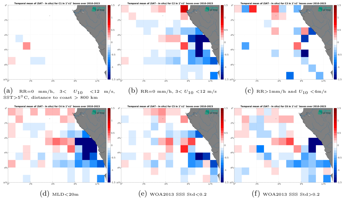
Figure 12: Temporal mean gridded over spatial boxes of size 1^\circ \times 1^\circ of \Delta SSS (SMOS SSS L3 v8 - 18 Days (CATDS-CEC-LOCEAN) - Argo) for 6 different subdatasets corresponding to:RR=0 mm/h, 3 < U_{10} < 12 m/s, SST >5^\circ\text{C} , distance to coast > 800 km (a), RR=0 mm/h, 3 < U_{10} < 12 m/s (b), RR >1 mm/h and U_{10} < 4 m/s (c),MLD <20 m (d),WOA2013 SSS Std <0.2 (e),WOA2013 SSS Std >0.2 (f).
