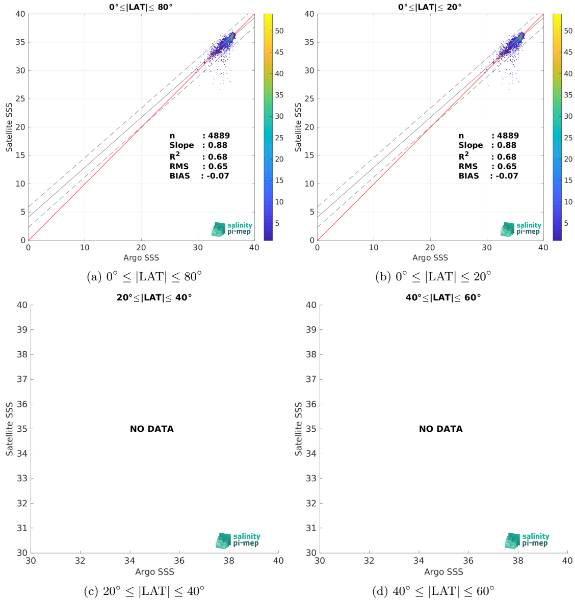
Figure 9: Contour maps of the concentration of SMOS SSS L3 v8 - 18 Days (CATDS-CEC-LOCEAN) SSS (y-axis) versus Argo SSS (x-axis) at match-up pairs for different latitude bands. For each plot, the red line shows x=y . The black thin and dashed lines indicate a linear fit through the data cloud and the \pm 95\% confidence levels, respectively. The number match-up pairs n , the slope and R^2 coefficient of the linear fit, the root mean square (RMS) and the mean bias between satellite and in situ data are indicated for each latitude band in each plots.
