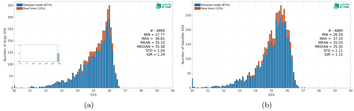
Figure 2: Histograms of SSS from Argo (a) and SMOS SSS L3 v8 - 18 Days (CATDS-CEC-LOCEAN) (b) considering all match-up pairs per bins of 0.1 over the Congo river plume Pi-MEP region and for the full satellite product period.
