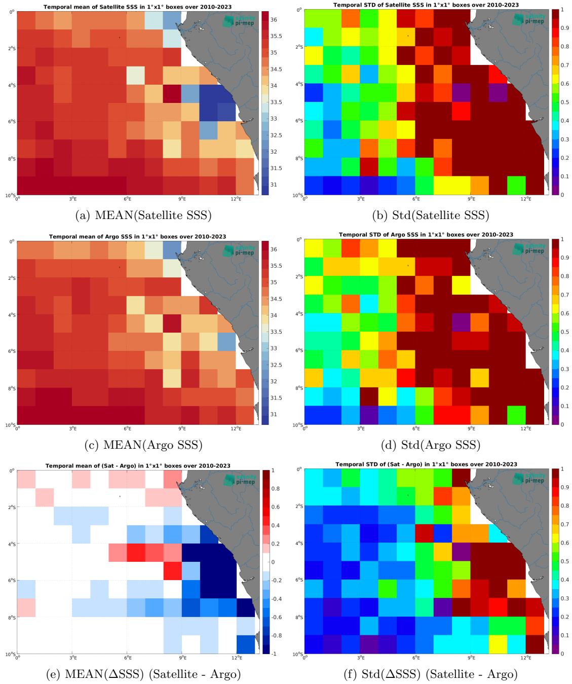
Figure 6: Temporal mean (left) and Std (right) of SSS from SMOS SSS L3 v8 - 18 Days (CATDS-CEC-LOCEAN) (top), Argo (middle), and of \Delta SSS (Satellite - Argo). Only match-up pairs are used to generate these maps.
