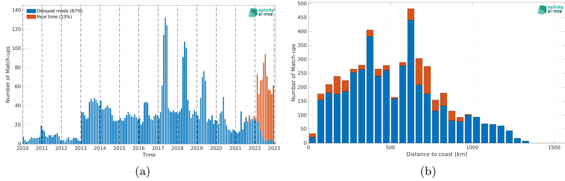
Figure 1: Number of match-ups between Argo and SMOS SSS L3 v8 - 18 Days (CATDS-CEC-LOCEAN) SSS as a function of time (a) and as function of the distance to coast (b) over the Congo river plume Pi-MEP region and for the full satellite product period.
