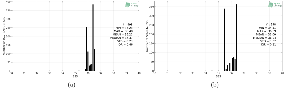
Figure 2: Histograms of SSS from TSG (SAMOS) (a) and SMOS SSS L3 v5 - 9 Days (CATDS-CECOS-LOCEAN) (b) considering all match-up pairs per bins of 0.1 over the Congo river plume Pi-MEP region and for the full satellite product period.
