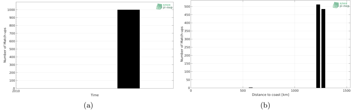
Figure 1: Number of match-ups between TSG (SAMOS) and SMOS SSS L3 v5 - 9 Days (CATDS-CECOS-LOCEAN) SSS as a function of time (a) and as function of the distance to coast (b) over the Congo river plume Pi-MEP region and for the full satellite product period.
