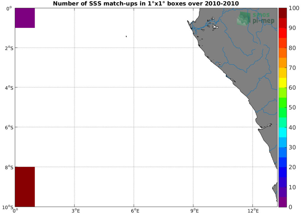
Figure 4: Number of SSS match-ups between TSG (SAMOS) SSS and the SMOS SSS L3 v5 - 9 Days (CATDS-CECOS-LOCEAN) SSS product for the Congo river plume Pi-MEP region over 1^\circ \times 1^\circ boxes and for the full satellite product period.
