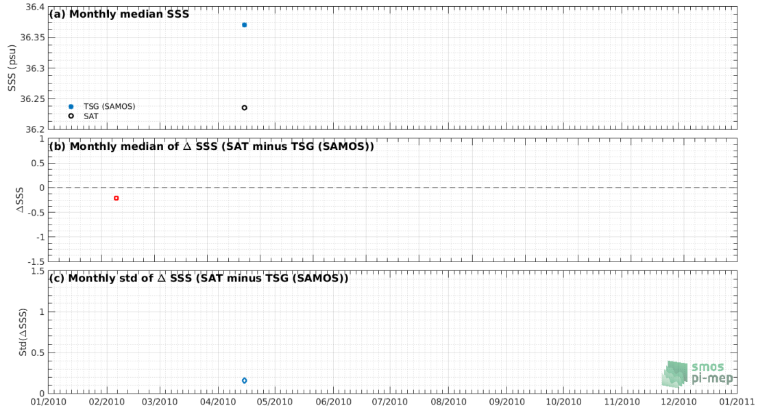
Figure 7: Time series of the monthly median SSS (top), median of \Delta SSS (Satellite - TSG (SAMOS)) and Std of \Delta SSS (Satellite - TSG (SAMOS)) over the Congo river plume Pi-MEP region considering all match-ups collected by the Pi-MEP.
