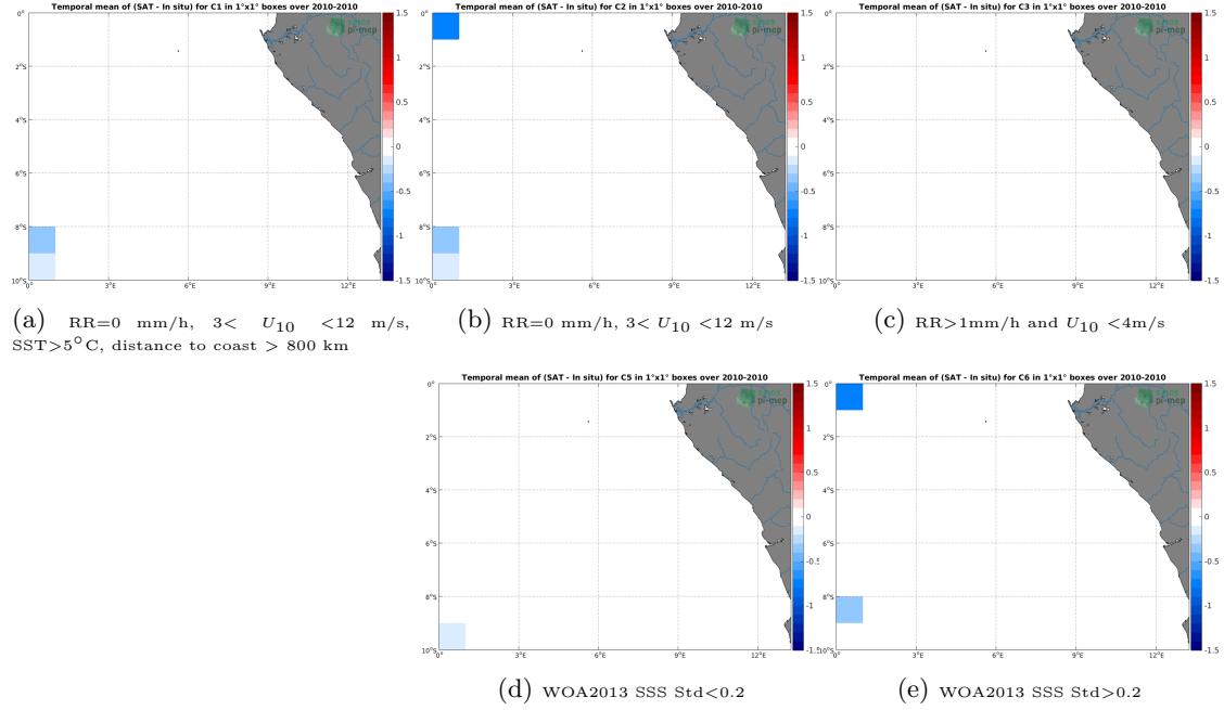
Figure 12: Temporal mean gridded over spatial boxes of size 1^{\circ} \times 1^{\circ} of \Delta\text{SSS} (SMOS SSS L3 v5 - 9 Days (CATDS-CECOS-LOCEAN) - TSG (SAMOS)) for 5 different subdatasets corresponding to:RR=0 mm/h, 3 < U_{10} < 12 m/s, SST >5^{\circ}\text{C} , distance to coast > 800 km (a), RR=0 mm/h, 3 < U_{10} < 12 m/s (b), RR >1 mm/h and U_{10} < 4 m/s (c), WOA2013 SSS Std <0.2 (d), WOA2013 SSS Std >0.2 (e).
