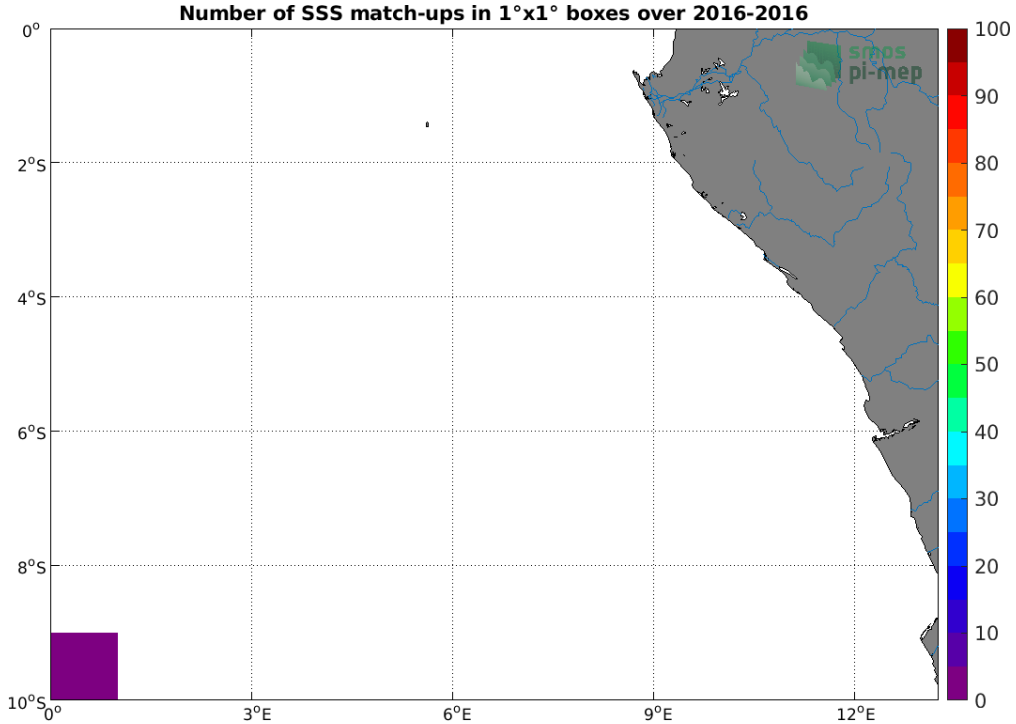
Figure 4: Number of SSS match-ups between TSG (Polarstern) SSS and the SMOS SSS L3 v5 - 9 Days (CATDS-CECOS-LOCEAN) SSS product for the Congo river plume Pi-MEP region over 1^\circ \times 1^\circ boxes and for the full satellite product period.
