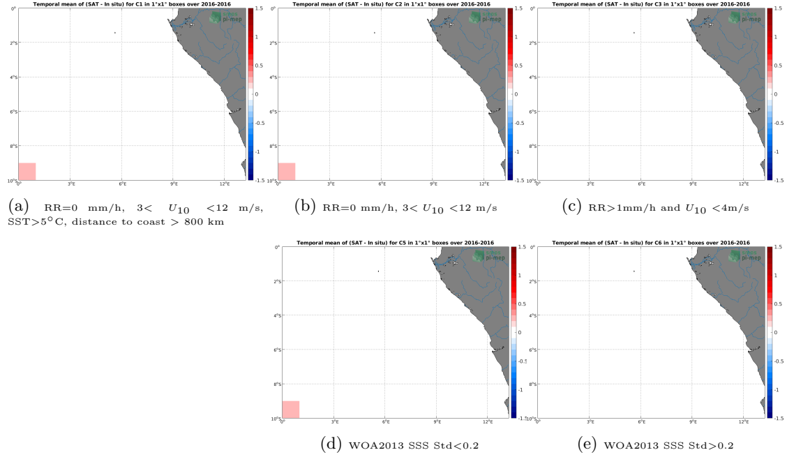
Figure 12: Temporal mean gridded over spatial boxes of size 1^{\circ}\times 1^{\circ} of \Delta\text{SSS} (SMOS SSS L3 v5 - 9 Days (CATDS-CECOS-LOCEAN) - TSG (Polarstern)) for 5 different subdatasets corresponding to:RR=0 mm/h, 3 < U_{10} < 12 m/s, SST >5^{\circ}\text{C} , distance to coast > 800 km (a), RR=0 mm/h, 3 < U_{10} < 12 m/s (b), RR >1 mm/h and U_{10} < 4 m/s (c), WOA2013 SSS Std <0.2 (d), WOA2013 SSS Std >0.2 (e).
