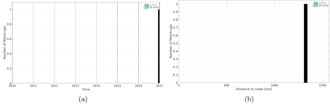
Figure 1: Number of match-ups between TSG (Polarstern) and SMOS SSS L3 v5 - 9 Days (CATDS-CECOS-LOCEAN) SSS as a function of time (a) and as function of the distance to coast (b) over the Congo river plume Pi-MEP region and for the full satellite product period.
