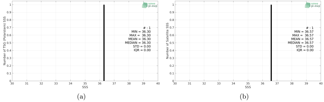
Figure 2: Histograms of SSS from TSG (Polarstern) (a) and SMOS SSS L3 v5 - 9 Days (CATDS-CECOS-LOCEAN) (b) considering all match-up pairs per bins of 0.1 over the Congo river plume Pi-MEP region and for the full satellite product period.
