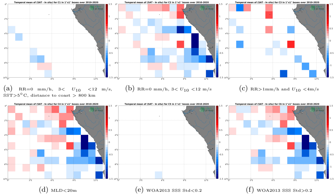
Figure 12: Temporal mean gridded over spatial boxes of size 1^\circ \times 1^\circ of \Delta SSS (SMOS SSS L3 v5 - 9 Days (CATDS-CECOS-LOCEAN) - Argo) for 6 different subdatasets corresponding to: RR=0 mm/h, 3 < U_{10} < 12 m/s, SST > 5^\circ C , distance to coast > 800 km (a), RR=0 mm/h, 3 < U_{10} < 12 m/s (b), RR > 1 mm/h and U_{10} < 4 m/s (c), MLD < 20 m (d), WOA2013 SSS Std < 0.2 (e), WOA2013 SSS Std > 0.2 (f).
