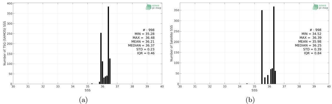
Figure 2: Histograms of SSS from TSG (SAMOS) (a) and SMOS SSS L3 v4 - 9 Days (CATDS-CECOS-LOCEAN) (b) considering all match-up pairs per bins of 0.1 over the Congo river plume Pi-MEP region and for the full satellite product period.
