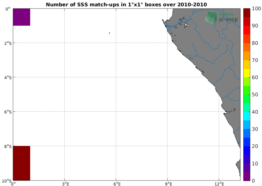
Figure 4: Number of SSS match-ups between TSG (SAMOS) SSS and the SMOS SSS L3 v4 - 9 Days (CATDS-CECOS-LOCEAN) SSS product for the Congo river plume Pi-MEP region over 1^\circ \times 1^\circ boxes and for the full satellite product period.
