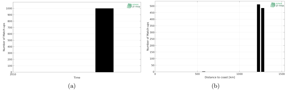
Figure 1: Number of match-ups between TSG (SAMOS) and SMOS SSS L3 v4 - 9 Days (CATDS-CECOS-LOCEAN) SSS as a function of time (a) and as function of the distance to coast (b) over the Congo river plume Pi-MEP region and for the full satellite product period.
