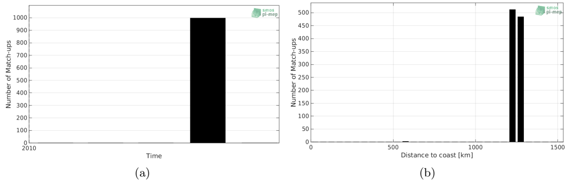
Figure 1: Number of match-ups between TSG-SAMOS and SMOS-L3-CATDS-CECOS-LOCEAN-V4-9DAYS-25KM SSS as a function of time (a) and as function of the distance to coast (b) over the Congo river plume Pi-MEP region and for the full satellite product period.
