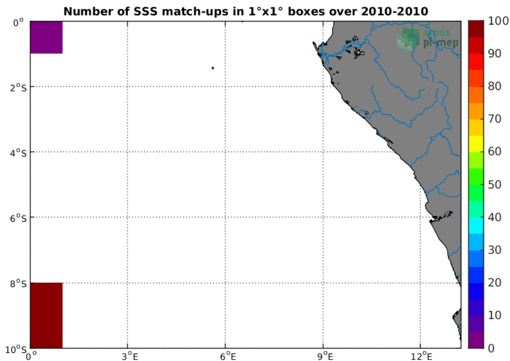
Figure 4: Number of SSS match-ups between TSG-SAMOS SSS and the SMOS-L3-CATDS-CECOS-LOCEAN-V4-9DAYS-25KM SSS product for the Congo river plume Pi-MEP region over 1^\circ \times 1^\circ boxes and for the full satellite product period.
