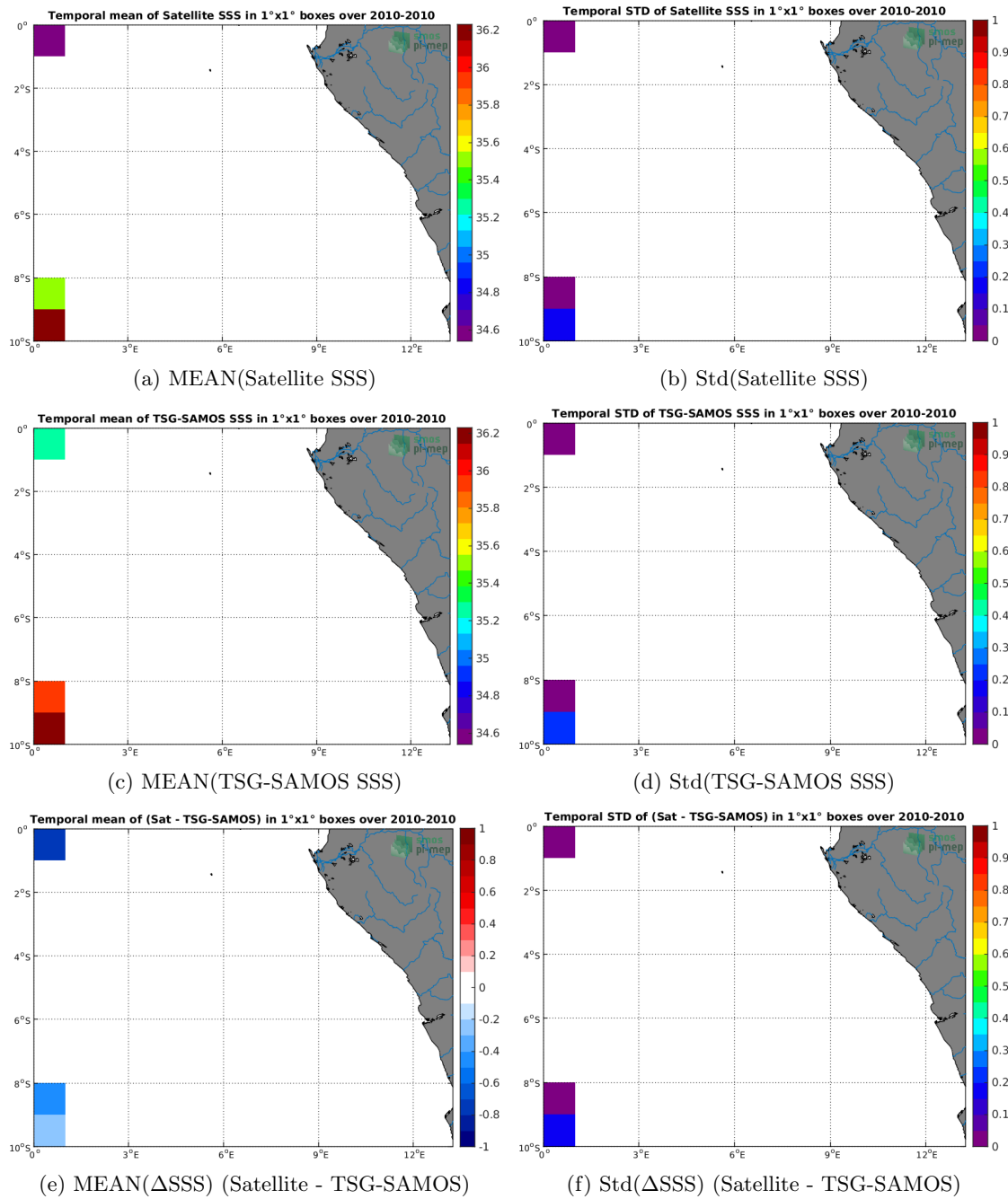
Figure 6: Temporal mean (left) and Std (right) of SSS from SMOS-L3-CATDS-CECOS-LOCEAN-V4-9DAYS-25KM (top), TSG-SAMOS (middle), and of \Delta SSS (Satellite - TSG-SAMOS). Only match-up pairs are used to generate these maps.
