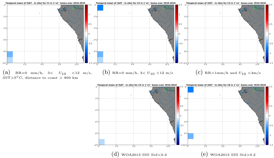
Figure 12: Temporal mean gridded over spatial boxes of size 1^\circ \times 1^\circ of \Delta SSS (SMOS-L3-CATDS-CECOS-LOCEAN-V4-9DAYS-25KM - TSG-SAMOS) for 5 different subdatasets corresponding to:RR=0 mm/h, 3 < U_{10} < 12 m/s, SST >5^\circ C, distance to coast > 800 km (a), RR=0 mm/h, 3 < U_{10} < 12 m/s (b), RR >1 mm/h and U_{10} < 4 m/s (c), WOA2013 SSS Std <0.2 (d), WOA2013 SSS Std >0.2 (e).
