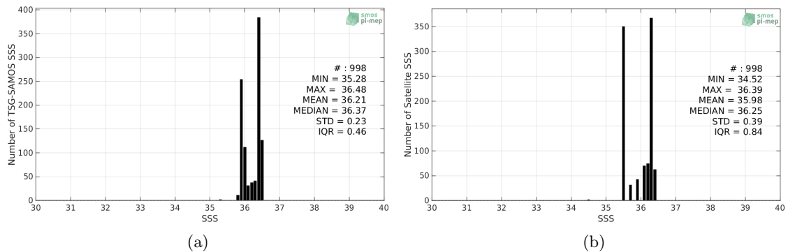
Figure 2: Histograms of SSS from TSG-SAMOS (a) and SMOS-L3-CATDS-CECOS-LOCEAN-V4-9DAYS-25KM (b) considering all match-up pairs per bins of 0.1 over the Congo river plume Pi-MEP region and for the full satellite product period.
