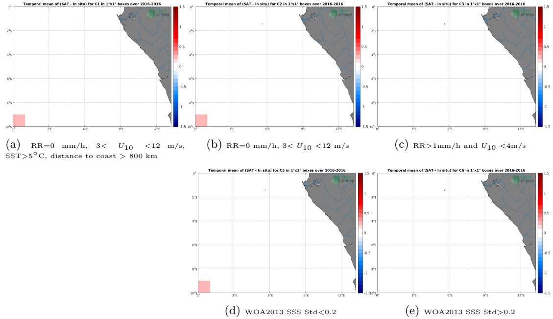
Figure 12: Temporal mean gridded over spatial boxes of size 1^{\circ}\times 1^{\circ} of \Delta\text{SSS} (SMOS SSS L3 v4 - 9 Days (CATDS-CECOS-LOCEAN) - TSG (Polarstern)) for 5 different subdatasets corresponding to:RR=0 mm/h, 3 < U_{10} < 12 m/s, SST >5^{\circ}\text{C} , distance to coast > 800 km (a), RR=0 mm/h, 3 < U_{10} < 12 m/s (b), RR >1 mm/h and U_{10} < 4 m/s (c), WOA2013 SSS Std <0.2 (d), WOA2013 SSS Std >0.2 (e).
