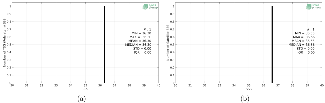
Figure 2: Histograms of SSS from TSG (Polarstern) (a) and SMOS SSS L3 v4 - 9 Days (CATDS-CECOS-LOCEAN) (b) considering all match-up pairs per bins of 0.1 over the Congo river plume Pi-MEP region and for the full satellite product period.
