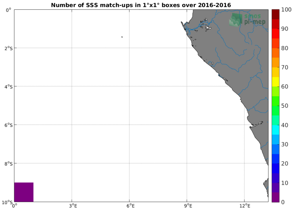
Figure 4: Number of SSS match-ups between TSG (Polarstern) SSS and the SMOS SSS L3 v4 - 9 Days (CATDS-CECOS-LOCEAN) SSS product for the Congo river plume Pi-MEP region over 1°x1° boxes and for the full satellite product period.
