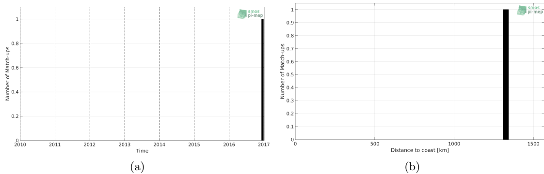
Figure 1: Number of match-ups between TSG (Polarstern) and SMOS SSS L3 v4 - 9 Days (CATDS-CECOS-LOCEAN) SSS as a function of time (a) and as function of the distance to coast (b) over the Congo river plume Pi-MEP region and for the full satellite product period.
