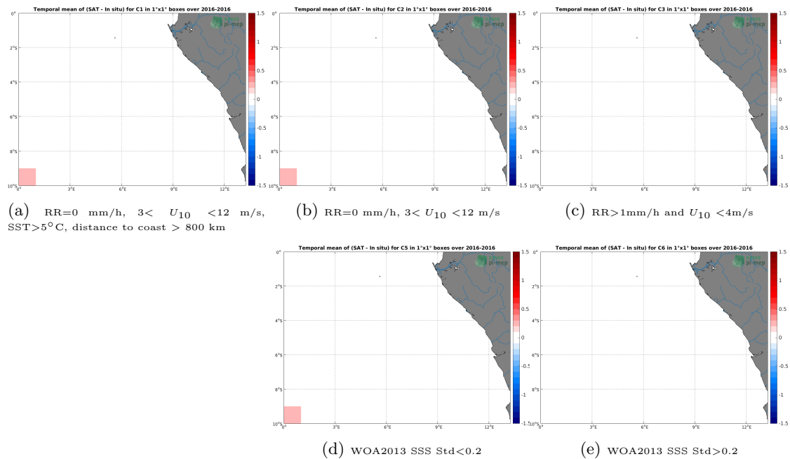
Figure 12: Temporal mean gridded over spatial boxes of size 1^{\circ}\times 1^{\circ} of \Delta\text{SSS} (SMOS-L3-CATDS-CECOS-LOCEAN-V4-9DAYS-25KM - TSG-POLARSTERN) for 5 different subdatasets corresponding to:RR=0 mm/h, 3 < U_{10} < 12 m/s, SST >5^{\circ}\text{C} , distance to coast > 800 km (a), RR=0 mm/h, 3 < U_{10} < 12 m/s (b), RR >1 mm/h and U_{10} < 4 m/s (c), WOA2013 SSS Std <0.2 (d), WOA2013 SSS Std >0.2 (e).
