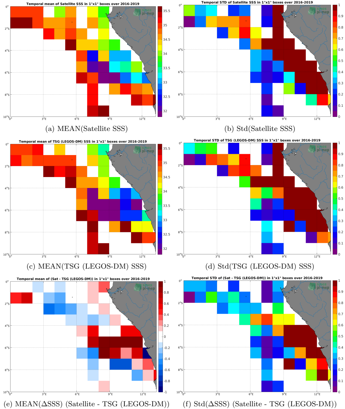
Figure 6: Temporal mean (left) and Std (right) of SSS from SMOS SSS L3 v4 - 9 Days (CATDS-CECOS-LOCEAN) (top), TSG (LEGOS-DM) (middle), and of \Delta SSS (Satellite - TSG (LEGOS-DM)). Only match-up pairs are used to generate these maps.
