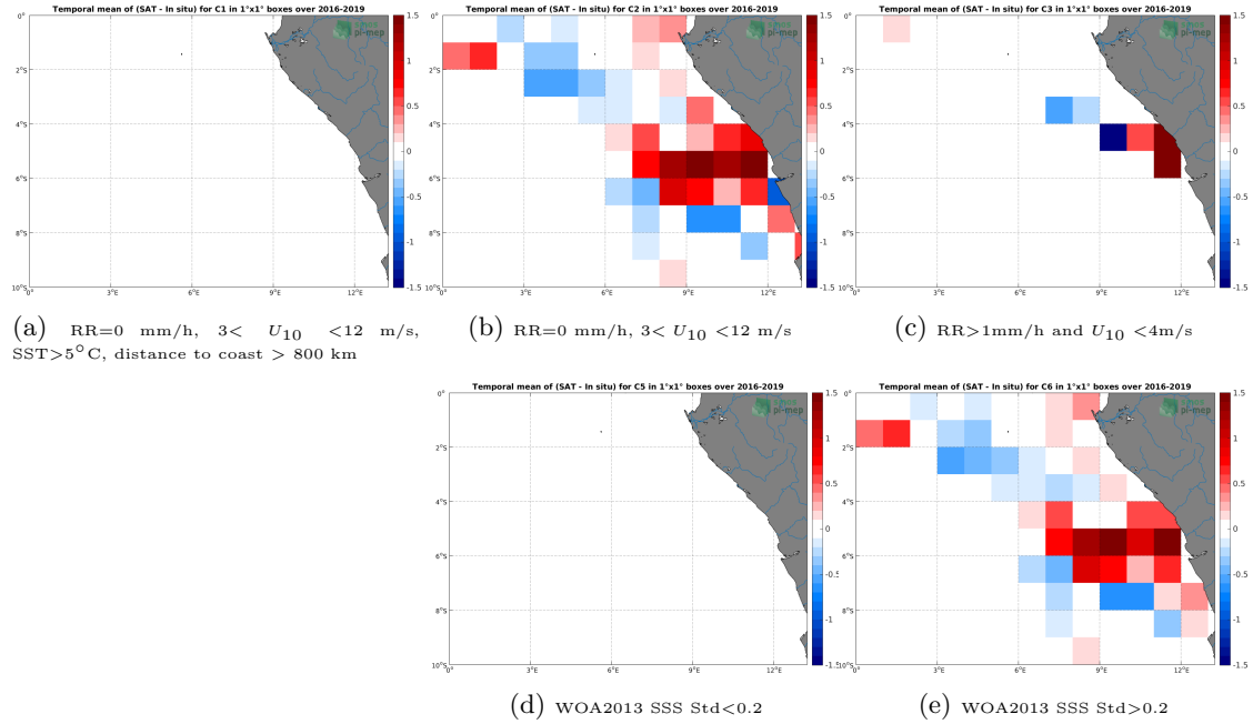
Figure 12: Temporal mean gridded over spatial boxes of size 1^{\circ}\times 1^{\circ} of \Delta\text{SSS} (SMOS SSS L3 v4 - 9 Days (CATDS-CECOS-LOCEAN) - TSG (LEGOS-DM)) for 5 different subdatasets corresponding to:RR=0 mm/h, 3 < U_{10} < 12 m/s, SST >5^{\circ}\text{C} , distance to coast > 800 km (a), RR=0 mm/h, 3 < U_{10} < 12 m/s (b), RR >1 mm/h and U_{10} < 4 m/s (c), WOA2013 SSS Std <0.2 (d), WOA2013 SSS Std >0.2 (e).
