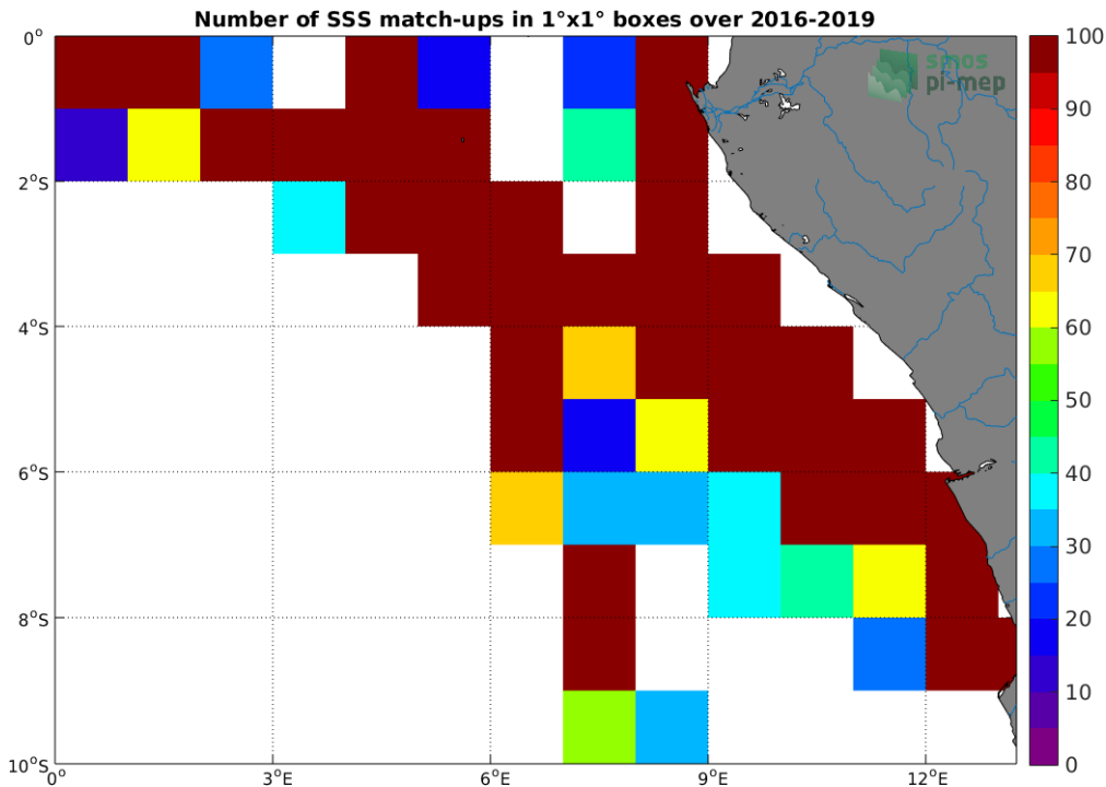
Figure 4: Number of SSS match-ups between TSG (LEGOS-DM) SSS and the SMOS SSS L3 v4 - 9 Days (CATDS-CECOS-LOCEAN) SSS product for the Congo river plume Pi-MEP region over 1°x1° boxes and for the full satellite product period.
