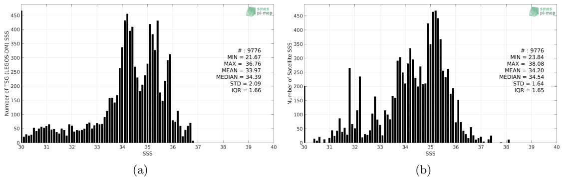
Figure 2: Histograms of SSS from TSG (LEGOS-DM) (a) and SMOS SSS L3 v4 - 9 Days (CATDS-CECOS-LOCEAN) (b) considering all match-up pairs per bins of 0.1 over the Congo river plume Pi-MEP region and for the full satellite product period.
