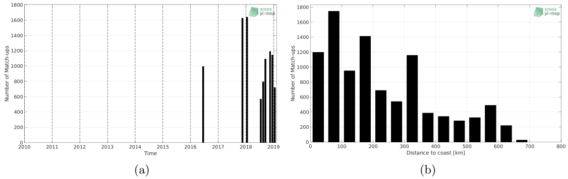
Figure 1: Number of match-ups between TSG-LEGOS-DM and SMOS-L3-CATDS-CECOS-LOCEAN-V4-9DAYS-25KM SSS as a function of time (a) and as function of the distance to coast (b) over the Congo river plume Pi-MEP region and for the full satellite product period.
