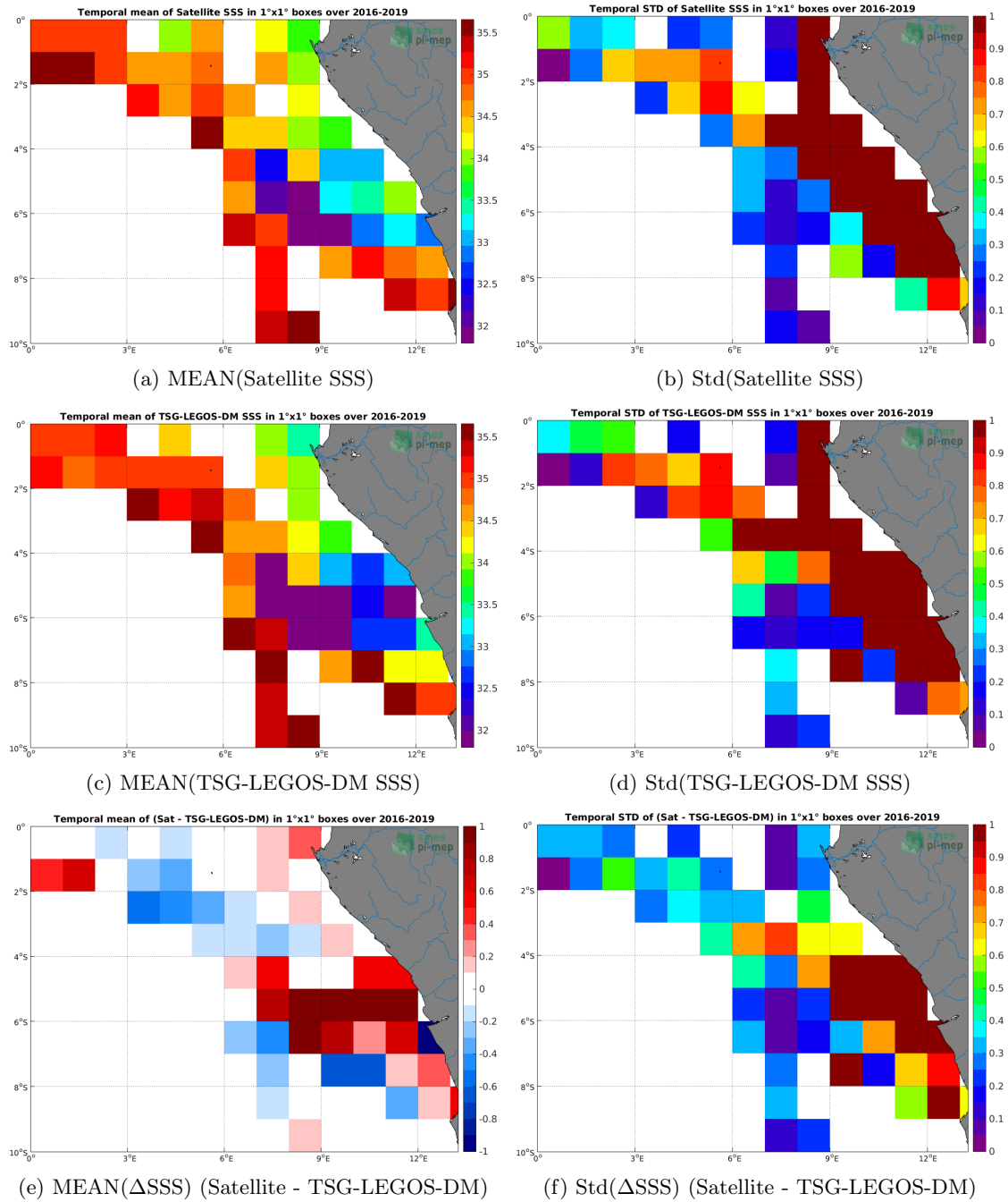
Figure 6: Temporal mean (left) and Std (right) of SSS from SMOS-L3-CATDS-CECOS-LOCEAN-V4-9DAYS-25KM (top), TSG-LEGOS-DM (middle), and of \Delta SSS (Satellite - TSG-LEGOS-DM). Only match-up pairs are used to generate these maps.
