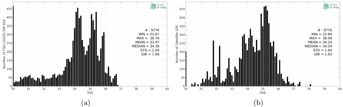
Figure 2: Histograms of SSS from TSG-LEGOS-DM (a) and SMOS-L3-CATDS-CECOS-LOCEAN-V4-9DAYS-25KM (b) considering all match-up pairs per bins of 0.1 over the Congo river plume Pi-MEP region and for the full satellite product period.
