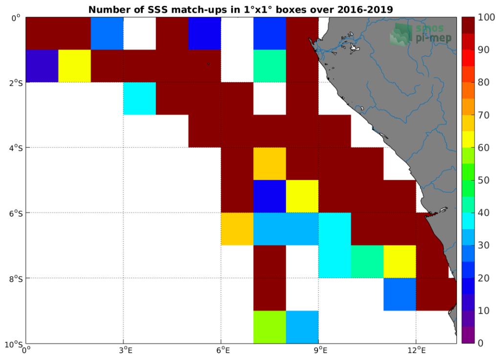
Figure 4: Number of SSS match-ups between TSG-LEGOS-DM SSS and the SMOS-L3-CATDS-CECOS-LOCEAN-V4-9DAYS-25KM SSS product for the Congo river plume Pi-MEP region over 1^\circ \times 1^\circ boxes and for the full satellite product period.
