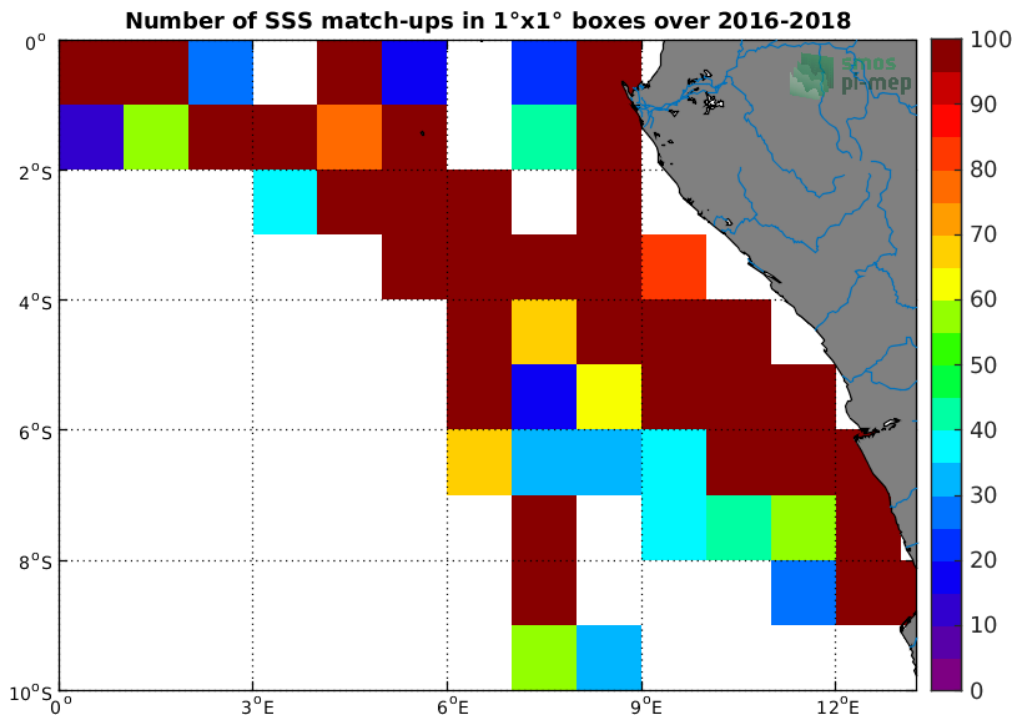
Figure 4: Number of SSS match-ups between TSG-LEGOS-DM SSS and the SMOS-L3-CATDS-CECOS-LOCEAN-V4-9DAYS-25KM SSS product for the Congo river plume Pi-MEP region over 1°x1° boxes and for the full satellite product period.
