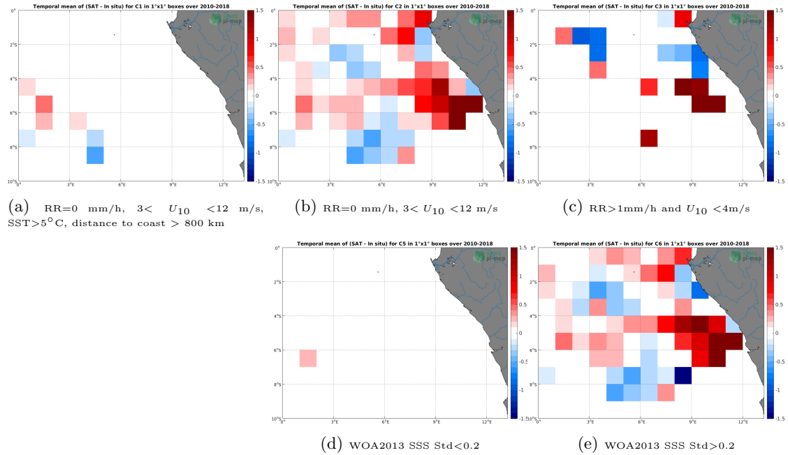
Figure 12: Temporal mean gridded over spatial boxes of size 1^\circ \times 1^\circ of \Delta SSS (SMOS SSS L3 v4 - 9 Days (CATDS-CECOS-LOCEAN) - TSG (GOSUD-Research-vessel)) for 5 different subdatasets corresponding to: RR=0 mm/h, 3 < U_{10} < 12 m/s, SST > 5^\circ\text{C} , distance to coast > 800 km (a), RR=0 mm/h, 3 < U_{10} < 12 m/s (b), RR > 1 mm/h and U_{10} < 4 m/s (c), WOA2013 SSS Std < 0.2 (d), WOA2013 SSS Std > 0.2 (e).
