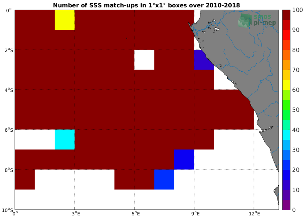
Figure 4: Number of SSS match-ups between TSG (GOSUD-Research-vessel) SSS and the SMOS SSS L3 v4 - 9 Days (CATDS-CECOS-LOCEAN) SSS product for the Congo river plume Pi-MEP region over 1^\circ \times 1^\circ boxes and for the full satellite product period.
