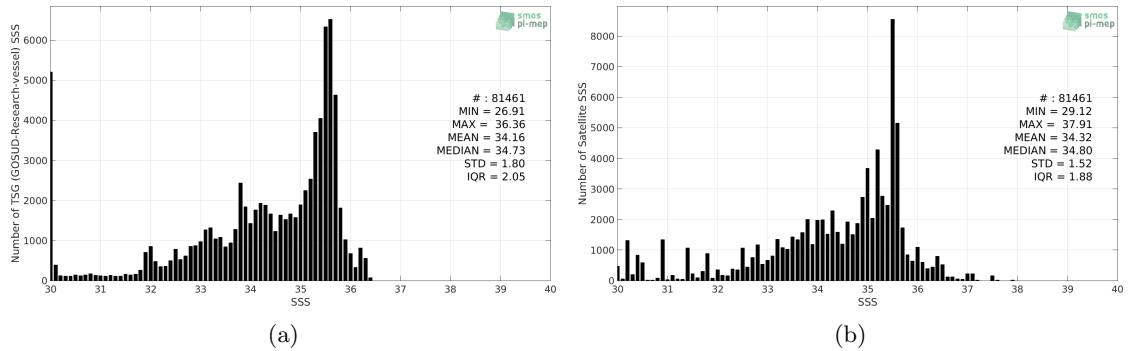
Figure 2: Histograms of SSS from TSG (GOSUD-Research-vessel) (a) and SMOS SSS L3 v4 - 9 Days (CATDS-CECOS-LOCEAN) (b) considering all match-up pairs per bins of 0.1 over the Congo river plume Pi-MEP region and for the full satellite product period.
