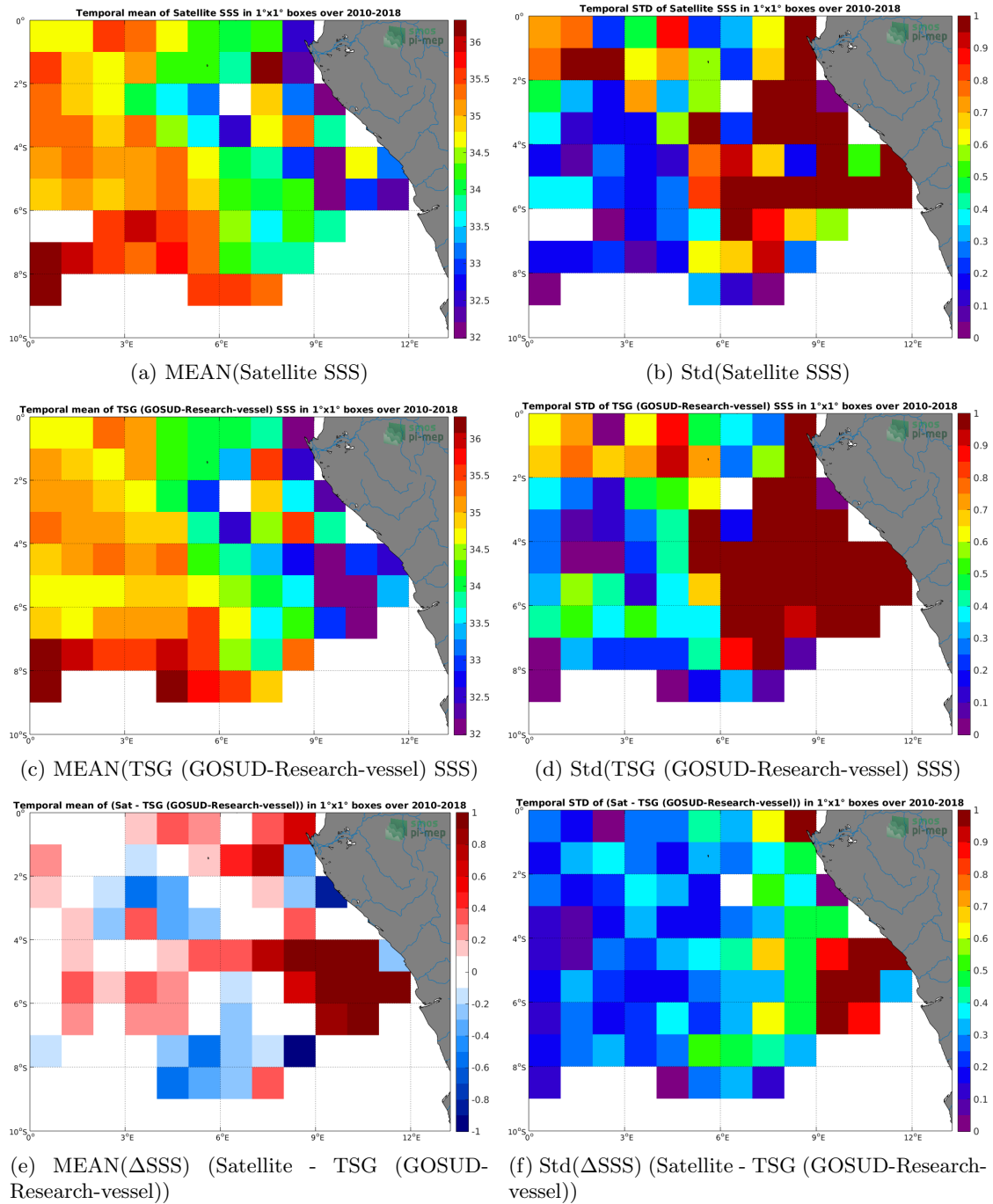
Figure 6: Temporal mean (left) and Std (right) of SSS from SMOS SSS L3 v4 - 9 Days (CATDS-CECOS-LOCEAN) (top), TSG (GOSUD-Research-vessel) (middle), and of \Delta SSS (Satellite - TSG (GOSUD-Research-vessel)). Only match-up pairs are used to generate these maps.
