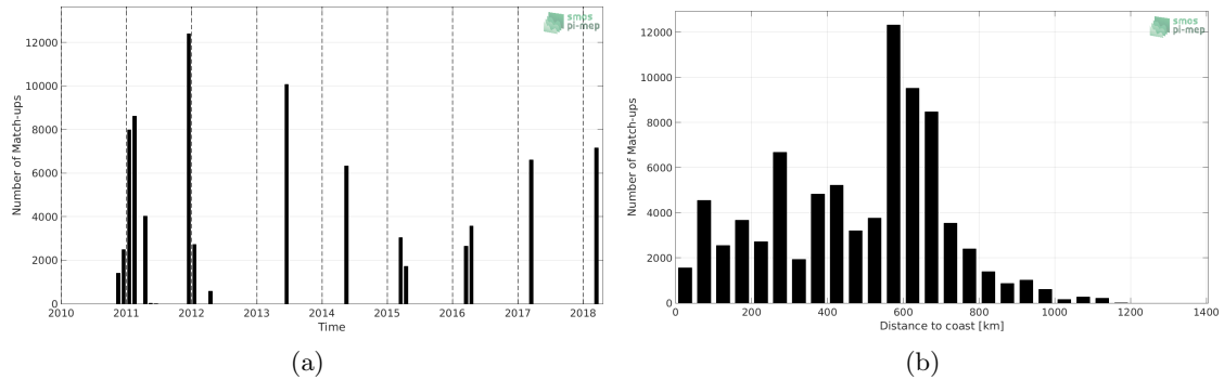
Figure 1: Number of match-ups between TSG (GOSUD-Research-vessel) and SMOS SSS L3 v4 - 9 Days (CATDS-CECOS-LOCEAN) SSS as a function of time (a) and as function of the distance to coast (b) over the Congo river plume Pi-MEP region and for the full satellite product period.
