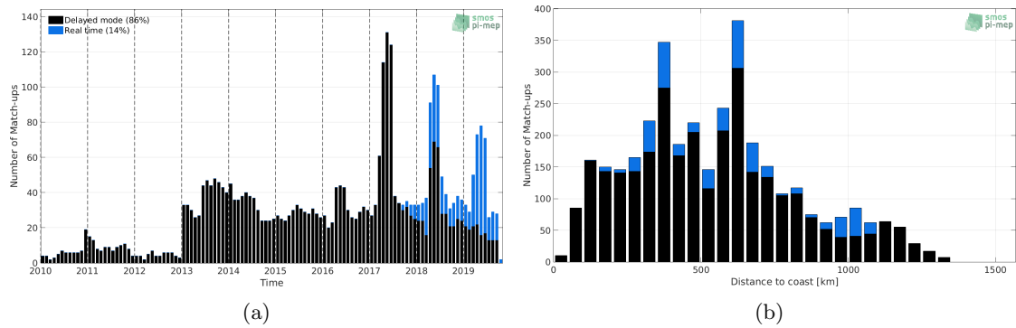
Figure 1: Number of match-ups between Argo and SMOS SSS L3 v4 - 9 Days (CATDS-CECOS-LOCEAN) SSS as a function of time (a) and as function of the distance to coast (b) over the Congo river plume Pi-MEP region and for the full satellite product period.
