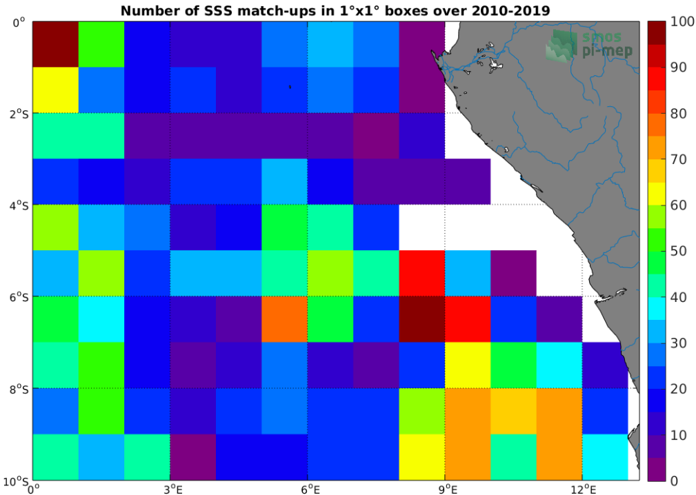
Figure 4: Number of SSS match-ups between Argo SSS and the SMOS SSS L3 v4 - 9 Days (CATDS-CECOS-LOCEAN) SSS product for the Congo river plume Pi-MEP region over 1°x1° boxes and for the full satellite product period.
