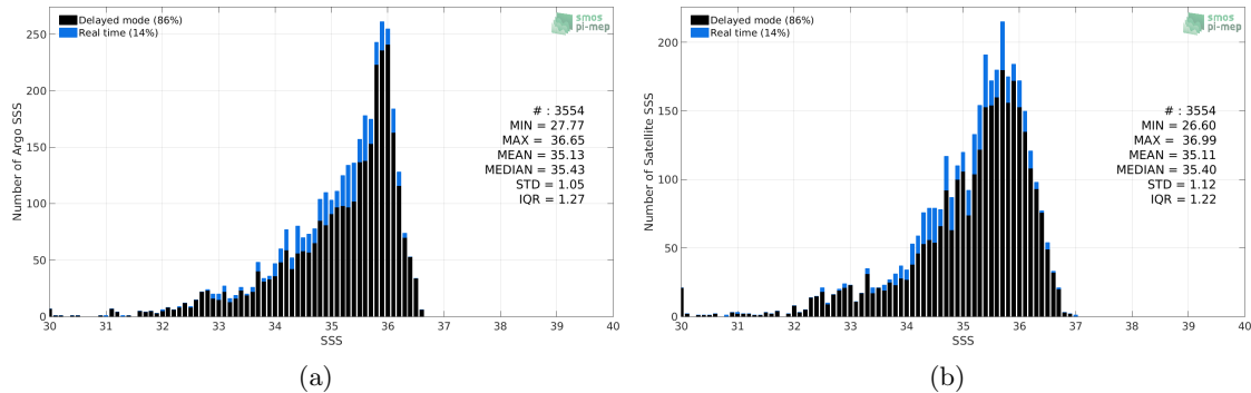
Figure 2: Histograms of SSS from Argo (a) and SMOS SSS L3 v4 - 9 Days (CATDS-CECOS-LOCEAN) (b) considering all match-up pairs per bins of 0.1 over the Congo river plume Pi-MEP region and for the full satellite product period.
