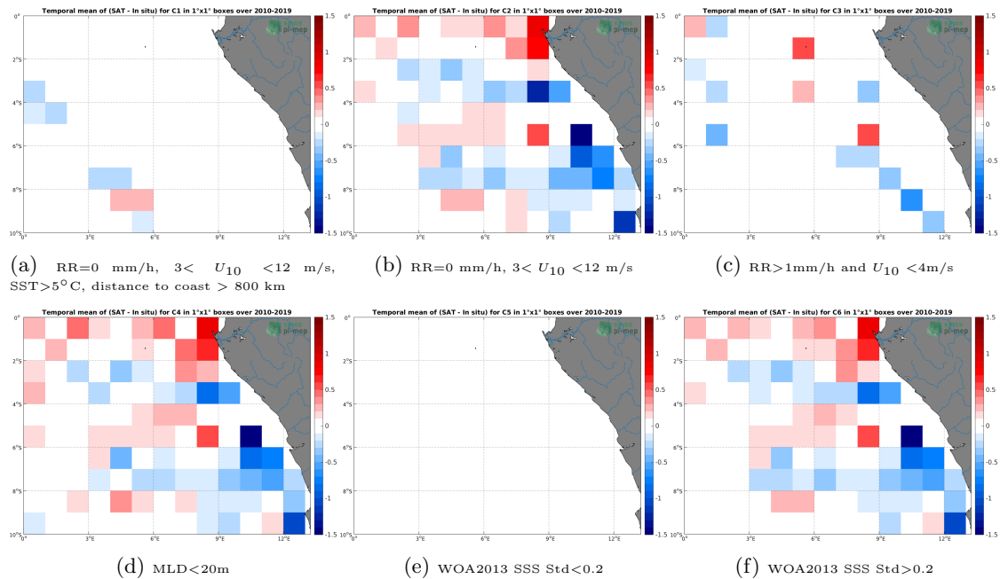
Figure 12: Temporal mean gridded over spatial boxes of size 1^\circ \times 1^\circ of \Delta SSS (SMOS SSS L3 v4 - 9 Days (CATDS-CECOS-LOCEAN) - Argo) for 6 different subdatasets corresponding to:RR=0 mm/h, 3 < U_{10} < 12 m/s, SST >5^\circ C, distance to coast > 800 km (a), RR=0 mm/h, 3 < U_{10} < 12 m/s (b), RR >1 mm/h and U_{10} < 4 m/s (c),MLD <20 m (d),WOA2013 SSS Std <0.2 (e),WOA2013 SSS Std >0.2 (f).
