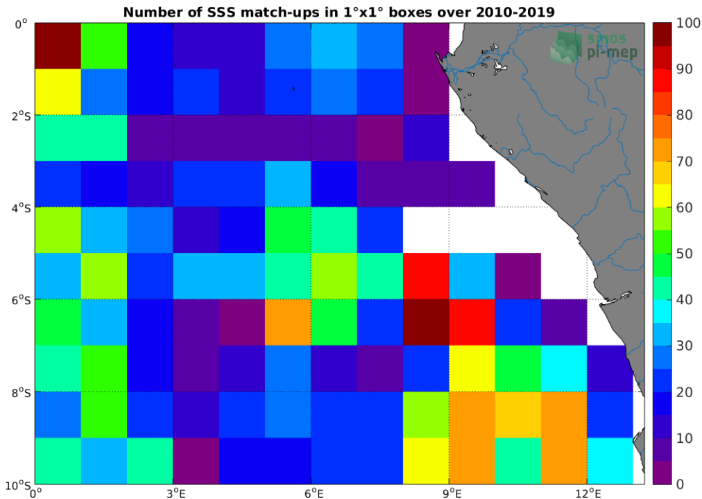
Figure 4: Number of SSS match-ups between Argo SSS and the SMOS-L3-CATDS-CECOS-LOCEAN-V4-9DAYS-25KM SSS product for the Congo river plume Pi-MEP region over 1°x1° boxes and for the full satellite product period.
