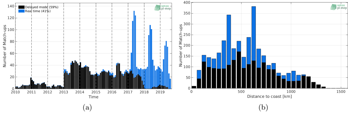
Figure 1: Number of match-ups between Argo and SMOS-L3-CATDS-CECOS-LOCEAN-V4-9DAYS-25KM SSS as a function of time (a) and as function of the distance to coast (b) over the Congo river plume Pi-MEP region and for the full satellite product period.
