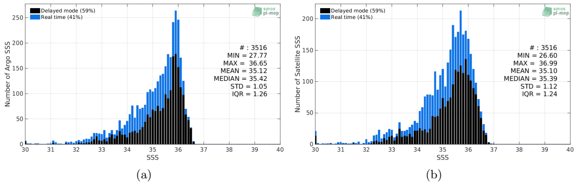
Figure 2: Histograms of SSS from Argo (a) and SMOS-L3-CATDS-CECOS-LOCEAN-V4-9DAYS-25KM (b) considering all match-up pairs per bins of 0.1 over the Congo river plume Pi-MEP region and for the full satellite product period.
