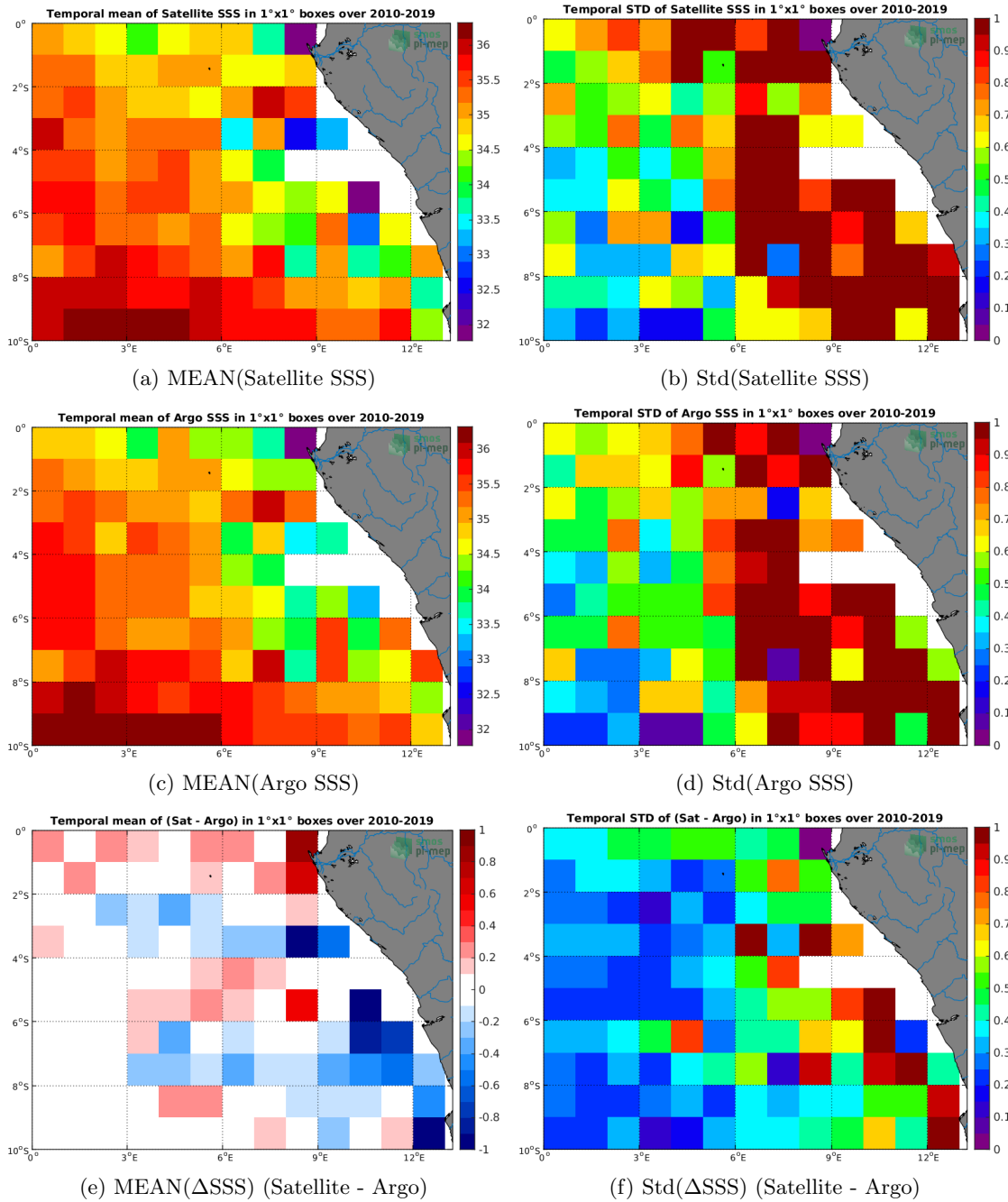
Figure 6: Temporal mean (left) and Std (right) of SSS from SMOS-L3-CATDS-CECOS-LOCEAN-V4-9DAYS-25KM (top), Argo (middle), and of \Delta SSS (Satellite - Argo). Only match-up pairs are used to generate these maps.
