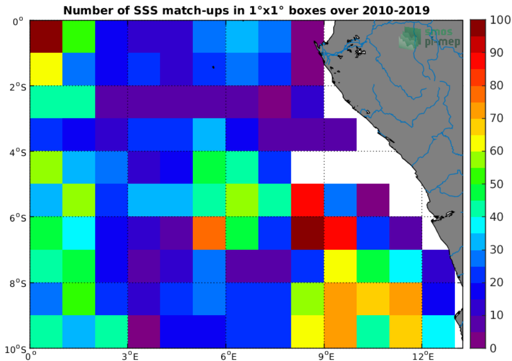
Figure 4: Number of SSS match-ups between Argo SSS and the SMOS-L3-CATDS-CECOS-LOCEAN-V4-9DAYS-25KM SSS product for the Congo river plume Pi-MEP region over 1^\circ \times 1^\circ boxes and for the full satellite product period.
