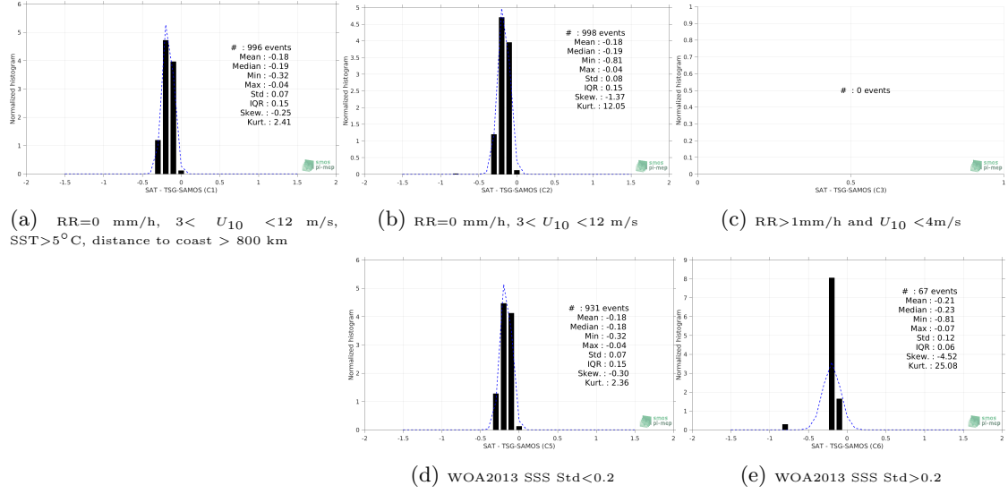
Figure 13: Normalized histogram of \Delta SSS (SMOS-L3-CATDS-CECOS-LOCEAN-V4-18DAYS-25KM - TSG-SAMOS) for 5 different subdatasets corresponding to: RR=0 mm/h, 3 < U_{10} < 12 m/s, SST>5°C, distance to coast > 800 km (a), RR=0 mm/h, 3 < U_{10} < 12 m/s (b), RR>1mm/h and U_{10} < 4 m/s (c), WOA2013 SSS Std<0.2 (d), WOA2013 SSS Std>0.2 (e).
