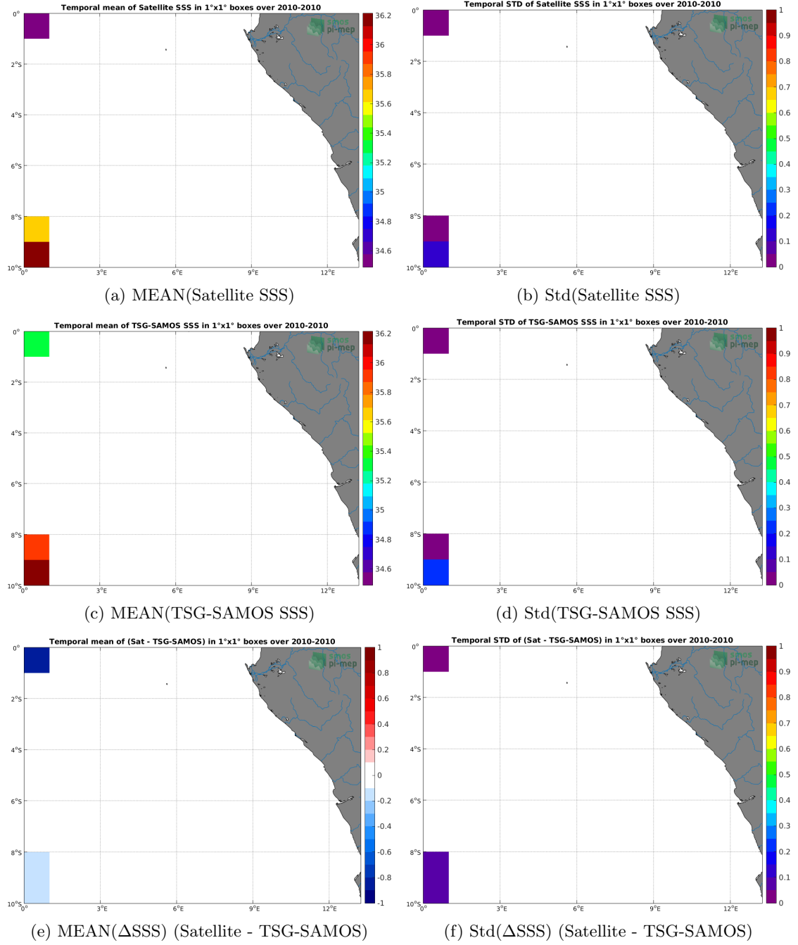
Figure 6: Temporal mean (left) and Std (right) of SSS from SMOS-L3-CATDS-CECOS-LOCEAN-V4-18DAYS-25KM (top), TSG-SAMOS (middle), and of \Delta SSS (Satellite - TSG-SAMOS). Only match-up pairs are used to generate these maps.
