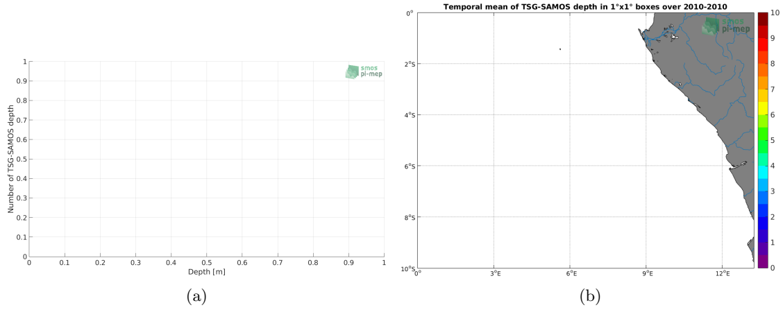
Figure 3: Histograms of the depth of the upper level SSS measurements from TSG-SAMOS in the Match-up DataBase for the Congo river plume Pi-MEP region (a) and temporal mean spatial distribution of pressure of the in situ SSS data over 1^\circ \times 1^\circ boxes and for the full satellite product period (b).
