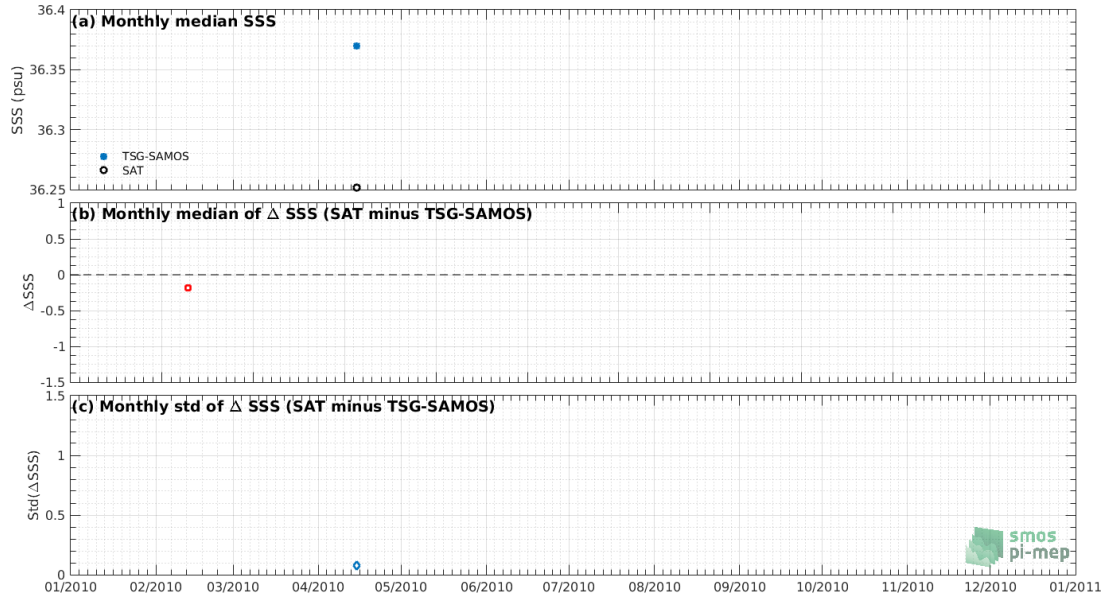
Figure 7: Time series of the monthly median SSS (top), median of \Delta SSS (Satellite - TSG-SAMOS) and Std of \Delta SSS (Satellite - TSG-SAMOS) over the Congo river plume Pi-MEP region considering all match-ups collected by the Pi-MEP.
