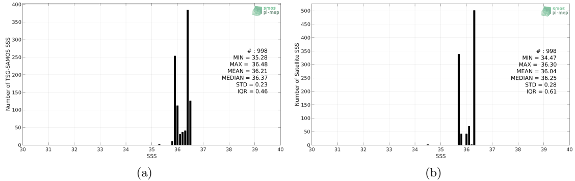
Figure 2: Histograms of SSS from TSG-SAMOS (a) and SMOS-L3-CATDS-CECOS-LOCEAN-V4-18DAYS-25KM (b) considering all match-up pairs per bins of 0.1 over the Congo river plume Pi-MEP region and for the full satellite product period.
