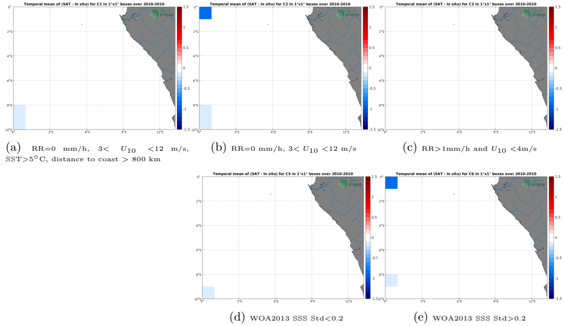
Figure 12: Temporal mean gridded over spatial boxes of size 1^{\circ}\times 1^{\circ} of \Delta\text{SSS} (SMOS-L3-CATDS-CECOS-LOCEAN-V4-18DAYS-25KM - TSG-SAMOS) for 5 different subdatasets corresponding to: RR=0 mm/h, 3 < U_{10} < 12 m/s, SST >5^{\circ}\text{C} , distance to coast > 800 km (a), RR=0 mm/h, 3 < U_{10} < 12 m/s (b), RR >1 mm/h and U_{10} < 4 m/s (c), WOA2013 SSS Std <0.2 (d), WOA2013 SSS Std >0.2 (e).
