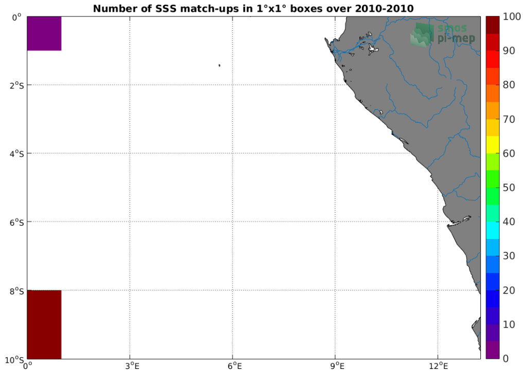
Figure 4: Number of SSS match-ups between TSG-SAMOS SSS and the SMOS-L3-CATDS-CECOS-LOCEAN-V4-18DAYS-25KM SSS product for the Congo river plume Pi-MEP region over 1^\circ \times 1^\circ boxes and for the full satellite product period.
