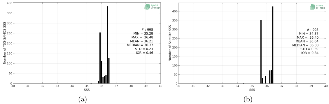
Figure 2: Histograms of SSS from TSG-SAMOS (a) and SMOS-L3-CATDS-CECOS-LOCEAN-V3-9DAYS-25KM (b) considering all match-up pairs per bins of 0.1 over the Congo river plume Pi-MEP region and for the full satellite product period.
