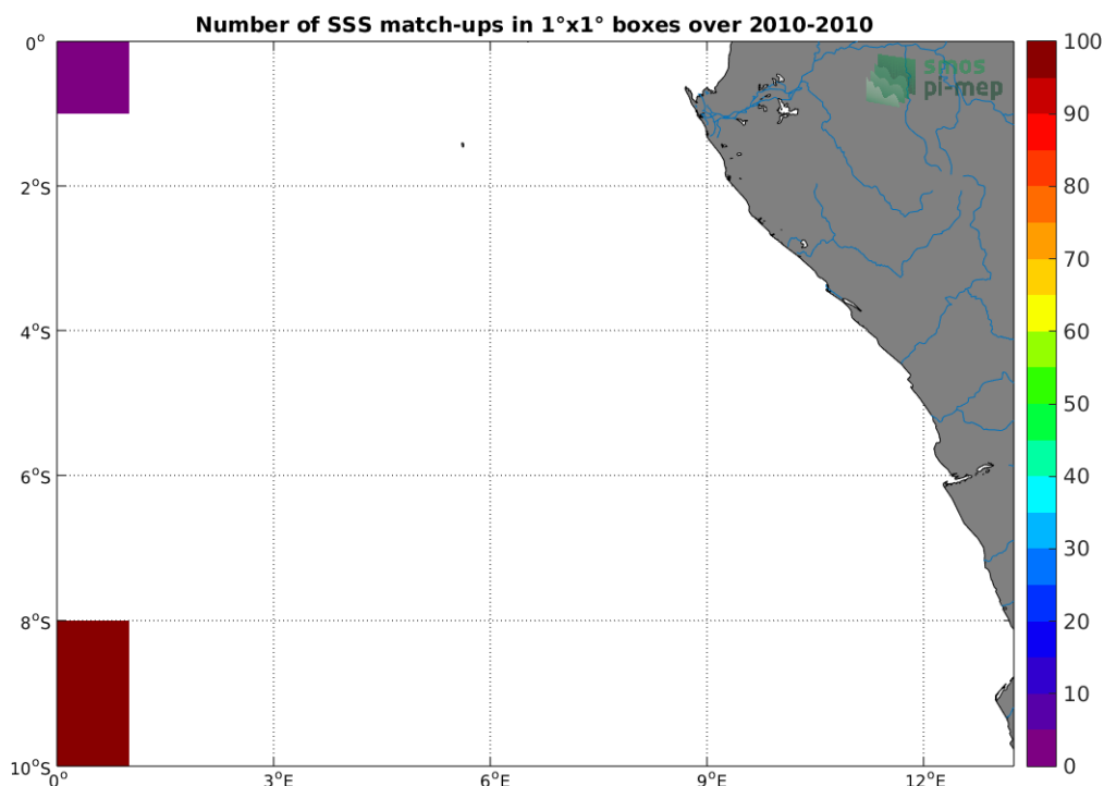
Figure 4: Number of SSS match-ups between TSG-SAMOS SSS and the SMOS-L3-CATDS-CECOS-LOCEAN-V3-9DAYS-25KM SSS product for the Congo river plume Pi-MEP region over 1^\circ \times 1^\circ boxes and for the full satellite product period.
