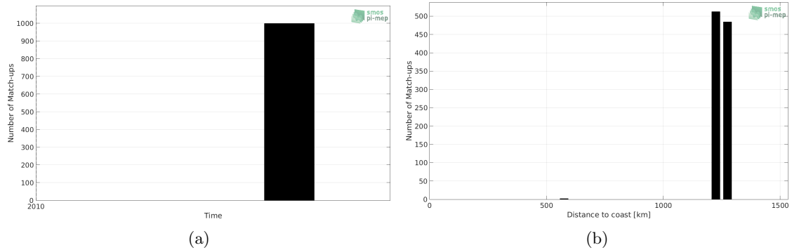
Figure 1: Number of match-ups between TSG-SAMOS and SMOS-L3-CATDS-CECOS-LOCEAN-V3-9DAYS-25KM SSS as a function of time (a) and as function of the distance to coast (b) over the Congo river plume Pi-MEP region and for the full satellite product period.
