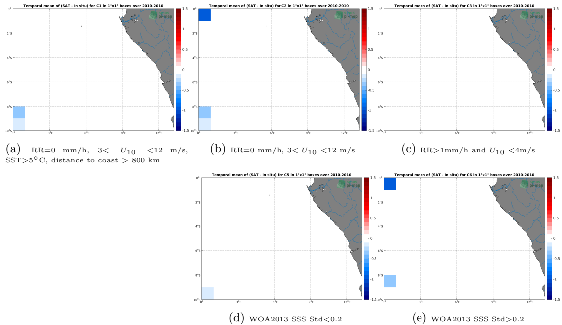
Figure 12: Temporal mean gridded over spatial boxes of size 1^\circ \times 1^\circ of \Delta SSS (SMOS-L3-CATDS-CECOS-LOCEAN-V3-9DAYS-25KM - TSG-SAMOS) for 5 different subdatasets corresponding to:RR=0 mm/h, 3 < U_{10} < 12 m/s, SST > 5^\circ\text{C} , distance to coast > 800 km (a), RR=0 mm/h, 3 < U_{10} < 12 m/s (b), RR > 1\text{mm/h} and U_{10} < 4\text{m/s} (c), WOA2013 SSS Std < 0.2 (d), WOA2013 SSS Std > 0.2 (e).
