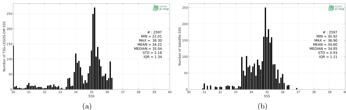
Figure 2: Histograms of SSS from TSG-LEGOS-DM (a) and SMOS-L3-CATDS-CECOS-LOCEAN-V3-9DAYS-25KM (b) considering all match-up pairs per bins of 0.1 over the Congo river plume Pi-MEP region and for the full satellite product period.
