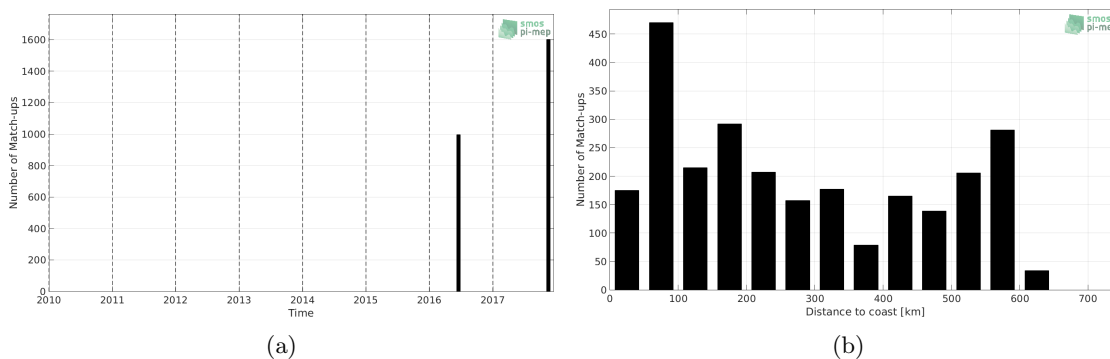
Figure 1: Number of match-ups between TSG-LEGOS-DM and SMOS-L3-CATDS-CECOS-LOCEAN-V3-9DAYS-25KM SSS as a function of time (a) and as function of the distance to coast (b) over the Congo river plume Pi-MEP region and for the full satellite product period.
