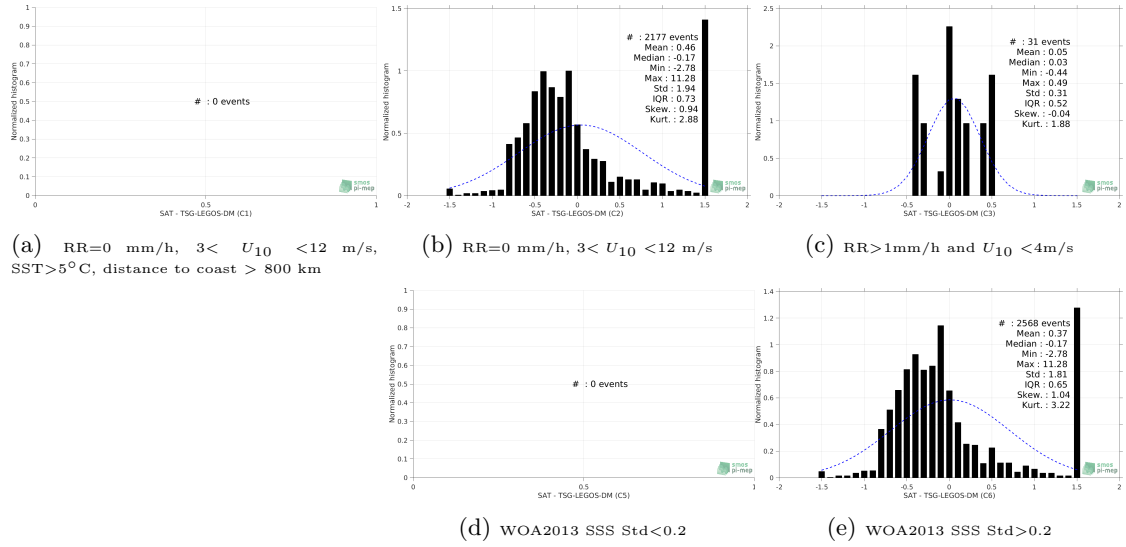
Figure 13: Normalized histogram of \Delta SSS (SMOS-L3-CATDS-CECOS-LOCEAN-V3-9DAYS-25KM - TSG-LEGOS-DM) for 5 different subdatasets corresponding to: RR=0 mm/h, 3 < U_{10} < 12 m/s, SST>5°C, distance to coast > 800 km (a), RR=0 mm/h, 3 < U_{10} < 12 m/s (b), RR>1mm/h and U_{10} < 4 m/s (c), WOA2013 SSS Std<0.2 (d), WOA2013 SSS Std>0.2 (e).
