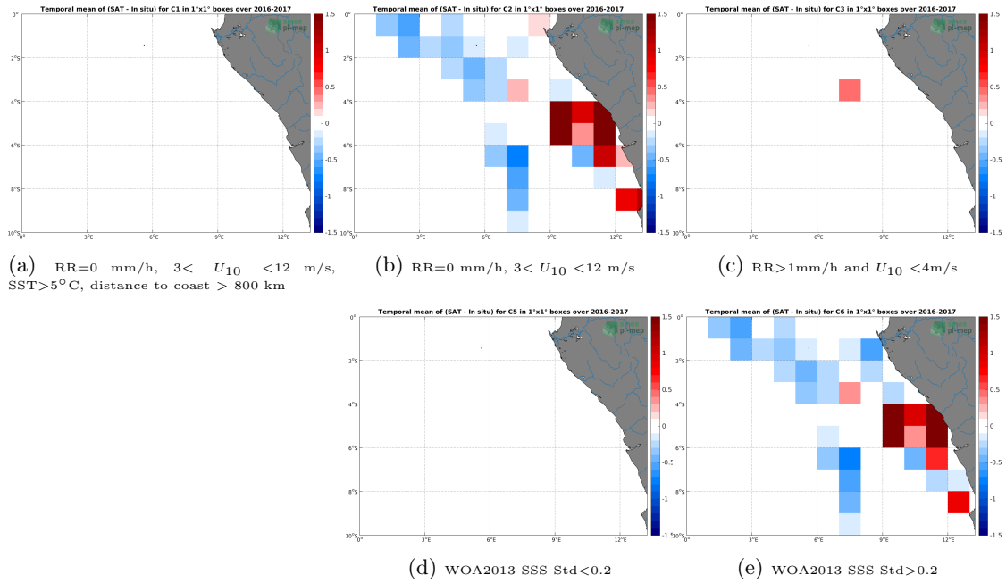
Figure 12: Temporal mean gridded over spatial boxes of size 1^\circ \times 1^\circ of \Delta SSS (SMOS-L3-CATDS-CECOS-LOCEAN-V3-9DAYS-25KM - TSG-LEGOS-DM) for 5 different subdatasets corresponding to:RR=0 mm/h, 3 < U_{10} < 12 m/s, SST >5^\circ C, distance to coast > 800 km (a), RR=0 mm/h, 3 < U_{10} < 12 m/s (b), RR >1 mm/h and U_{10} < 4 m/s (c), WOA2013 SSS Std <0.2 (d), WOA2013 SSS Std >0.2 (e).
