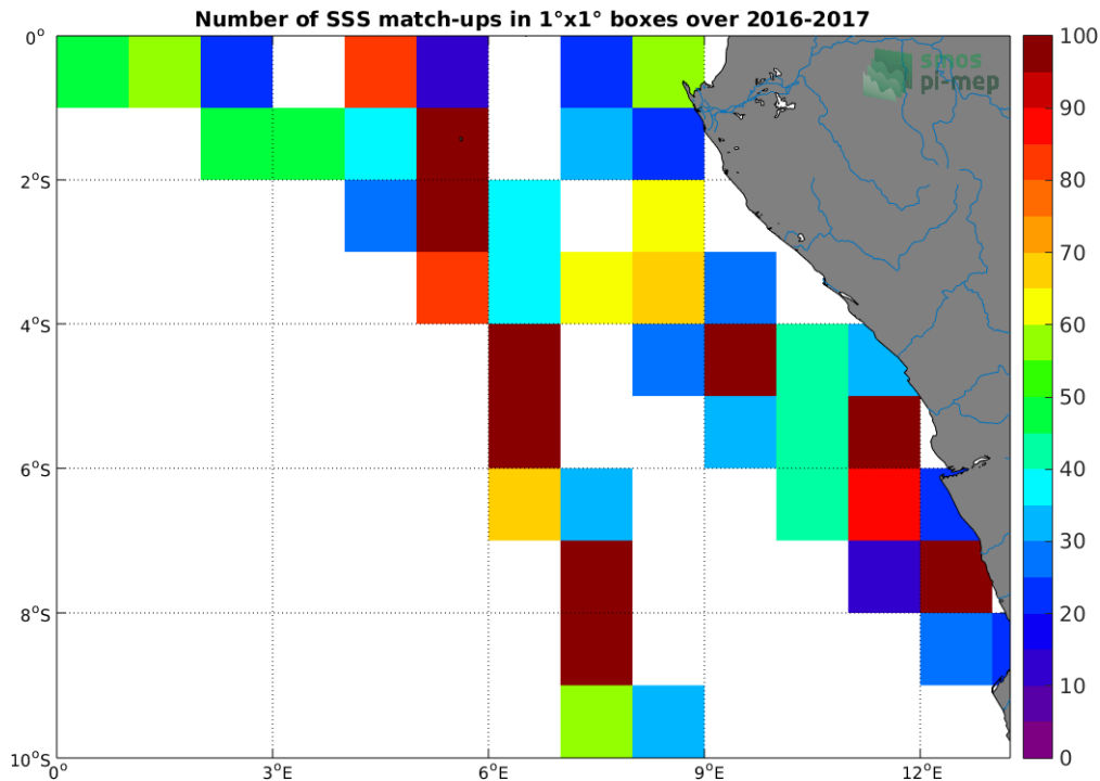
Figure 4: Number of SSS match-ups between TSG-LEGOS-DM SSS and the SMOS-L3-CATDS-CECOS-LOCEAN-V3-9DAYS-25KM SSS product for the Congo river plume Pi-MEP region over 1^\circ \times 1^\circ boxes and for the full satellite product period.
