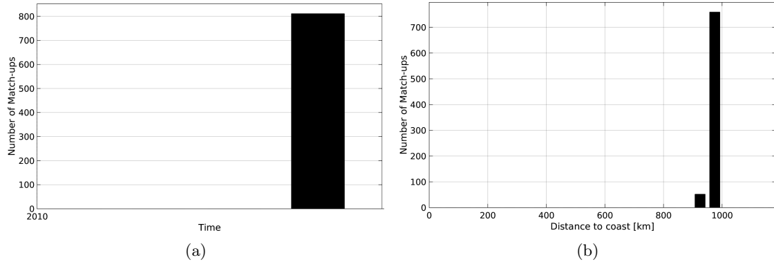
Figure 1: Number of match-ups between TSG-SAMOS and SMOS-L3-CATDS-CECOS-LOCEAN-V2.1-9DAYS-25KM SSS as a function of time (a) and as function of the distance to coast (b) over the Congo river plume Pi-MEP region and for the full satellite product period.
