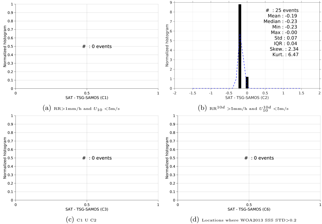
Figure 13: Normalized histogram of \Delta\text{SSS} (SMOS-L3-CATDS-CECOS-LOCEAN-V2.1-9DAYS-25KM - TSG-SAMOS) for 6 different subdatasets corresponding to: RR > 1\text{mm/h} and U_{10} < 5\text{m/s} (a), RR^{10d} > 5\text{mm/h} and U_{10}^{10d} < 5\text{m/s} (b), C1 U C2 (c), Locations where WOA2013 SSS STD > 0.2 (d).
