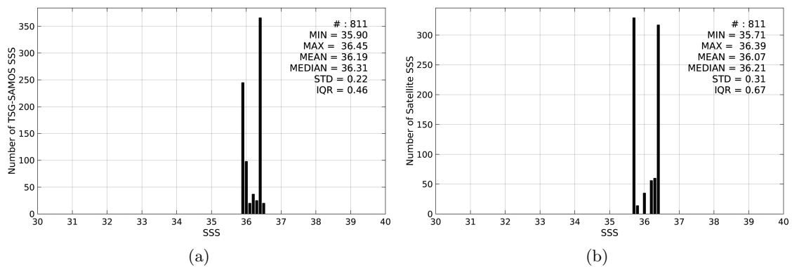
Figure 2: Histograms of SSS from TSG-SAMOS (a) and SMOS-L3-CATDS-CECOS-LOCEAN-V2.1-9DAYS-25KM (b) considering all match-up pairs per bins of 0.1 over the Congo river plume Pi-MEP region and for the full satellite product period.
