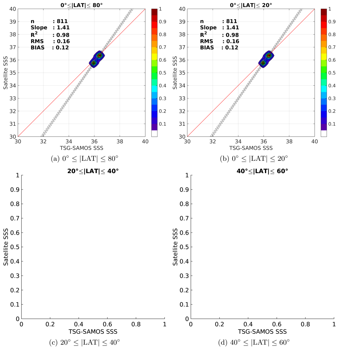
Figure 9: Contour maps of the concentration of SMOS-L3-CATDS-CECOS-LOCEAN-V2.1-9DAYS-25KM SSS (y-axis) versus TSG-SAMOS SSS (x-axis) at match-up pairs for different latitude bands. For each plot, the red line shows x=y . The black thin and dashed lines indicate a linear fit through the data cloud and the \pm 95\% confidence levels, respectively. The number match-up pairs n , the slope and R^2 coefficient of the linear fit, the root mean square (RMS) and the mean bias between satellite and in situ data are indicated for each latitude band in each plots.
