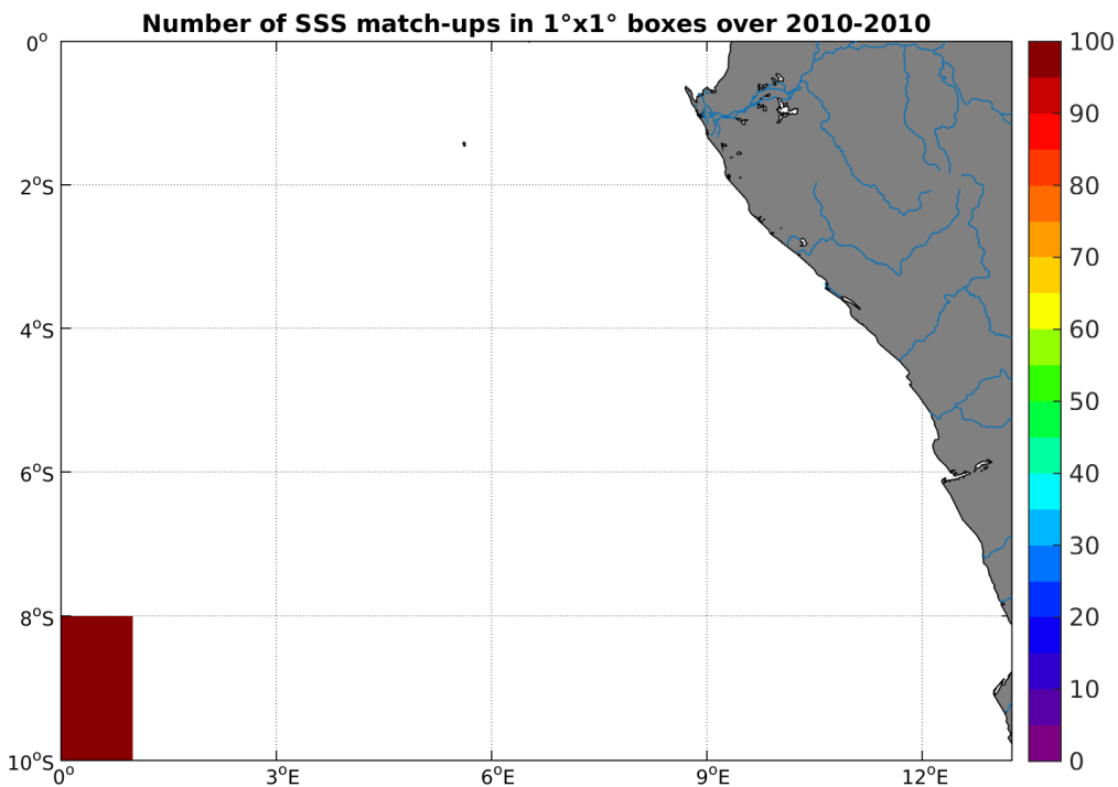
Figure 4: Number of SSS match-ups between TSG-SAMOS SSS and the SMOS-L3-CATDS-CECOS-LOCEAN-V2.1-9DAYS-25KM SSS product for the Congo river plume Pi-MEP region over 1^\circ \times 1^\circ boxes and for the full satellite product period.
