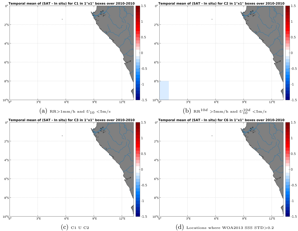
Figure 12: Temporal mean gridded over spatial boxes of size 1^\circ \times 1^\circ of \Delta SSS (SMOS-L3-CATDS-CECOS-LOCEAN-V2.1-9DAYS-25KM - TSG-SAMOS) for 4 different subdatasets corresponding to: RR > 1\text{mm/h} and U_{10} < 5\text{m/s} (a), RR^{10d} > 5\text{mm/h} and U_{10}^{10d} < 5\text{m/s} (b), C1 \cup C2 (c), Locations where WOA2013 SSS STD > 0.2 (d).
