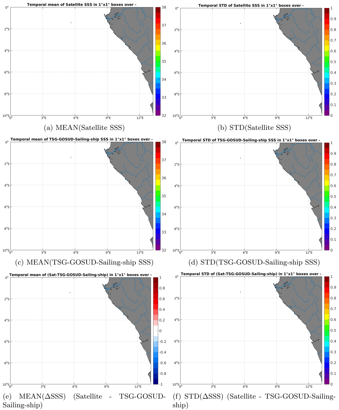
Figure 6: Temporal mean (left) and STD (right) of SSS from SMOS-L3-CATDS-CECOS-LOCEAN-V2.1-9DAYS-25KM (top), TSG-GOSUD-Sailing-ship (middle), and of \Delta SSS (Satellite - TSG-GOSUD-Sailing-ship). Only match-up pairs are used to generate these maps.
