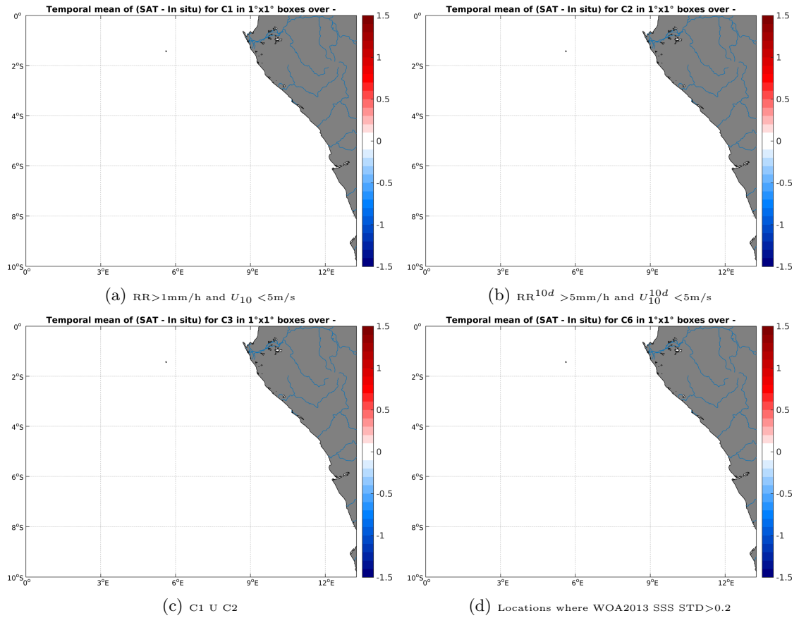
Figure 12: Temporal mean gridded over spatial boxes of size 1^\circ \times 1^\circ of \Delta SSS (SMOS-L3-CATDS-CECOS-LOCEAN-V2.1-9DAYS-25KM - TSG-GOSUD-Sailing-ship) for 4 different subdatasets corresponding to:RR >1 mm/h and U_{10} < 5 m/s (a), RR ^{10d} > 5 mm/h and U_{10}^{10d} < 5 m/s (b), C1 U C2 (c),Locations where WOA2013 SSS STD >0.2 (d).
