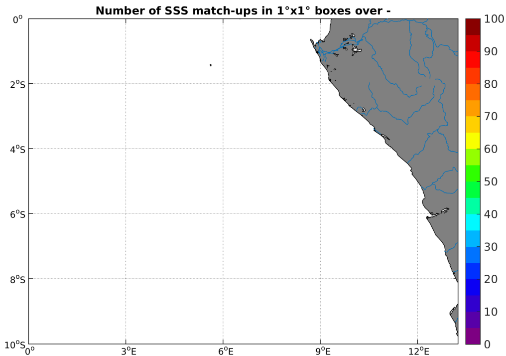
Figure 4: Number of SSS match-ups between TSG-GOSUD-Sailing-ship SSS and the SMOS-L3-CATDS-CECOS-LOCEAN-V2.1-9DAYS-25KM SSS product for the Congo river plume Pi-MEP region over 1^{\circ} \times 1^{\circ} boxes and for the full satellite product period.
