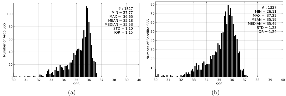
Figure 2: Histograms of SSS from Argo (a) and SMOS-L3-CATDS-CECOS-LOCEAN-V2.1-9DAYS-25KM (b) considering all match-up pairs per bins of 0.1 over the Congo river plume Pi-MEP region and for the full satellite product period.
