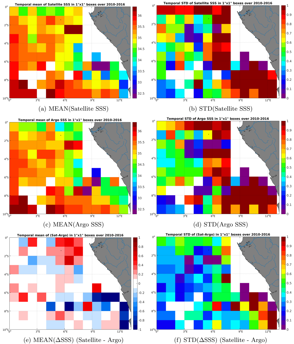
Figure 6: Temporal mean (left) and STD (right) of SSS from SMOS-L3-CATDS-CECOS-LOCEAN-V2.1-9DAYS-25KM (top), Argo (middle), and of \Delta SSS (Satellite - Argo). Only match-up pairs are used to generate these maps.
