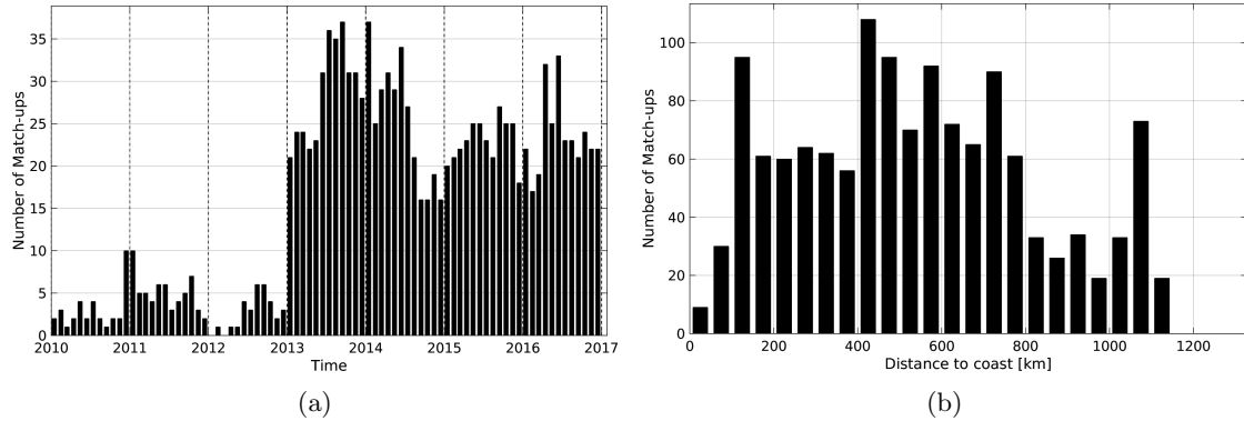
Figure 1: Number of match-ups between Argo and SMOS-L3-CATDS-CECOS-LOCEAN-V2.1-9DAYS-25KM SSS as a function of time (a) and as function of the distance to coast (b) over the Congo river plume Pi-MEP region and for the full satellite product period.
