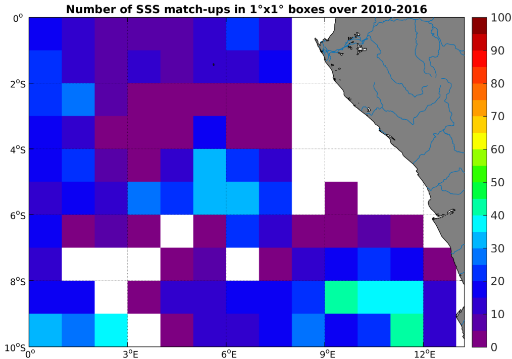
Figure 4: Number of SSS match-ups between Argo SSS and the SMOS-L3-CATDS-CECOS-LOCEAN-V2.1-9DAYS-25KM SSS product for the Congo river plume Pi-MEP region over 1°x1° boxes and for the full satellite product period.
