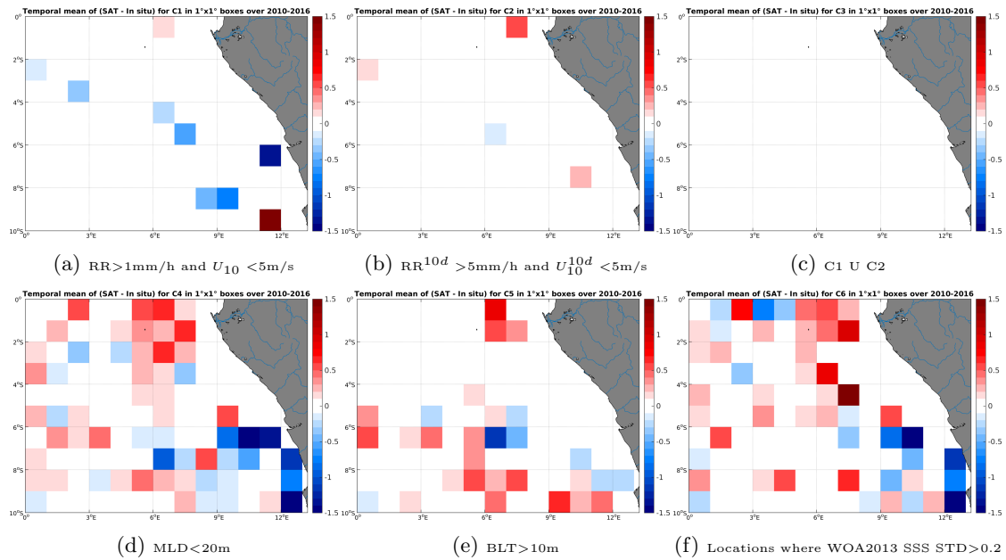
Figure 12: Temporal mean gridded over spatial boxes of size 1^\circ \times 1^\circ of \Delta SSS (SMOS-L3-CATDS-CECOS-LOCEAN-V2.1-9DAYS-25KM - Argo) for 6 different subdatasets corresponding to:RR >1 mm/h and U_{10} < 5 m/s (a), RR 10d > 5 mm/h and U_{10}^{10d} < 5 m/s (b), C1 U C2 (c),MLD <20 m (d),BLT >10 m (e),Locations where WOA2013 SSS STD >0.2 (f).
