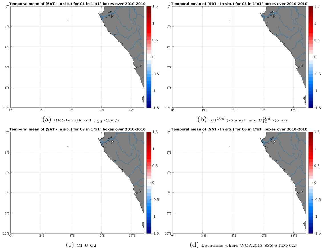
Figure 12: Temporal mean gridded over spatial boxes of size 1^\circ \times 1^\circ of \Delta SSS (SMOS-L3-CATDS-CECOS-LOCEAN-V2-9DAYS-25KM - TSG-SAMOS) for 4 different subdatasets corresponding to: RR > 1\text{mm/h} and U_{10} < 5\text{m/s} (a), RR^{10d} > 5\text{mm/h} and U_{10}^{10d} < 5\text{m/s} (b), C1 \cup C2 (c), Locations where WOA2013 SSS STD > 0.2 (d).
