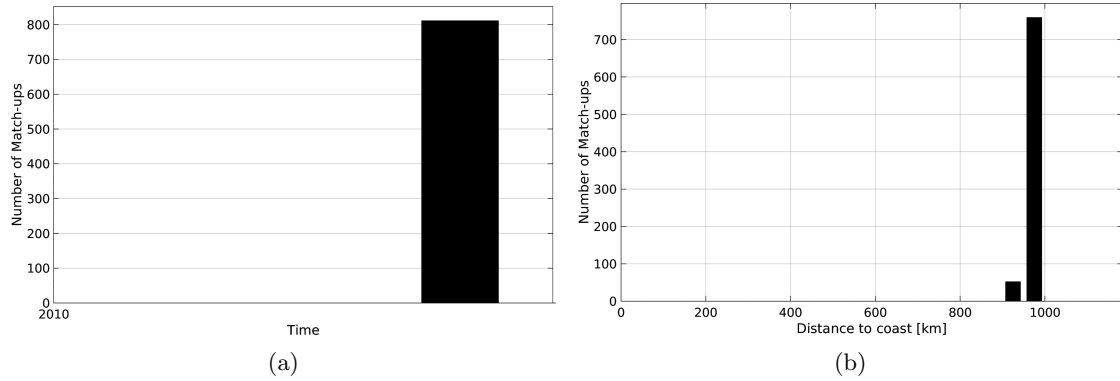
Figure 1: Number of match-ups between TSG-SAMOS and SMOS-L3-CATDS-CECOS-LOCEAN-V2-9DAYS-25KM SSS as a function of time (a) and as function of the distance to coast (b) over the Congo river plume Pi-MEP region and for the full satellite product period.
