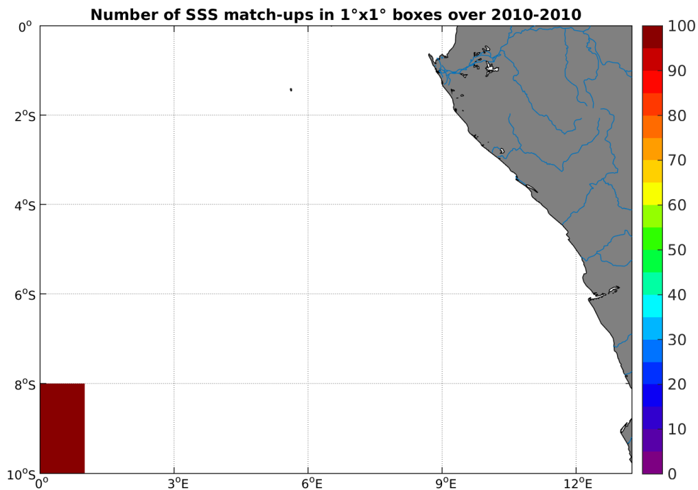
Figure 4: Number of SSS match-ups between TSG-SAMOS SSS and the SMOS-L3-CATDS-CECOS-LOCEAN-V2-9DAYS-25KM SSS product for the Congo river plume Pi-MEP region over 1^\circ \times 1^\circ boxes and for the full satellite product period.
