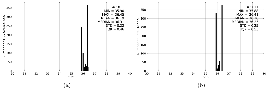
Figure 2: Histograms of SSS from TSG-SAMOS (a) and SMOS-L3-CATDS-CECOS-LOCEAN-V2-9DAYS-25KM (b) considering all match-up pairs per bins of 0.1 over the Congo river plume Pi-MEP region and for the full satellite product period.
