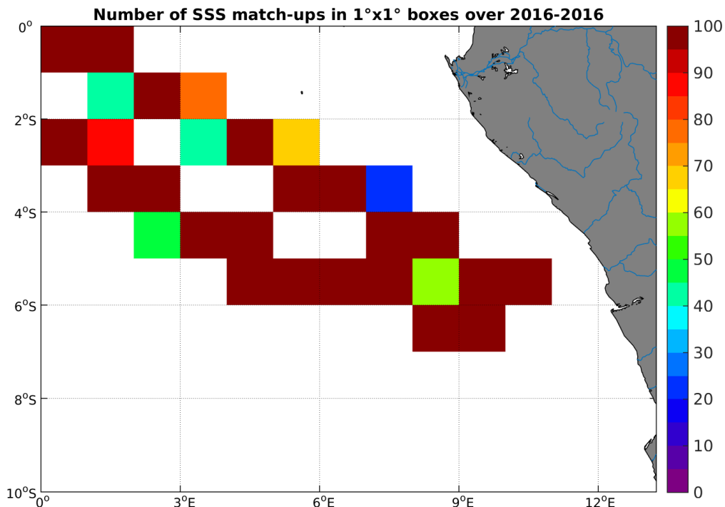
Figure 4: Number of SSS match-ups between TSG-GOSUD-Sailing-ship SSS and the SMOS-L3-CATDS-CECOS-LOCEAN-V2-9DAYS-25KM SSS product for the Congo river plume Pi-MEP region over 1^\circ \times 1^\circ boxes and for the full satellite product period.
