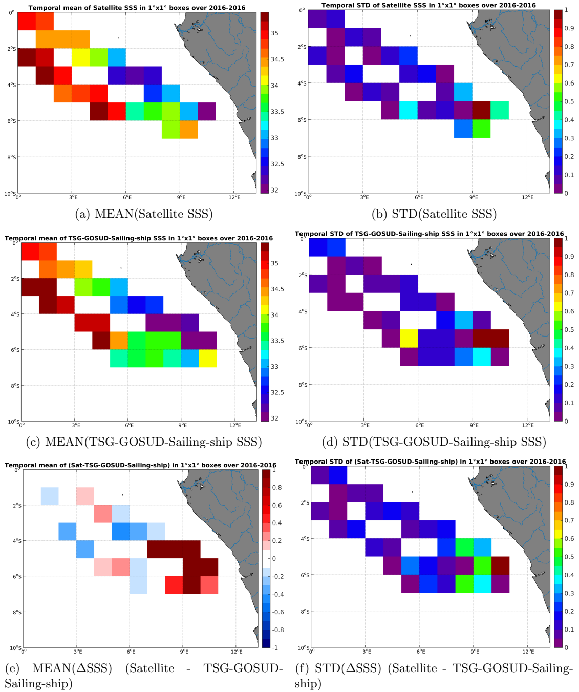
Figure 6: Temporal mean (left) and STD (right) of SSS from SMOS-L3-CATDS-CECOS-LOCEAN-V2-9DAYS-25KM (top), TSG-GOSUD-Sailing-ship (middle), and of \Delta SSS (Satellite - TSG-GOSUD-Sailing-ship). Only match-up pairs are used to generate these maps.
