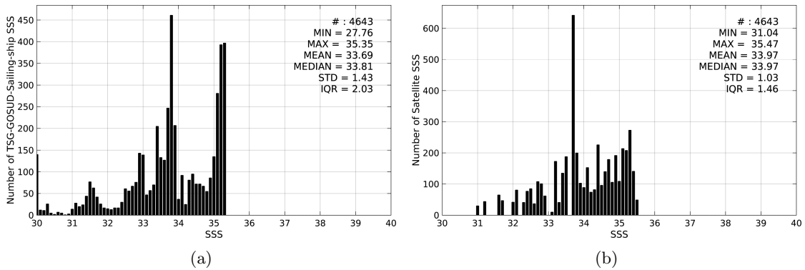
Figure 2: Histograms of SSS from TSG-GOSUD-Sailing-ship (a) and SMOS-L3-CATDS-CECOS-LOCEAN-V2-9DAYS-25KM (b) considering all match-up pairs per bins of 0.1 over the Congo river plume Pi-MEP region and for the full satellite product period.
