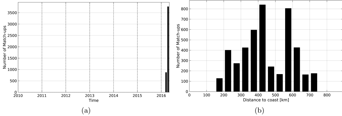
Figure 1: Number of match-ups between TSG-GOSUD-Sailing-ship and SMOS-L3-CATDS-CECOS-LOCEAN-V2-9DAYS-25KM SSS as a function of time (a) and as function of the distance to coast (b) over the Congo river plume Pi-MEP region and for the full satellite product period.
