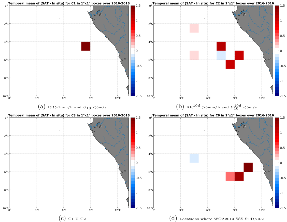
Figure 12: Temporal mean gridded over spatial boxes of size 1^\circ \times 1^\circ of \Delta SSS (SMOS-L3-CATDS-CECOS-LOCEAN-V2-9DAYS-25KM - TSG-GOSUD-Sailing-ship) for 4 different subdatasets corresponding to: RR > 1\text{mm/h} and U_{10} < 5\text{m/s} (a), RR^{10d} > 5\text{mm/h} and U_{10}^{10d} < 5\text{m/s} (b), C1 \cup C2 (c), Locations where WOA2013 SSS STD > 0.2 (d).
