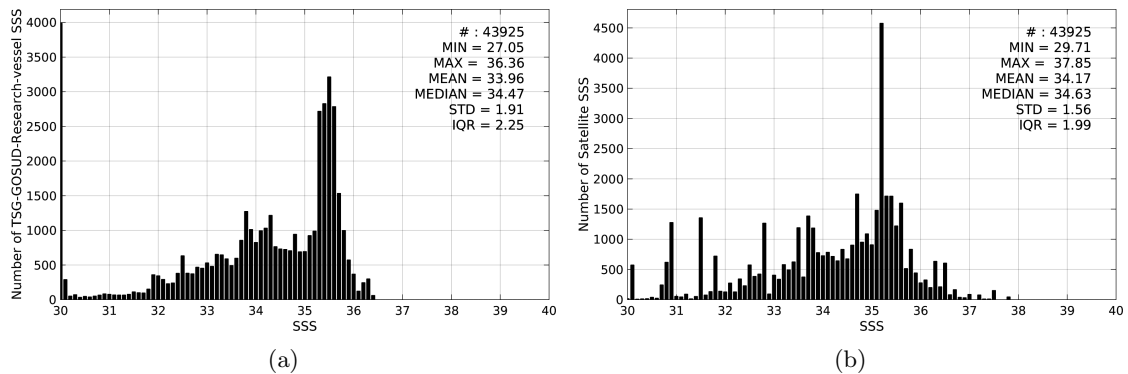
Figure 2: Histograms of SSS from TSG-GOSUD-Research-vessel (a) and SMOS-L3-CATDS-CECOS-LOCEAN-V2-9DAYS-25KM (b) considering all match-up pairs per bins of 0.1 over the Congo river plume Pi-MEP region and for the full satellite product period.
