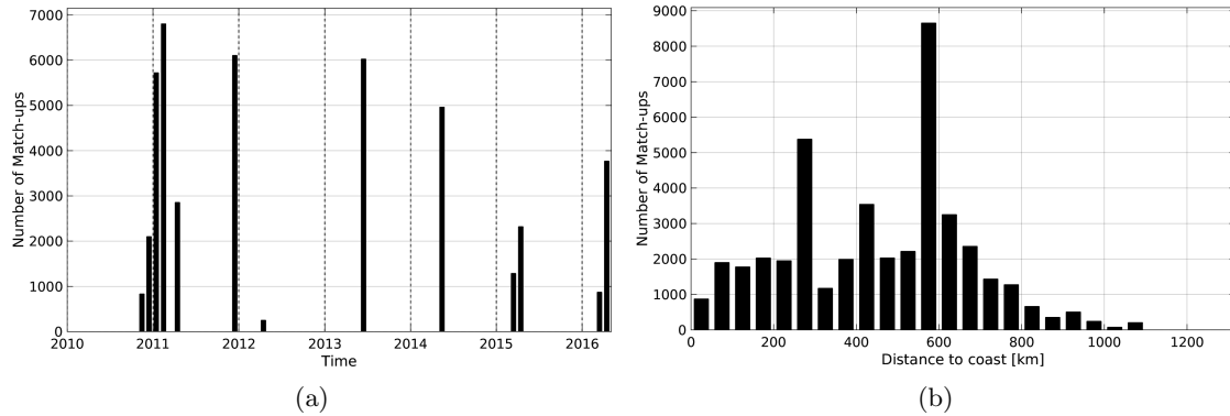
Figure 1: Number of match-ups between TSG-GOSUD-Research-vessel and SMOS-L3-CATDS-CECOS-LOCEAN-V2-9DAYS-25KM SSS as a function of time (a) and as function of the distance to coast (b) over the Congo river plume Pi-MEP region and for the full satellite product period.
