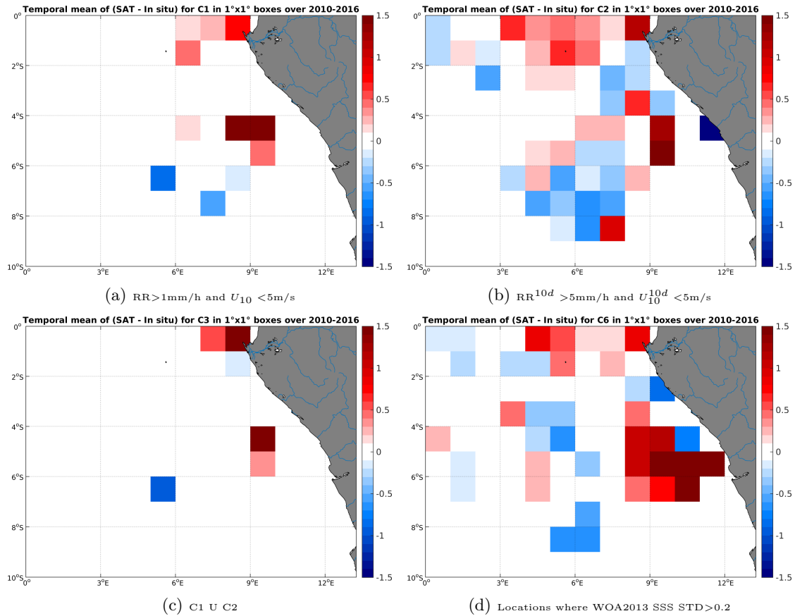
Figure 12: Temporal mean gridded over spatial boxes of size 1^\circ \times 1^\circ of \Delta SSS (SMOS-L3-CATDS-CECOS-LOCEAN-V2-9DAYS-25KM - TSG-GOSUD-Research-vessel) for 4 different subdatasets corresponding to: RR > 1\text{mm/h} and U_{10} < 5\text{m/s} (a), RR^{10d} > 5\text{mm/h} and U_{10}^{10d} < 5\text{m/s} (b), C1 \cup C2 (c), Locations where WOA2013 SSS STD > 0.2 (d).
