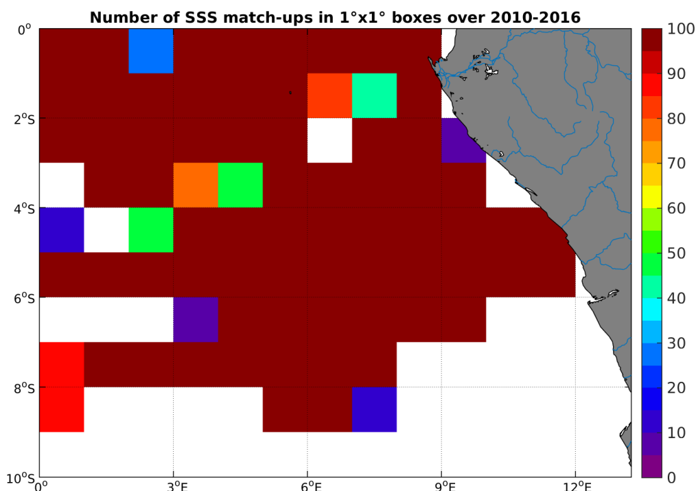
Figure 4: Number of SSS match-ups between TSG-GOSUD-Research-vessel SSS and the SMOS-L3-CATDS-CECOS-LOCEAN-V2-9DAYS-25KM SSS product for the Congo river plume Pi-MEP region over 1^\circ \times 1^\circ boxes and for the full satellite product period.
