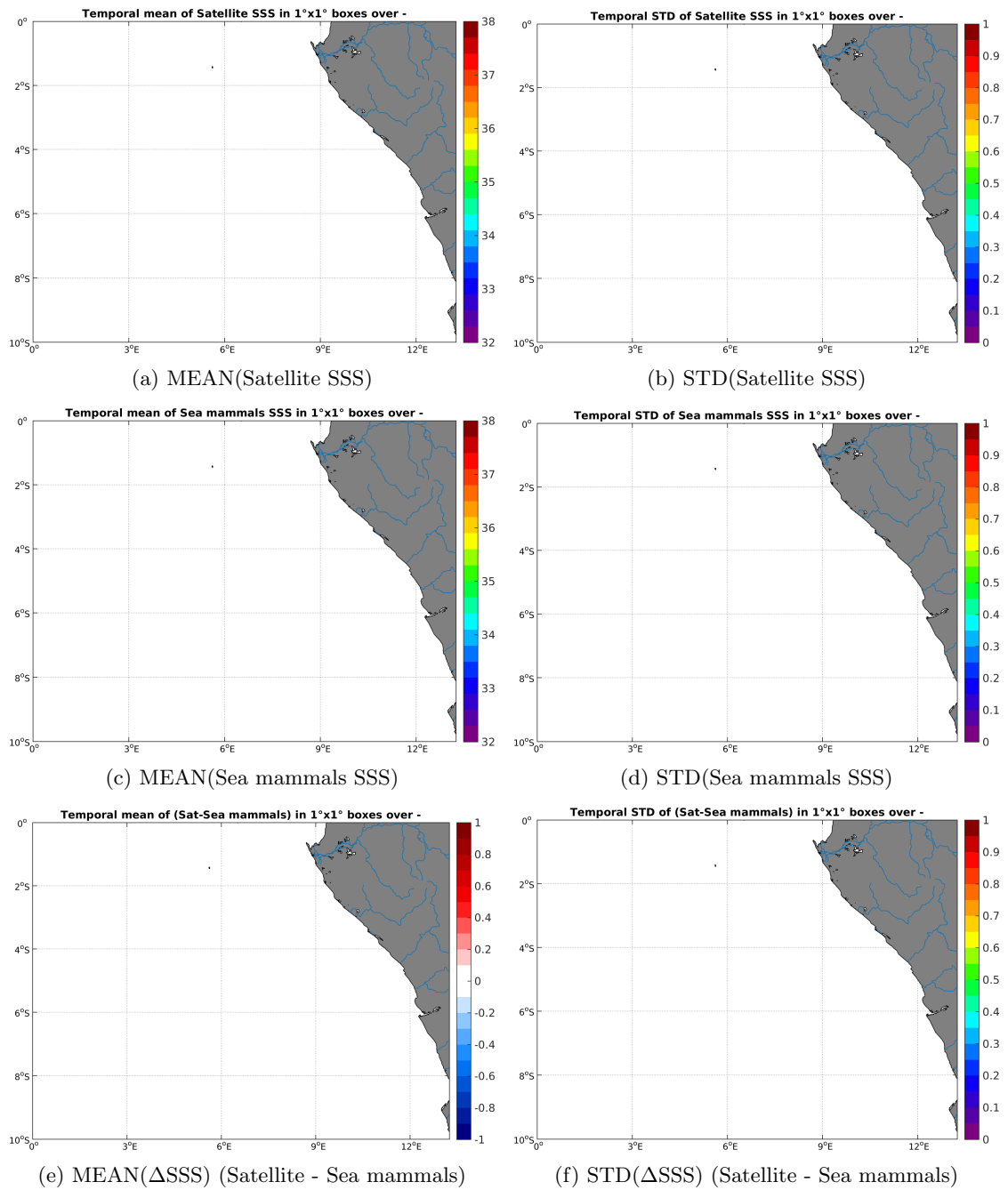
Figure 6: Temporal mean (left) and STD (right) of SSS from SMOS-L3-CATDS-CECOS-LOCEAN-V2-9DAYS-25KM (top), Sea mammals (middle), and of \Delta SSS (Satellite - Sea mammals). Only match-up pairs are used to generate these maps.
