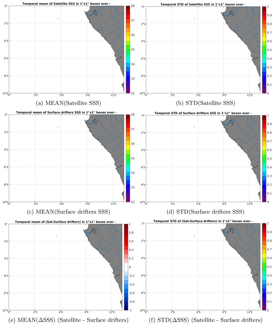
Figure 5: Temporal mean (left) and STD (right) of SSS from SMOS-L3-CATDS-CECOS-LOCEAN-V2-9DAYS-25KM (top), Surface drifters (middle), and of \Delta SSS (Satellite - Surface drifters). Only match-up pairs are used to generate these maps.
