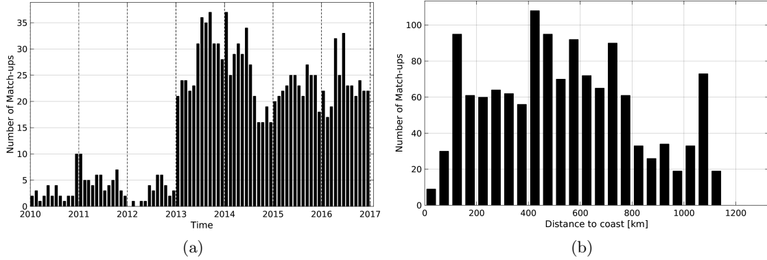
Figure 1: Number of match-ups between Argo and SMOS-L3-CATDS-CECOS-LOCEAN-V2-9DAYS-25KM SSS as a function of time (a) and as function of the distance to coast (b) over the Congo river plume Pi-MEP region and for the full satellite product period.
