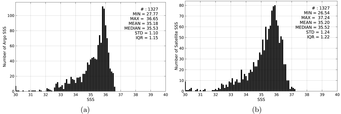
Figure 2: Histograms of SSS from Argo (a) and SMOS-L3-CATDS-CECOS-LOCEAN-V2-9DAYS-25KM (b) considering all match-up pairs per bins of 0.1 over the Congo river plume Pi-MEP region and for the full satellite product period.
