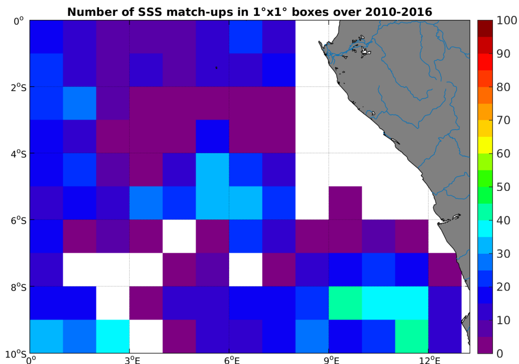
Figure 4: Number of SSS match-ups between Argo SSS and the SMOS-L3-CATDS-CECOS-LOCEAN-V2-9DAYS-25KM SSS product for the Congo river plume Pi-MEP region over 1^\circ \times 1^\circ boxes and for the full satellite product period.
