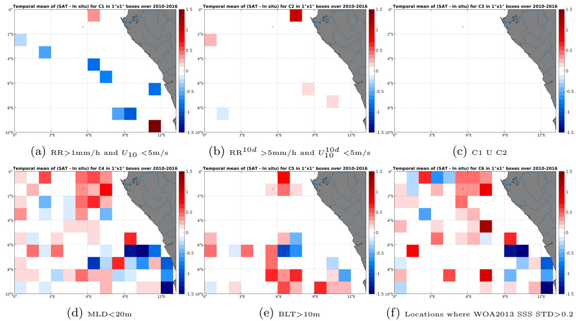
Figure 12: Temporal mean gridded over spatial boxes of size 1^\circ \times 1^\circ of \Delta SSS (SMOS-L3-CATDS-CECOS-LOCEAN-V2-9DAYS-25KM - Argo) for 6 different subdatasets corresponding to:RR >1 mm/h and U_{10} < 5 m/s (a), RR^{10d} > 5 mm/h and U_{10}^{10d} < 5 m/s (b), C1 U C2 (c),MLD <20 m (d),BLT >10 m (e),Locations where WOA2013 SSS STD >0.2 (f).
