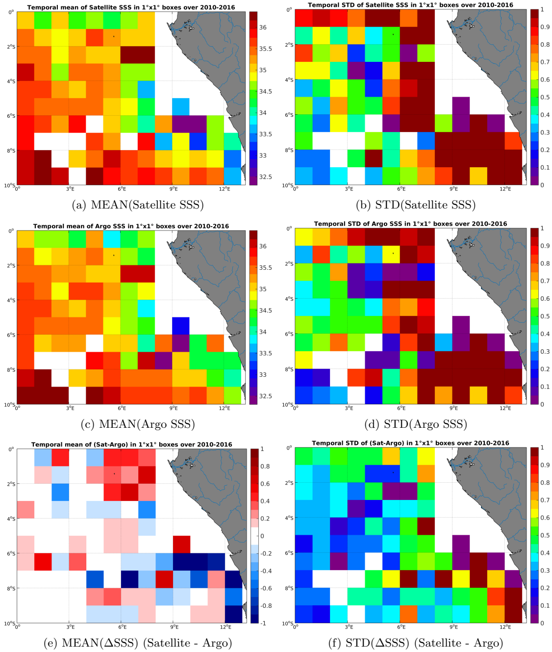
Figure 6: Temporal mean (left) and STD (right) of SSS from SMOS-L3-CATDS-CECOS-LOCEAN-V2-9DAYS-25KM (top), Argo (middle), and of \Delta SSS (Satellite - Argo). Only match-up pairs are used to generate these maps.
